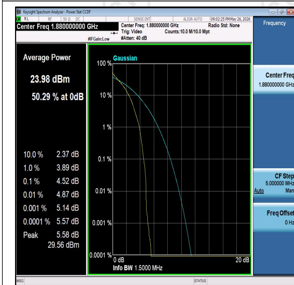
Band2-1.4MHz-QPSK-18900-PASS
