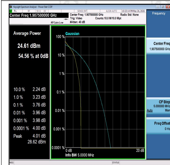
Band2-5MHz-QPSK-19175-PASS
