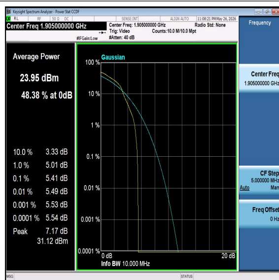
Band2-10MHz-16QAM-19150-PASS
