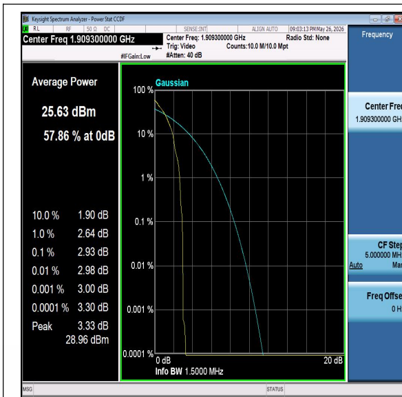
Band2-1.4MHz-QPSK-19193-PASS
