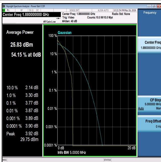
Band2-5MHz-QPSK-18900-PASS
