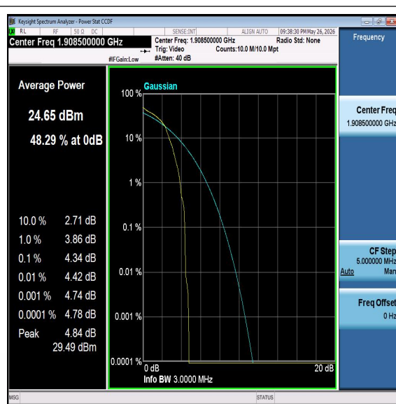
Band2-3MHz-16QAM-19185-PASS
