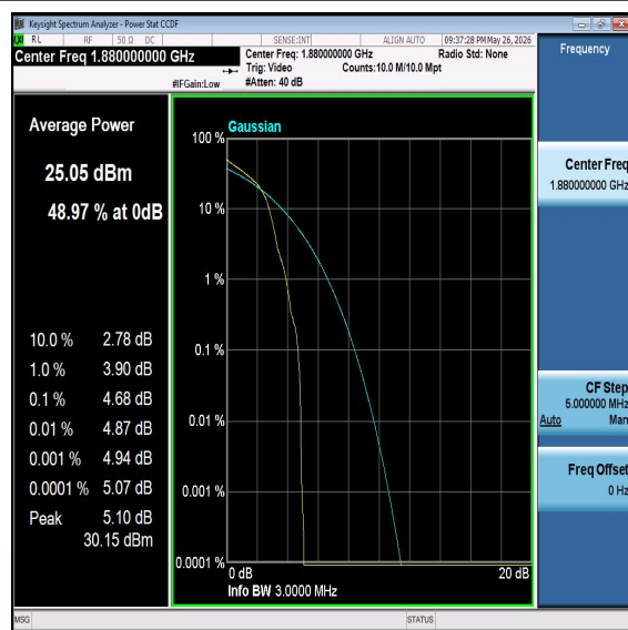
Band2-3MHz-16QAM-18900-PASS
