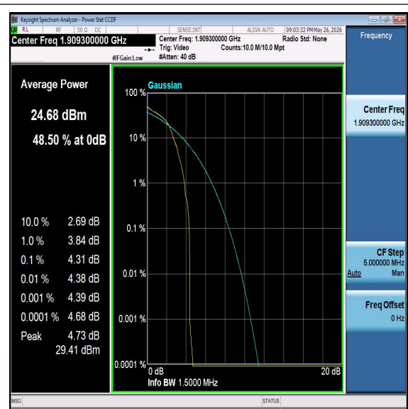
Band2-1.4MHz-16QAM-19193-PASS
