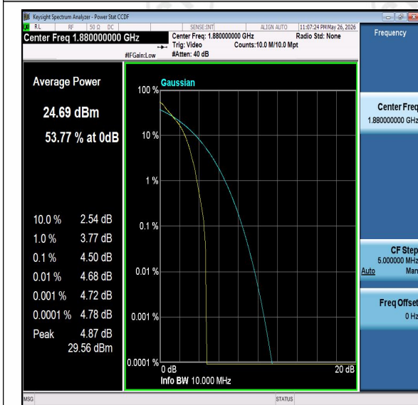
Band2-10MHz-QPSK-18900-PASS
