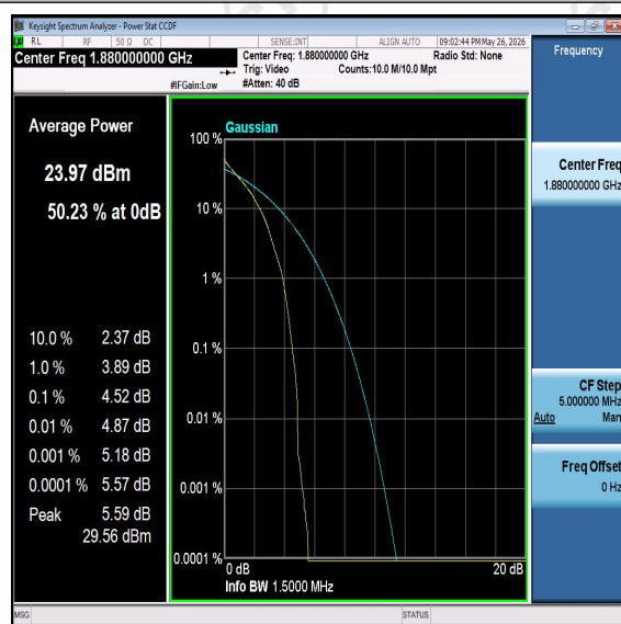
Band2-1.4MHz-16QAM-18900-PASS
