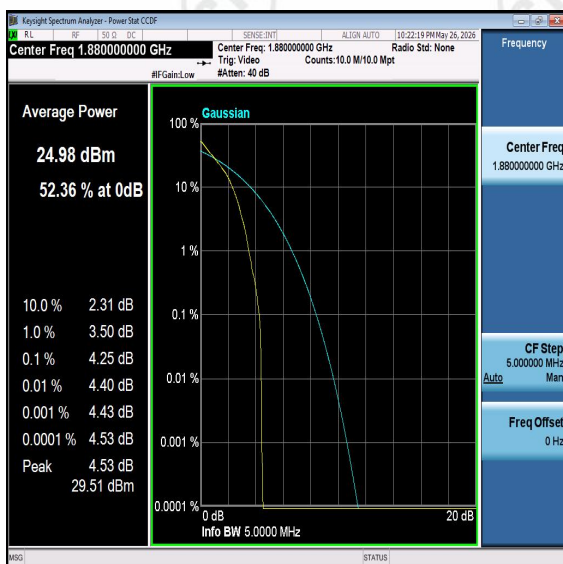
Band2-5MHz-QPSK-18900-PASS
