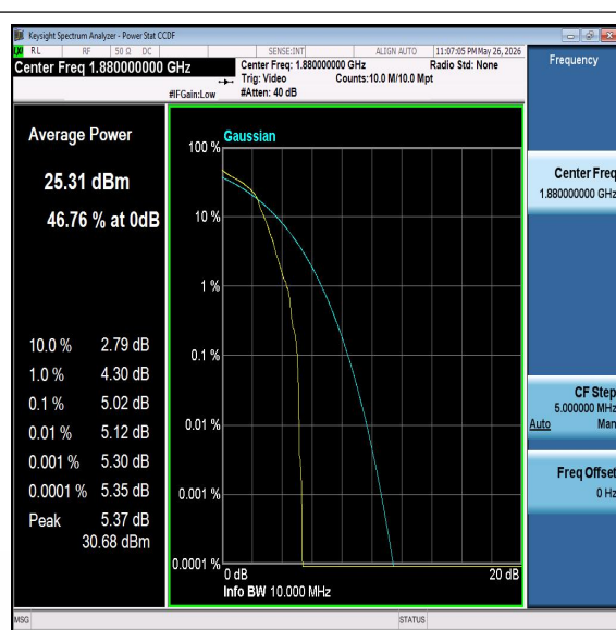
Band2-10MHz-16QAM-18900-PASS
