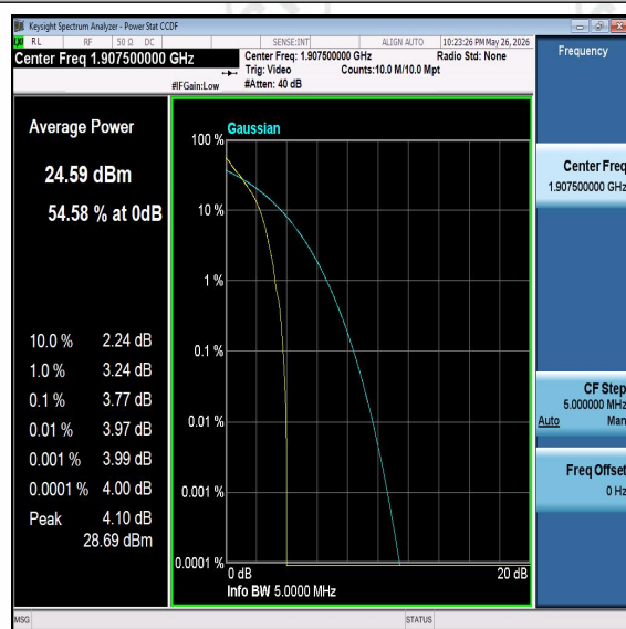
Band2-5MHz-16QAM-19175-PASS
