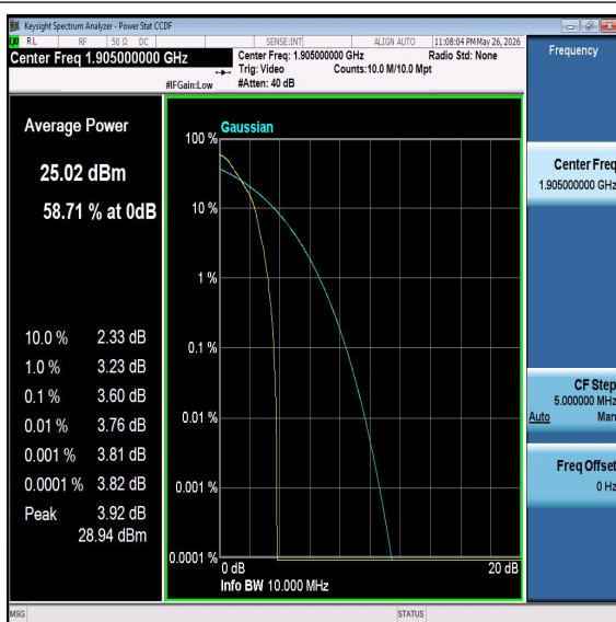
Band2-10MHz-QPSK-19150-PASS
