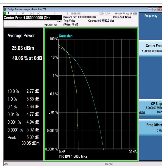
Band2-1.4MHz-16QAM-18900-PASS
