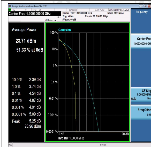
Band2-1.4MHz-QPSK-19193-PASS
