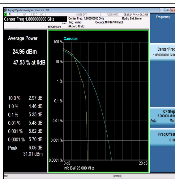
Band2-20MHz-16QAM-18700-PASS
