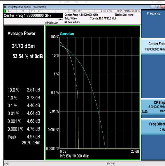
Band2-10MHz-16QAM-18900-PASS
