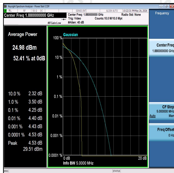
Band2-5MHz-16QAM-18900-PASS
