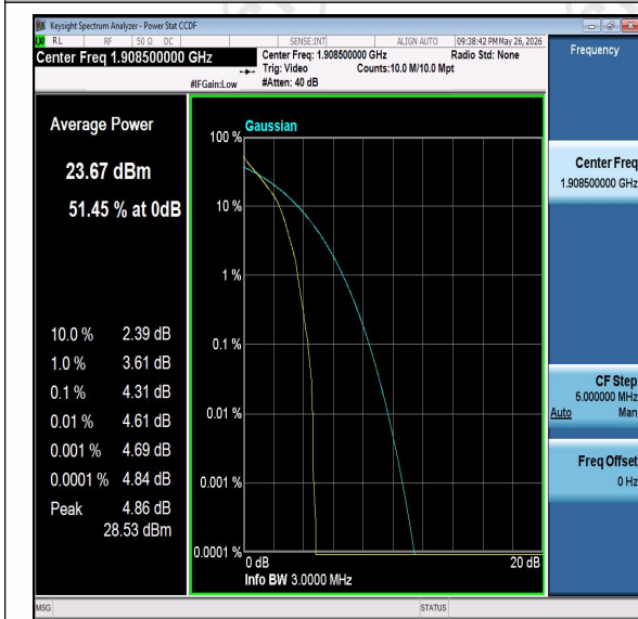
Band2-3MHz-QPSK-19185-PASS
