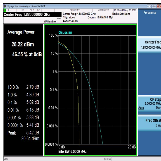
Band2-5MHz-16QAM-18900-PASS
