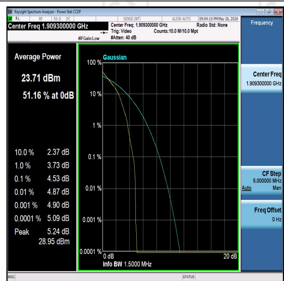
Band2-1.4MHz-16QAM-19193-PASS
