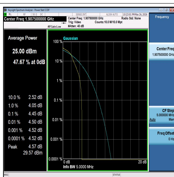
Band2-5MHz-16QAM-19175-PASS
