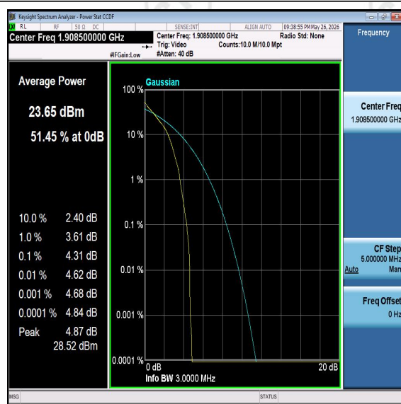
Band2-3MHz-16QAM-19185-PASS
