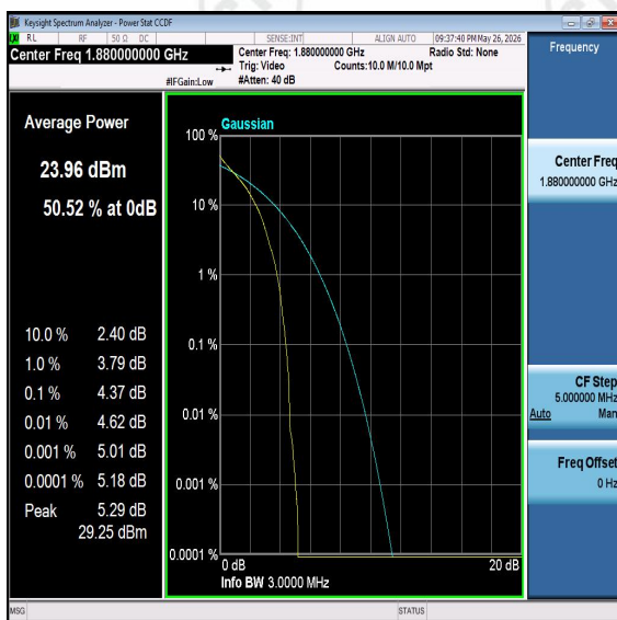
Band2-3MHz-QPSK-18900-PASS
