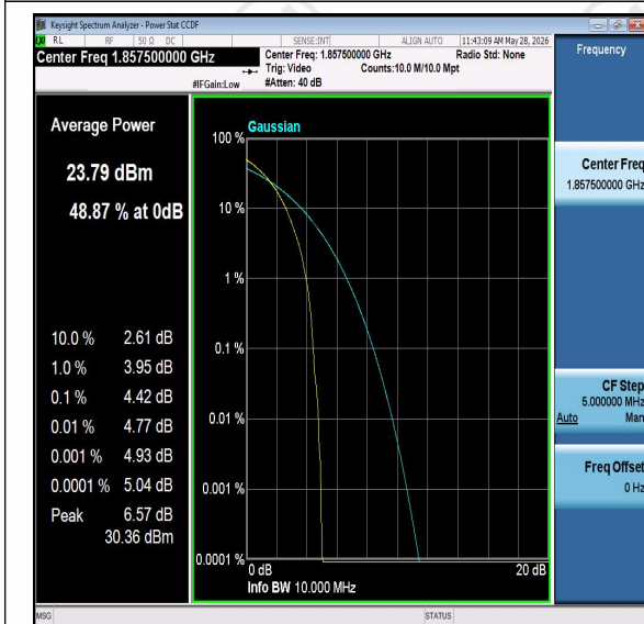
Band25-15MHz-QPSK-26115-PASS
