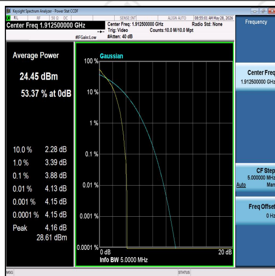
Band25-5MHz-16QAM-26665-PASS
