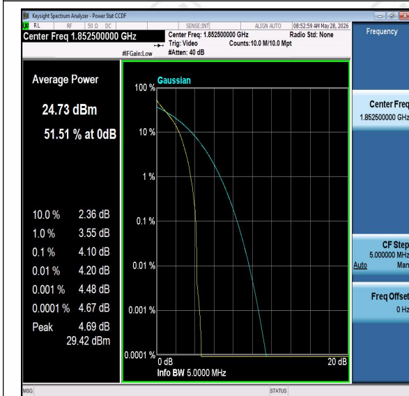
Band25-5MHz-QPSK-26065-PASS
