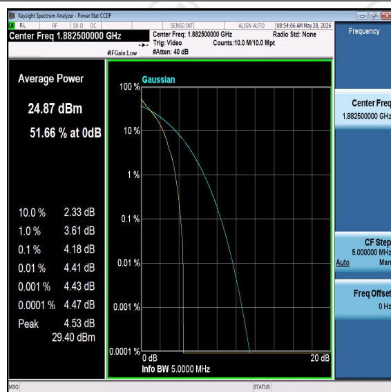
Band25-5MHz-16QAM-26365-PASS
