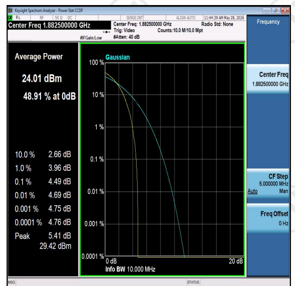
Band25-15MHz-16QAM-26365-PASS
