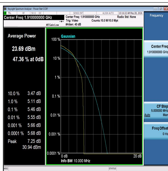
Band25-10MHz-16QAM-26640-PASS
