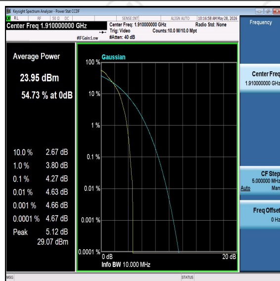
Band25-10MHz-16QAM-26640-PASS
