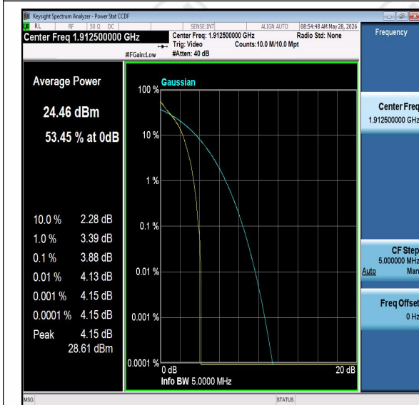
Band25-5MHz-QPSK-26665-PASS
