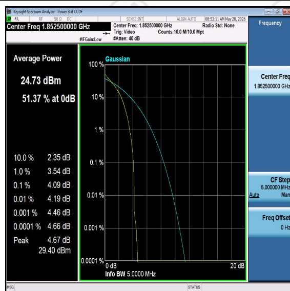
Band25-5MHz-16QAM-26065-PASS
