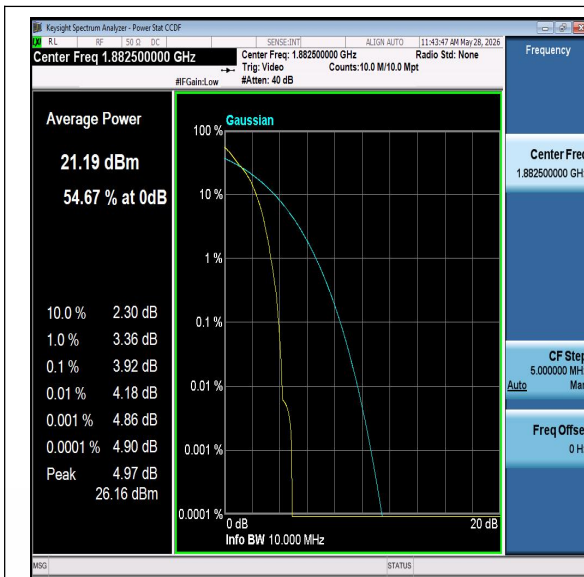
Band25-15MHz-QPSK-26365-PASS
