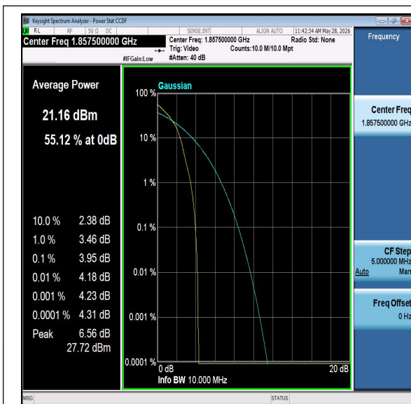
Band25-15MHz-QPSK-26115-PASS
