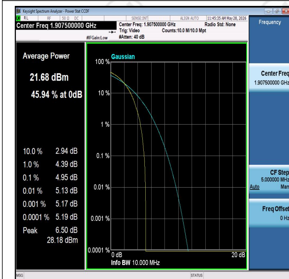
Band25-15MHz-QPSK-26615-PASS
