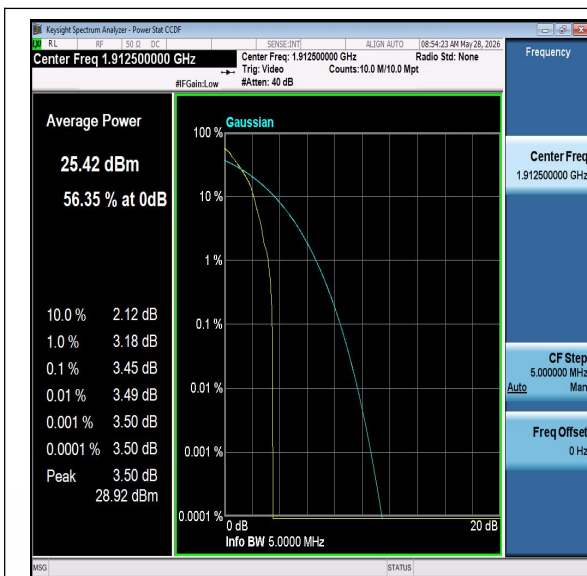
Band25-5MHz-QPSK-26665-PASS
