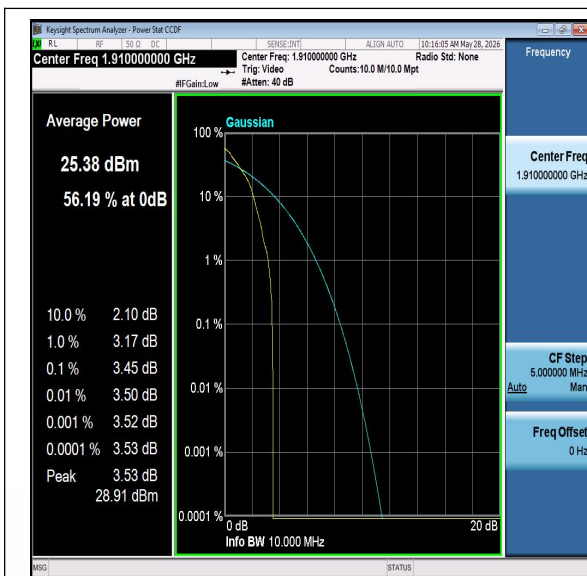
Band25-10MHz-QPSK-26640-PASS
