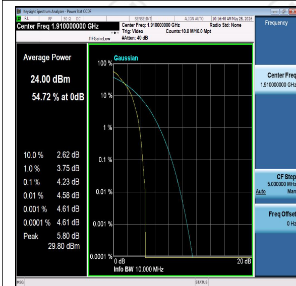
Band25-10MHz-QPSK-26640-PASS
