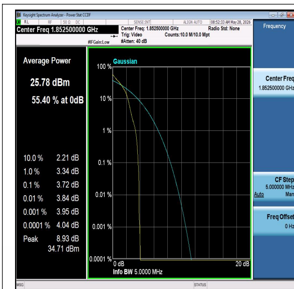
Band25-5MHz-QPSK-26065-PASS
