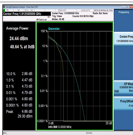
Band25-5MHz-16QAM-26665-PASS
