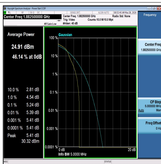
Band25-5MHz-16QAM-26365-PASS
