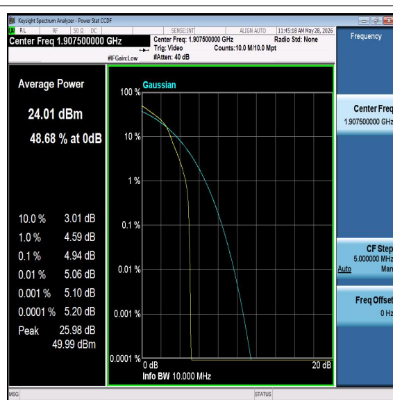
Band25-15MHz-16QAM-26615-PASS
