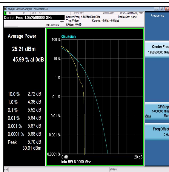
Band25-5MHz-16QAM-26065-PASS
