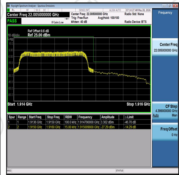
Band25-1.4MHz-QPSK-26683-PASS
