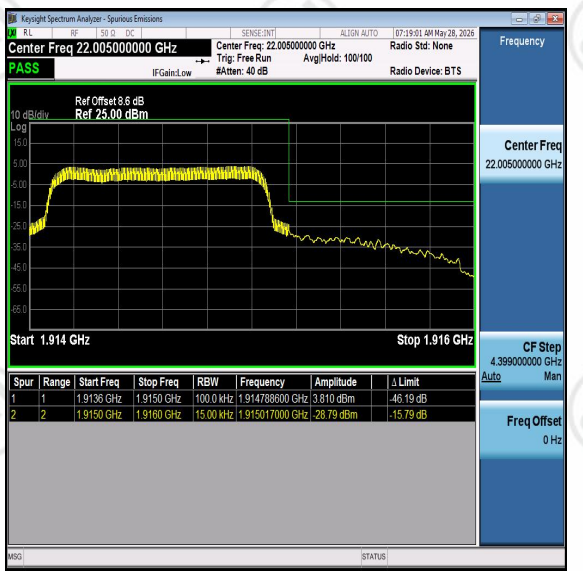
Band25-1.4MHz-16QAM-26683-PASS
