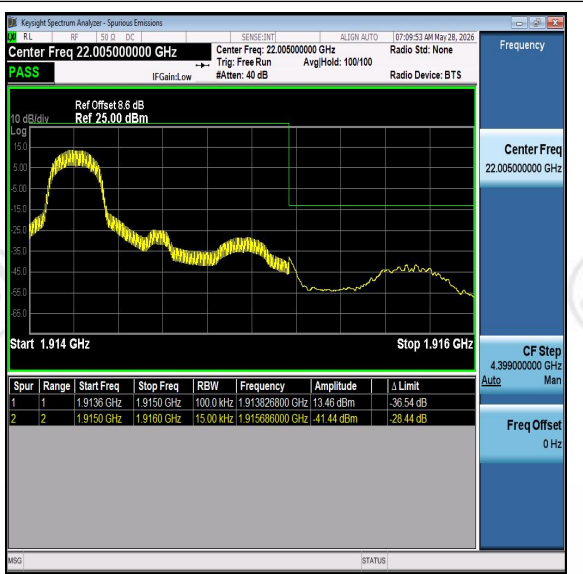
Band25-1.4MHz-16QAM-26683-PASS
