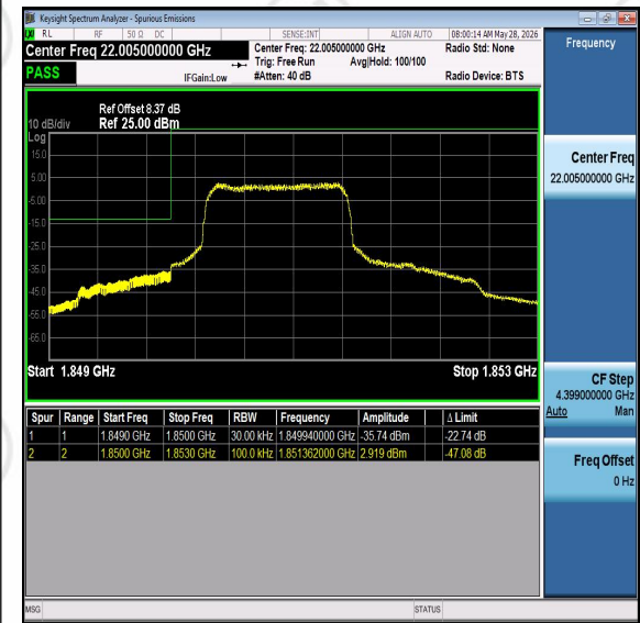
Band25-3MHz-QPSK-26055-PASS
