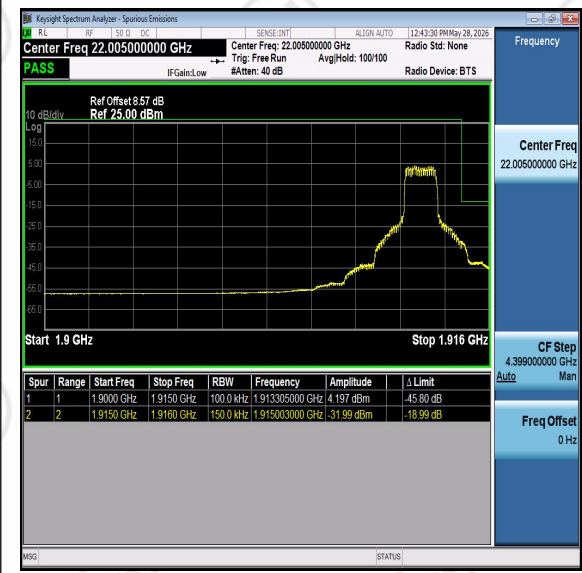
Band25-15MHz-QPSK-26615-PASS
