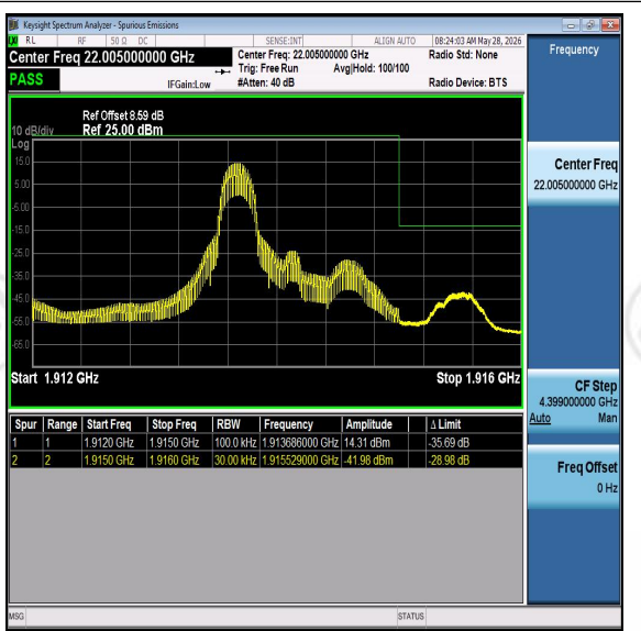
Band25-3MHz-16QAM-26675-PASS
