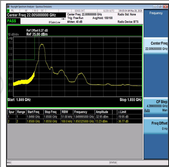
Band25-5MHz-QPSK-26065-PASS
