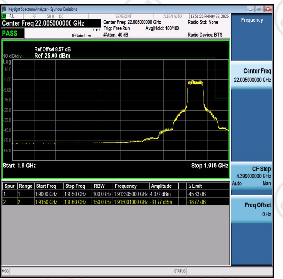
Band25-15MHz-16QAM-26615-PASS
