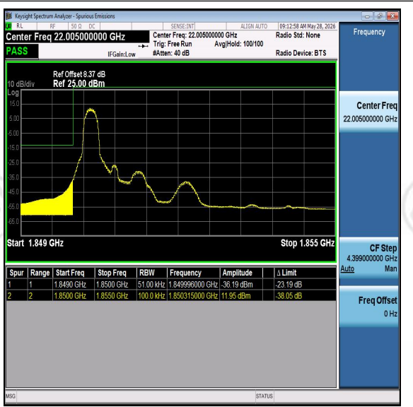
Band25-5MHz-16QAM-26065-PASS
