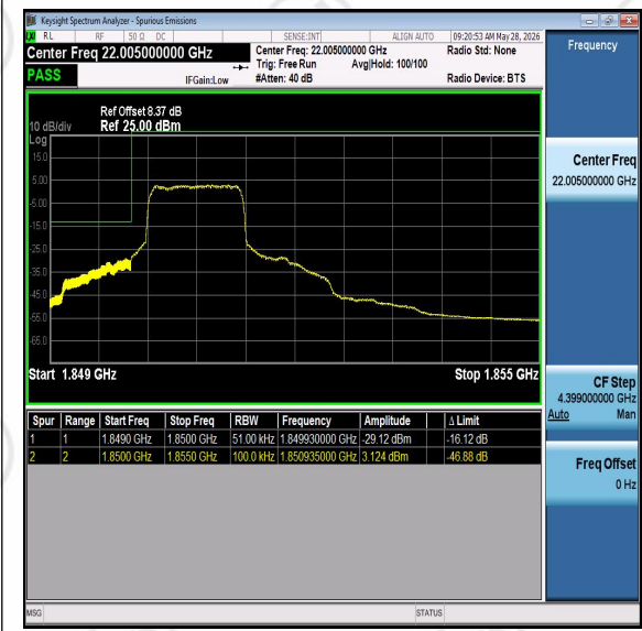
Band25-5MHz-QPSK-26065-PASS
