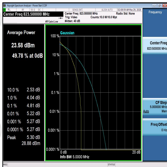
Band26-5MHz-QPSK-26785-PASS
