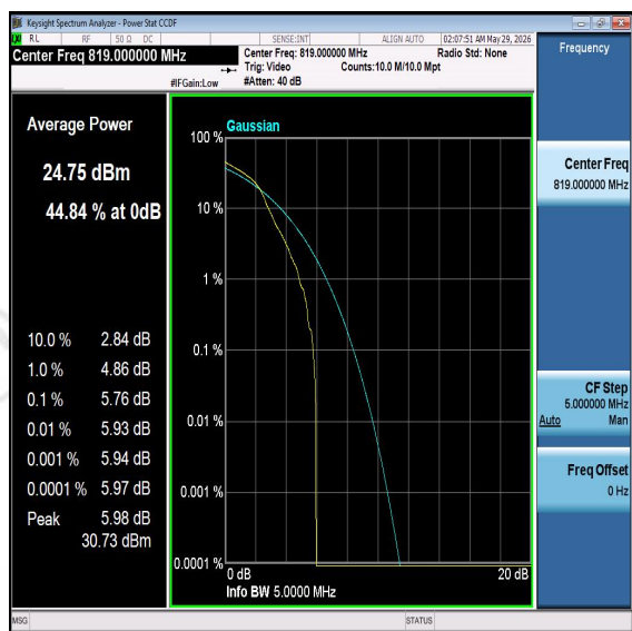
Band26-5MHz-16QAM-26740-PASS
