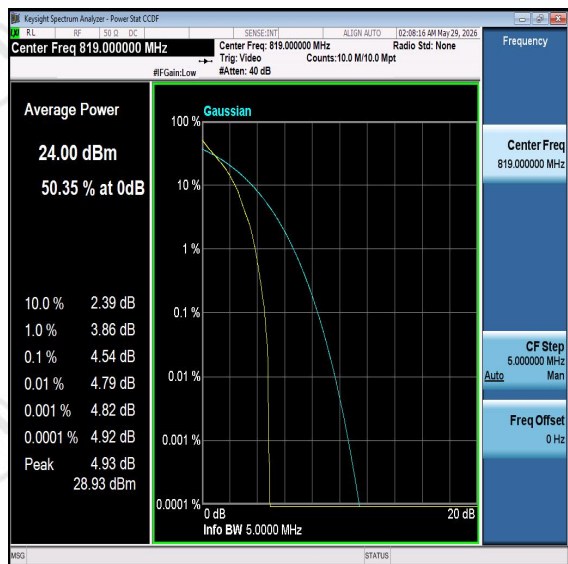
Band26-5MHz-16QAM-26740-PASS
