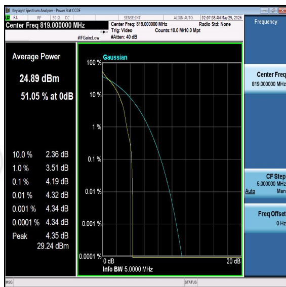
Band26-5MHz-QPSK-26740-PASS
