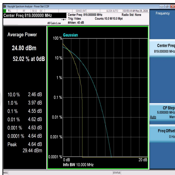
Band26-10MHz-QPSK-26740-PASS
