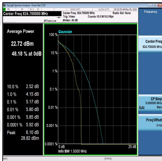
Band26-1.4MHz-QPSK-26797-PASS
