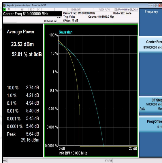
Band26-10MHz-16QAM-26740-PASS
