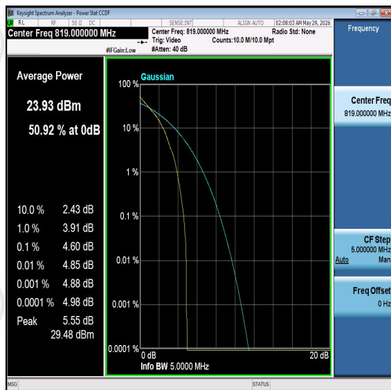
Band26-5MHz-QPSK-26740-PASS
