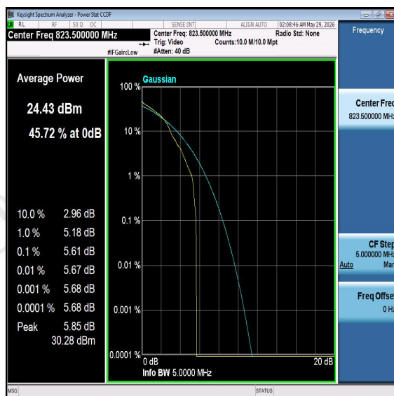
Band26-5MHz-16QAM-26785-PASS
