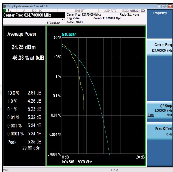
Band26-1.4MHz-16QAM-26797-PASS
