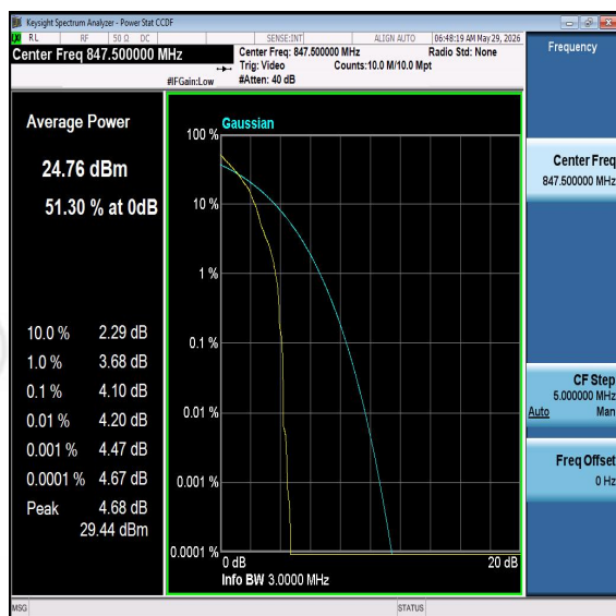
Band26-3MHz-QPSK-27025-PASS
