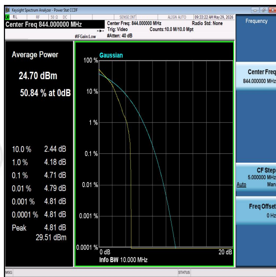
Band26-10MHz-QPSK-26990-PASS
