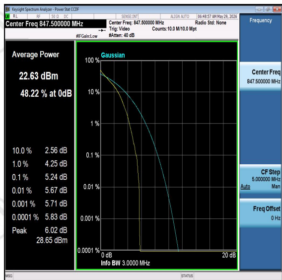
Band26-3MHz-16QAM-27025-PASS
