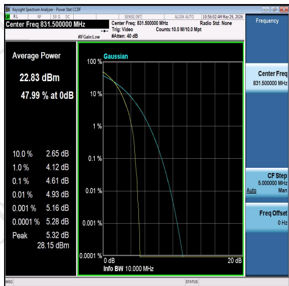
Band26-15MHz-16QAM-26865-PASS
