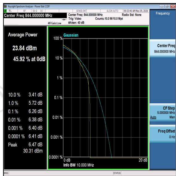
Band26-10MHz-16QAM-26990-PASS
