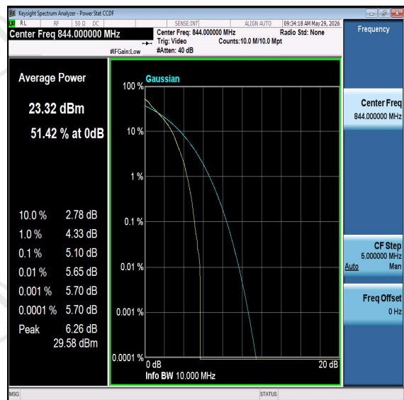
Band26-10MHz-16QAM-26990-PASS
