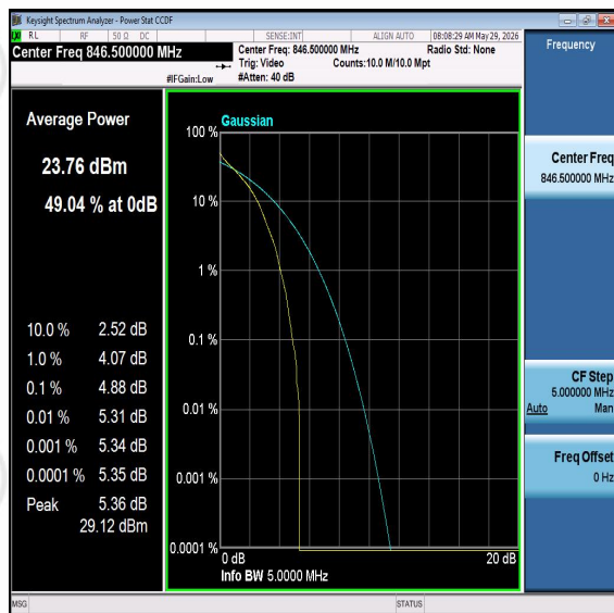
Band26-5MHz-QPSK-27015-PASS
