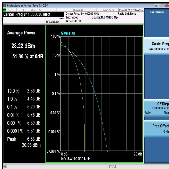
Band26-10MHz-QPSK-26990-PASS
