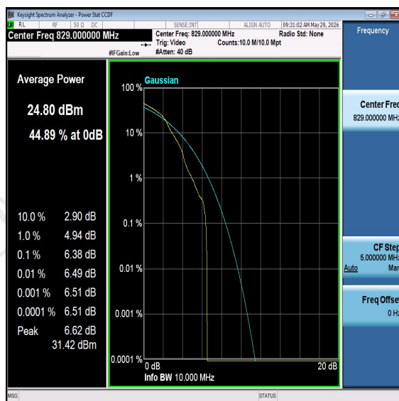
Band26-10MHz-16QAM-26840-PASS
