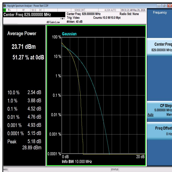
Band26-10MHz-QPSK-26840-PASS
