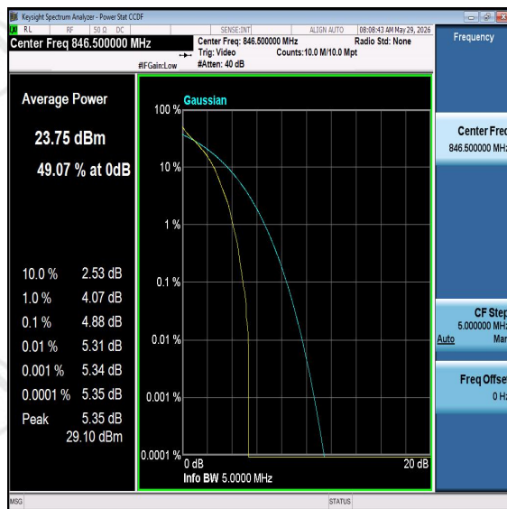
Band26-5MHz-16QAM-27015-PASS
