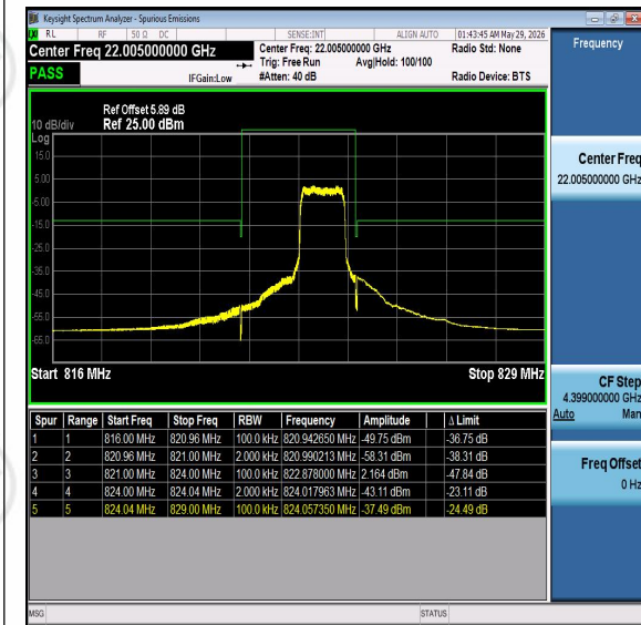
Band26-3MHz-QPSK-26775-PASS
