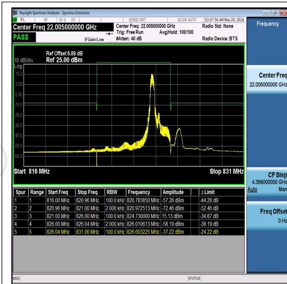
Band26-5MHz-QPSK-26785-PASS
