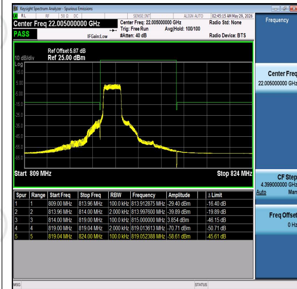
Band26-5MHz-QPSK-26715-PASS
