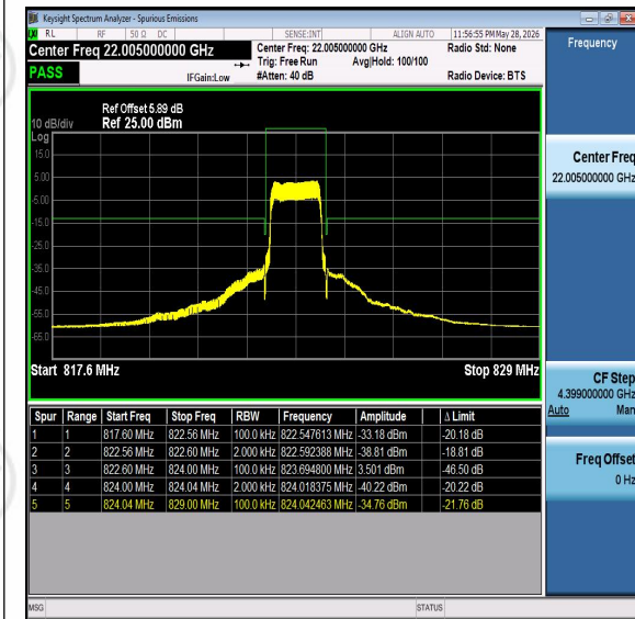
Band26-1.4MHz-QPSK-26783-PASS
