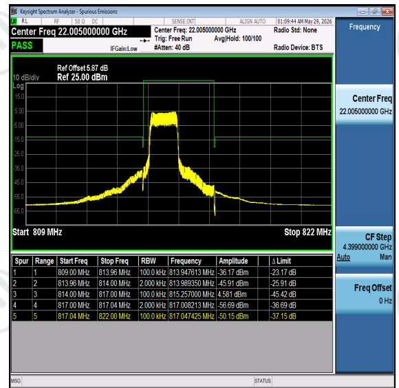
Band26-3MHz-16QAM-26705-PASS
