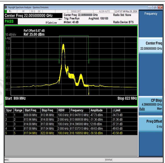
Band26-3MHz-16QAM-26705-PASS
