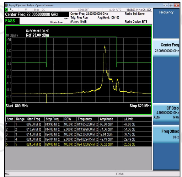
Band26-10MHz-16QAM-26740-PASS
