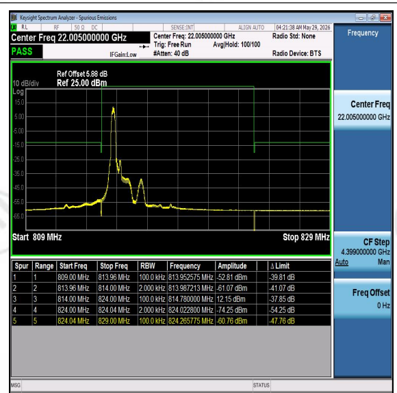
Band26-10MHz-16QAM-26740-PASS
