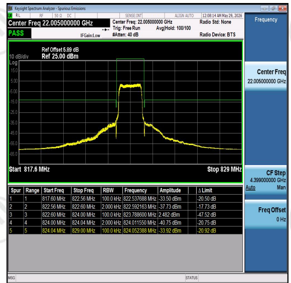
Band26-1.4MHz-16QAM-26783-PASS
