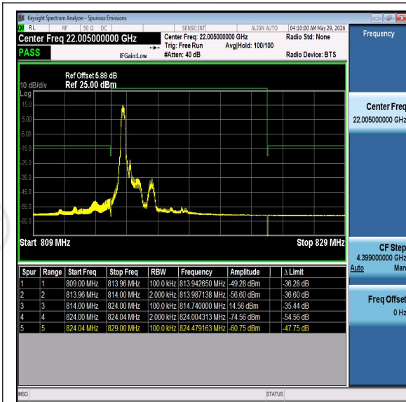
Band26-10MHz-QPSK-26740-PASS
