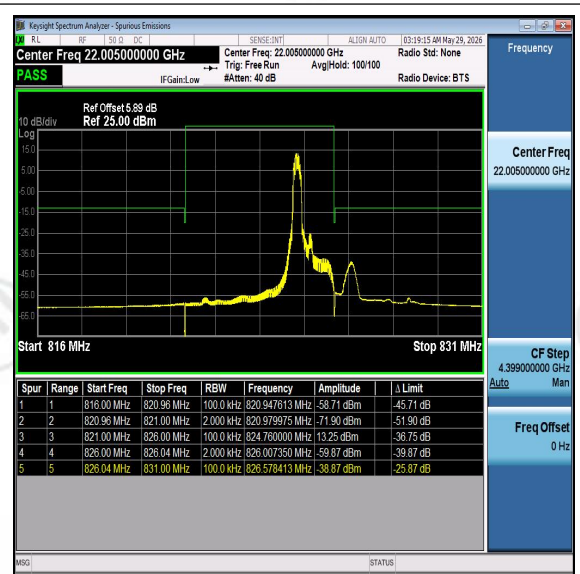
Band26-5MHz-16QAM-26785-PASS
