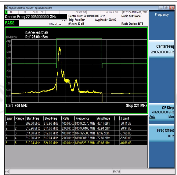
Band26-5MHz-16QAM-26715-PASS
