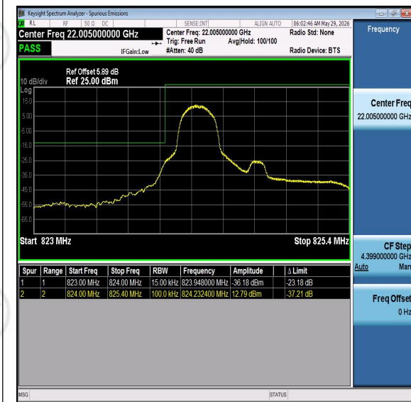
Band26-1.4MHz-QPSK-26797-PASS
