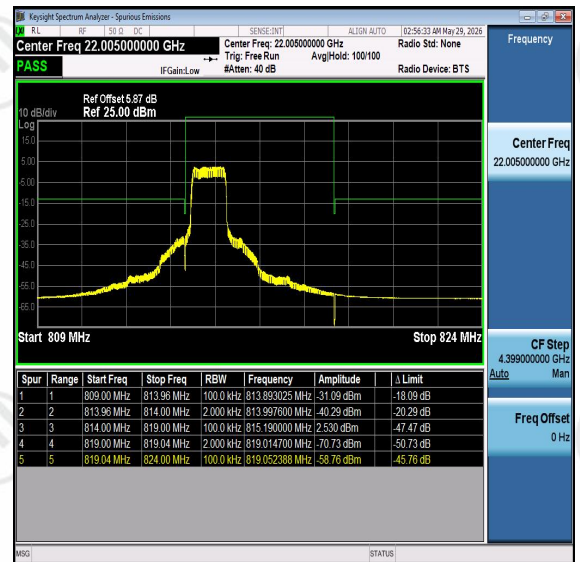
Band26-5MHz-16QAM-26715-PASS
