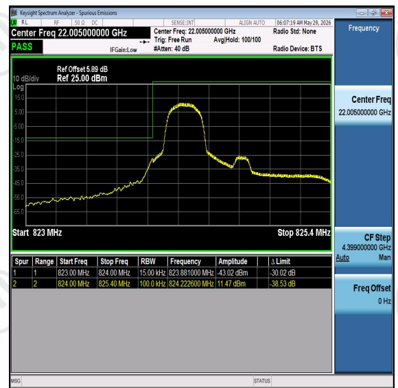
Band26-1.4MHz-16QAM-26797-PASS
