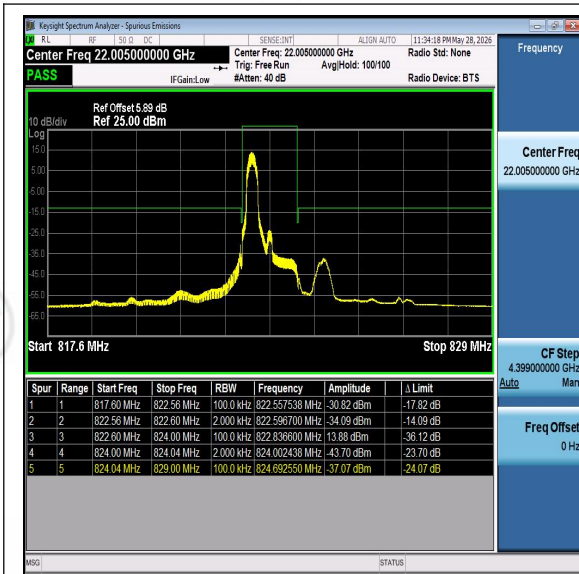
Band26-1.4MHz-QPSK-26783-PASS
