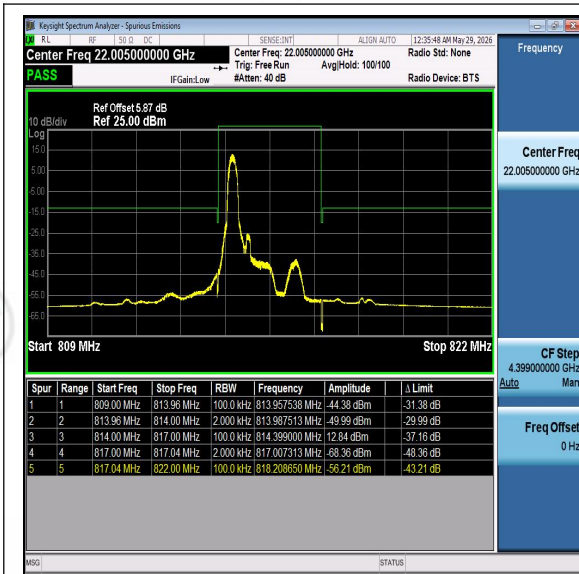
Band26-3MHz-QPSK-26705-PASS
