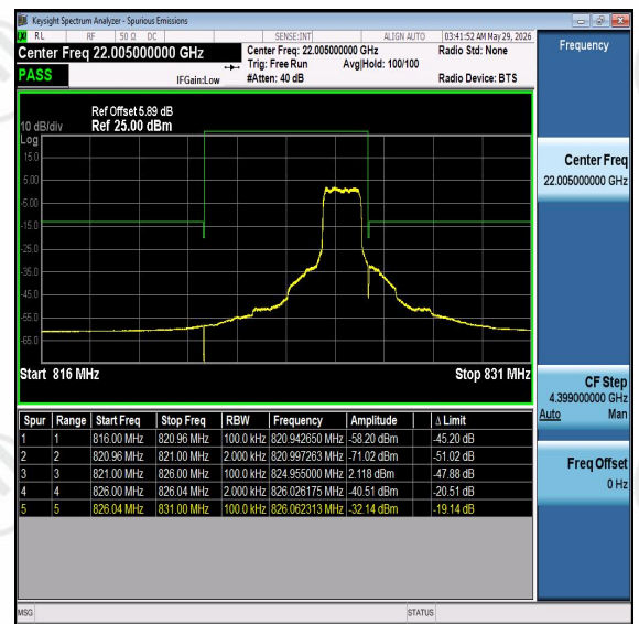
Band26-5MHz-16QAM-26785-PASS
