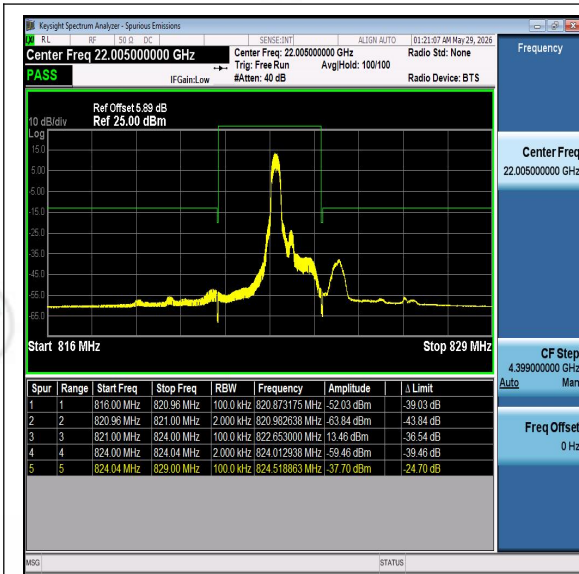
Band26-3MHz-QPSK-26775-PASS
