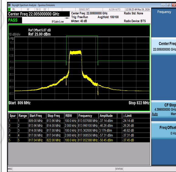
Band26-3MHz-QPSK-26705-PASS
