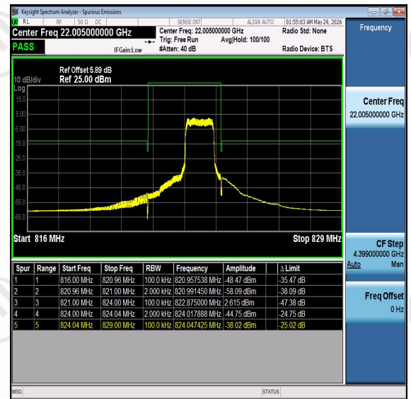
Band26-3MHz-16QAM-26775-PASS
