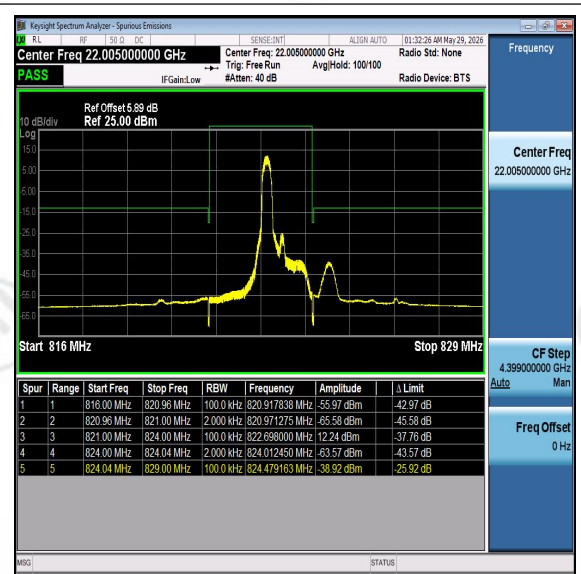
Band26-3MHz-16QAM-26775-PASS
