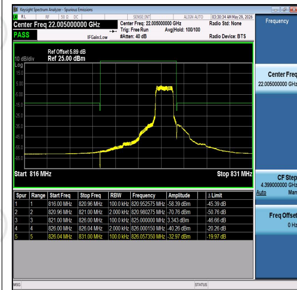
Band26-5MHz-QPSK-26785-PASS
