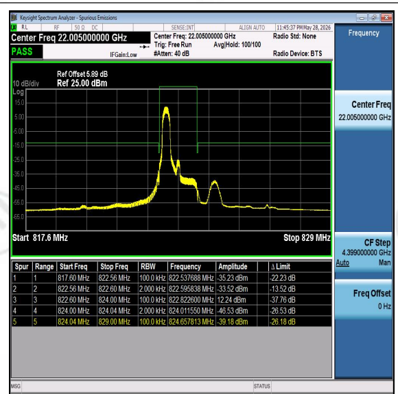
Band26-1.4MHz-16QAM-26783-PASS
