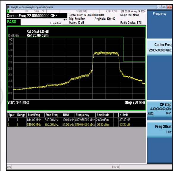
Band26-5MHz-QPSK-27015-PASS
