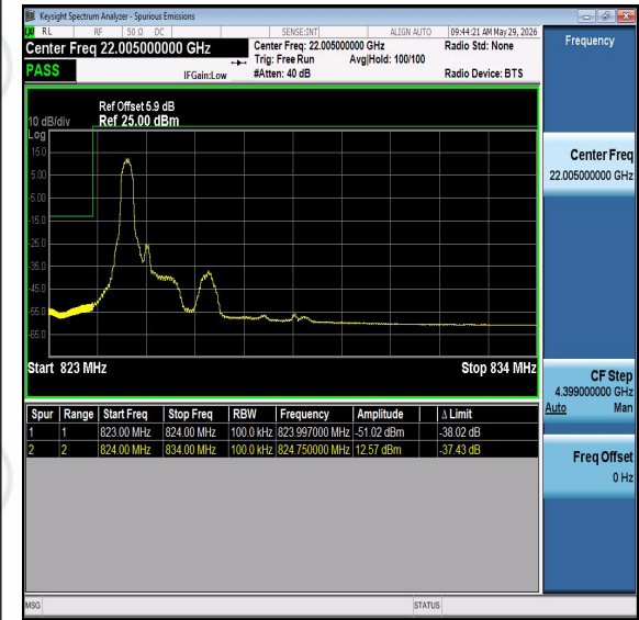
Band26-10MHz-QPSK-26840-PASS
