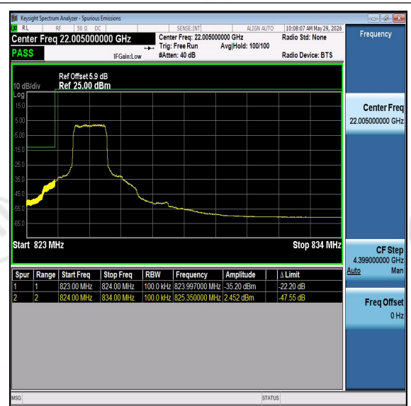
Band26-10MHz-16QAM-26840-PASS
