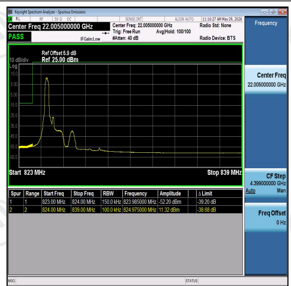
Band26-15MHz-16QAM-26865-PASS
