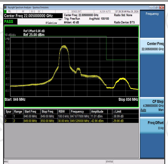
Band26-3MHz-16QAM-27025-PASS
