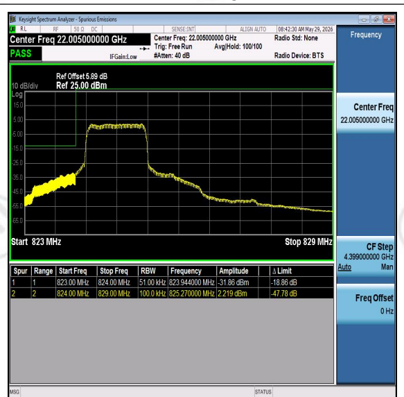
Band26-5MHz-16QAM-26815-PASS
