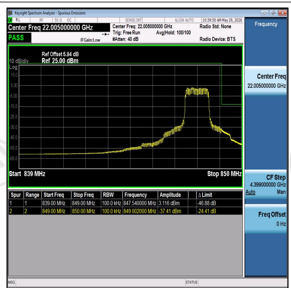
Band26-10MHz-16QAM-26990-PASS
