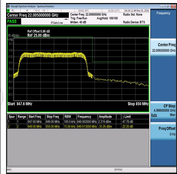
Band26-1.4MHz-QPSK-27033-PASS
