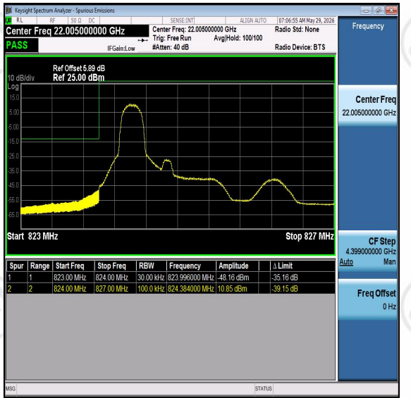
Band26-3MHz-16QAM-26805-PASS
