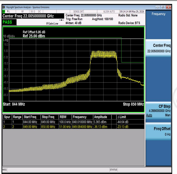
Band26-5MHz-16QAM-27015-PASS
