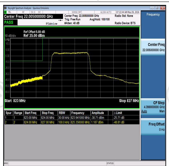
Band26-3MHz-16QAM-26805-PASS
