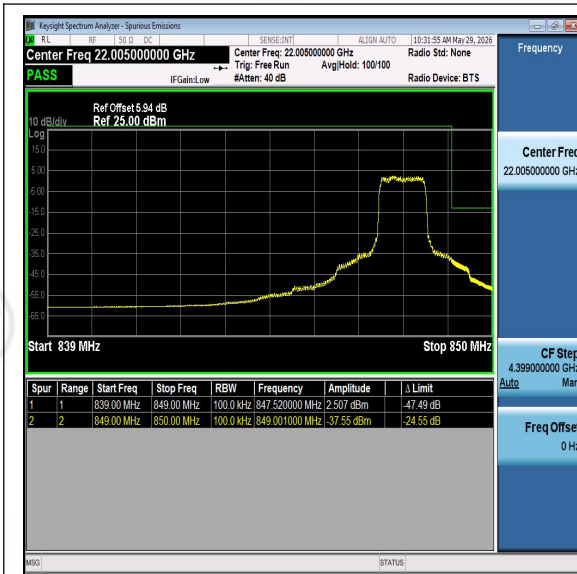
Band26-10MHz-QPSK-26990-PASS
