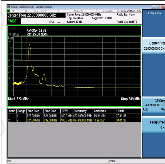
Band26-15MHz-QPSK-26865-PASS
