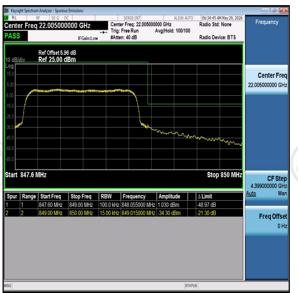
Band26-1.4MHz-16QAM-27033-PASS
