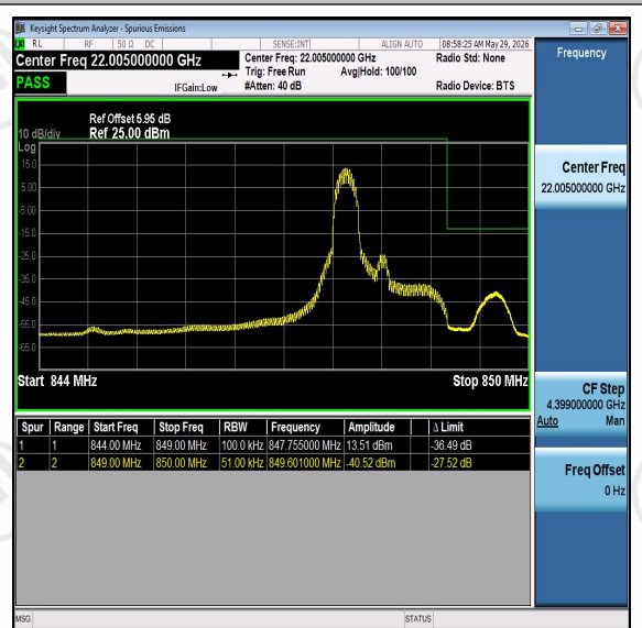
Band26-5MHz-16QAM-27015-PASS
