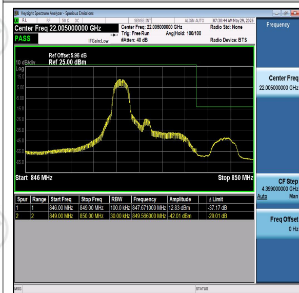
Band26-3MHz-QPSK-27025-PASS
