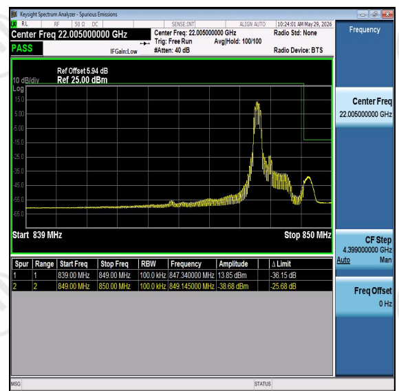
Band26-10MHz-16QAM-26990-PASS
