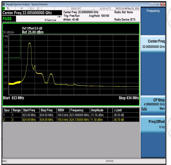
Band26-10MHz-16QAM-26840-PASS
