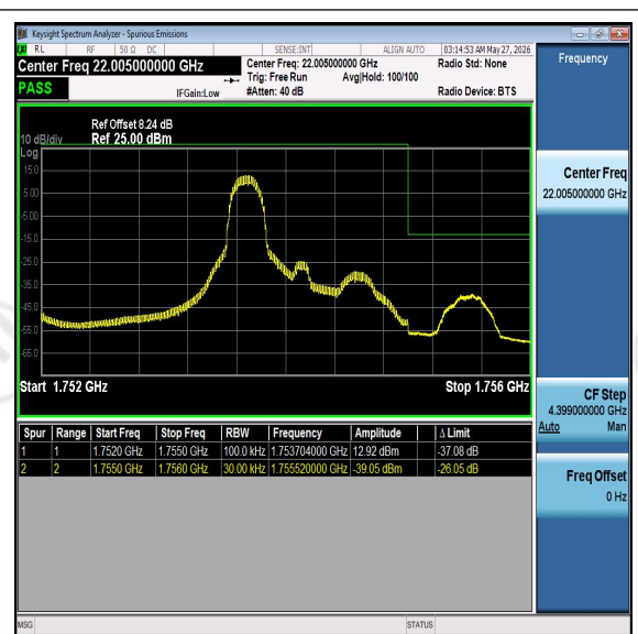
Band4-3MHz-16QAM-20385-PASS
