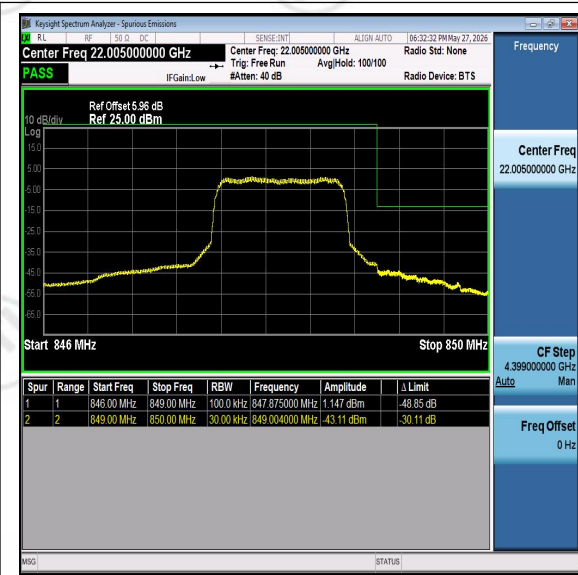
Band5-3MHz-16QAM-20635-PASS
