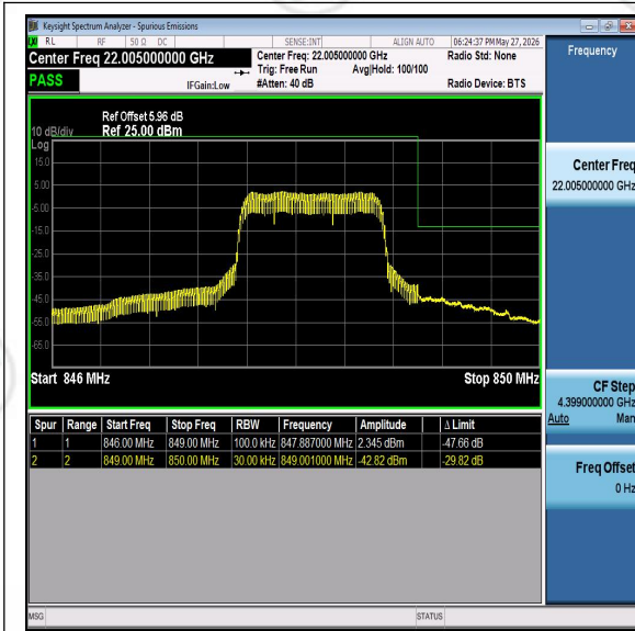
Band5-3MHz-QPSK-20635-PASS
