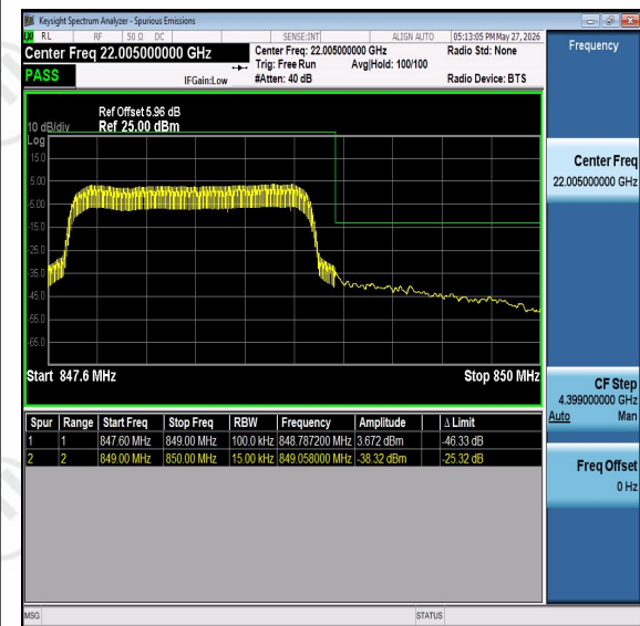
Band5-1.4MHz-16QAM-20643-PASS
