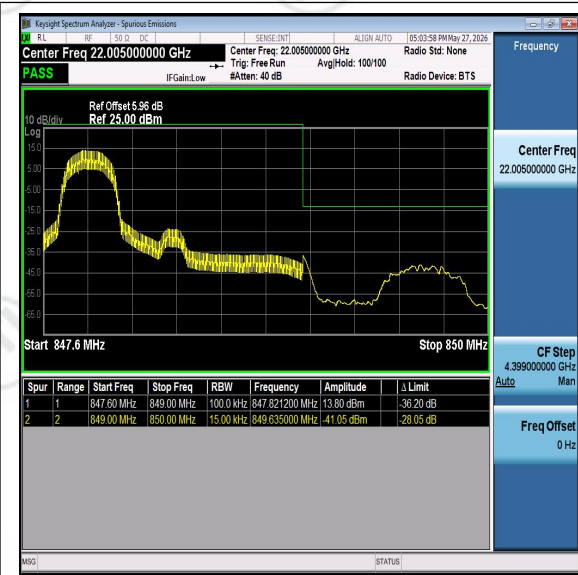
Band5-1.4MHz-16QAM-20643-PASS
