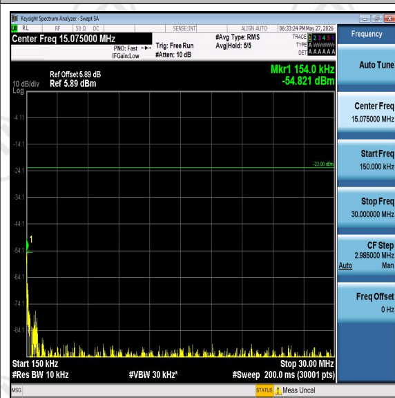
Band5-3MHz-QPSK-20415-30-1000-PASS
