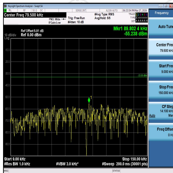
Band5-3MHz-QPSK-20525-0.009-0.15-PASS
