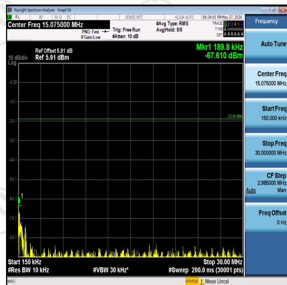
Band5-3MHz-QPSK-20525-0.15-30-PASS
