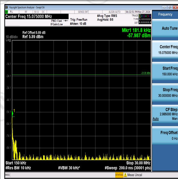
Band5-3MHz-QPSK-20415-0.15-30-PASS
