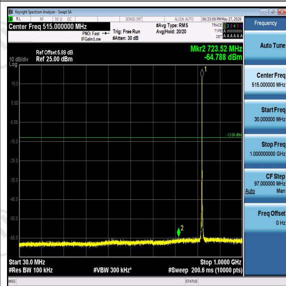
Band5-3MHz-QPSK-20415-30-1000-PASS
