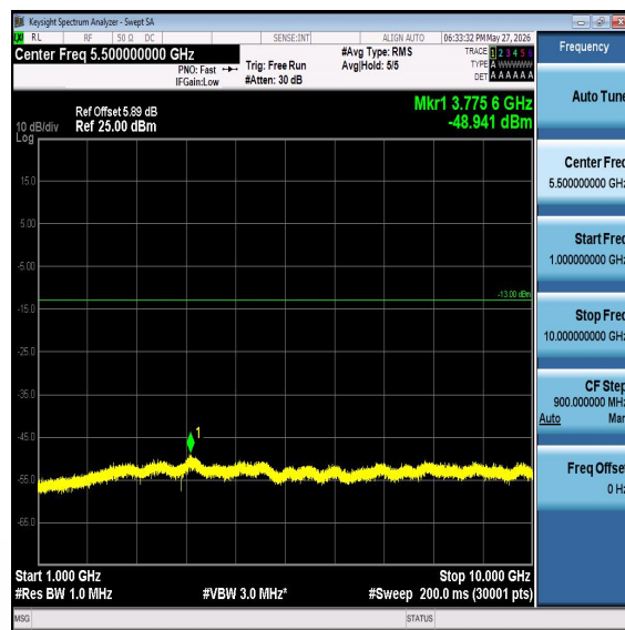
Band5-3MHz-16QAM-20415-1000-10000-PASS
