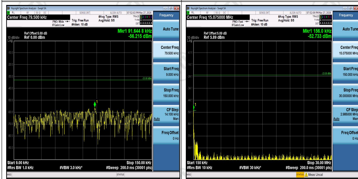
Band5-3MHz-16QAM-20635-1000-10000-PASS
