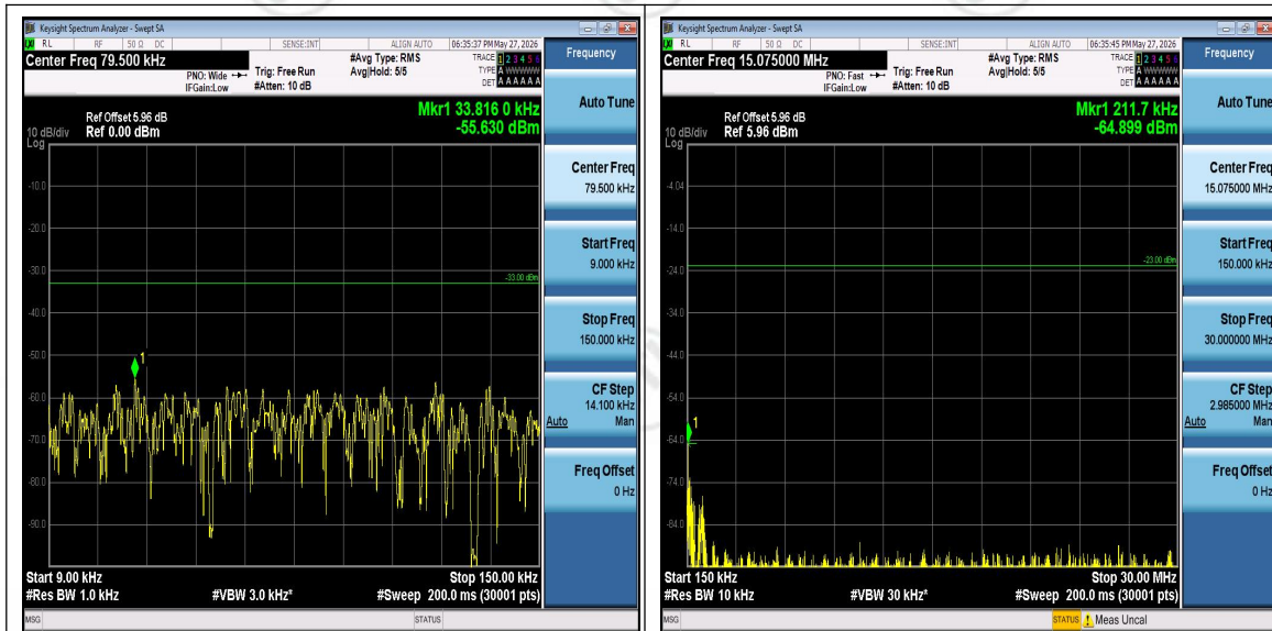
Band5-3MHz-16QAM-20635-0.009-0.15-PASS
