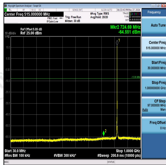
Band5-3MHz-16QAM-20415-30-10000-PASS
