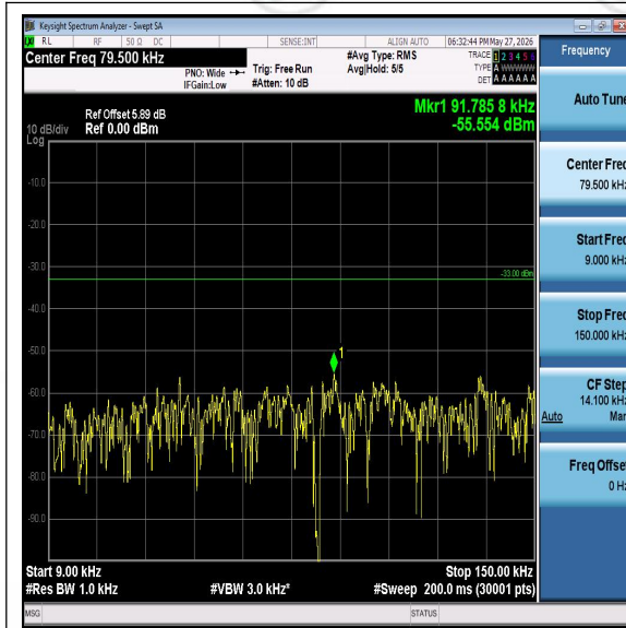
Band5-3MHz-QPSK-20415-0.009-0.15-PASS
