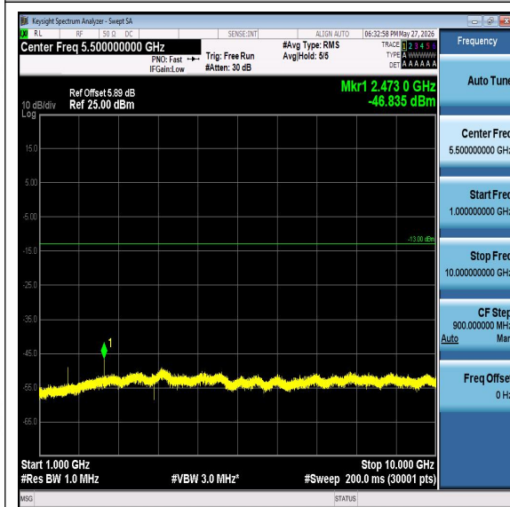
Band5-3MHz-QPSK-20415-1000-10000-PASS
