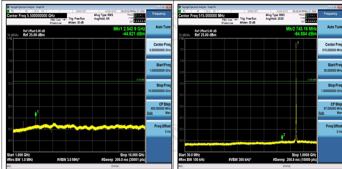
Band5-3MHz-16QAM-20635-1000-10000-PASS
