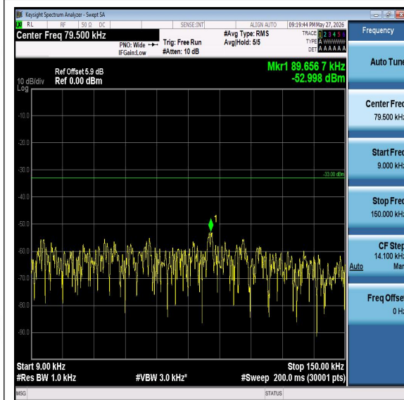
Band5-10MHz-16QAM-20450-0.009-0.15-PASS
