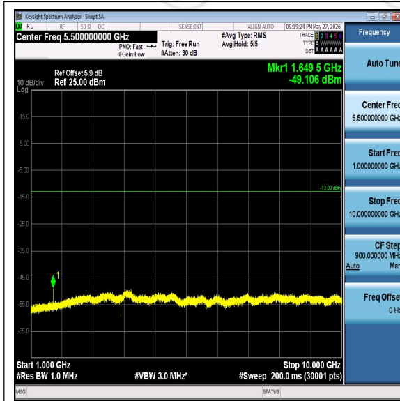
Band5-10MHz-QPSK-20450-1000-10000-PASS
