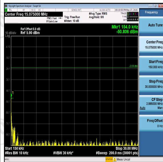
Band5-10MHz-16QAM-20450-0.15-30-PASS
