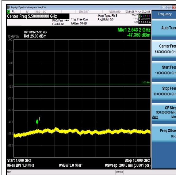
Band5-5MHz-QPSK-20625-1000-10000-PASS
