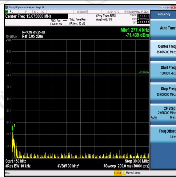
Band5-5MHz-QPSK-20625-0.15-30-PASS
