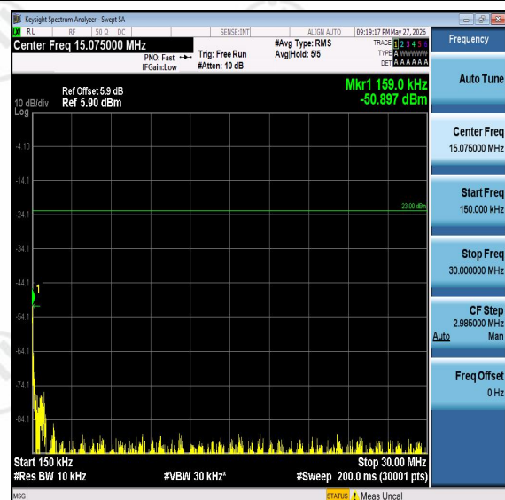
Band5-10MHz-QPSK-20450-0.15-30-PASS
