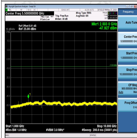
Band5-5MHz-QPSK-20525-0.009-0.15-PASS
