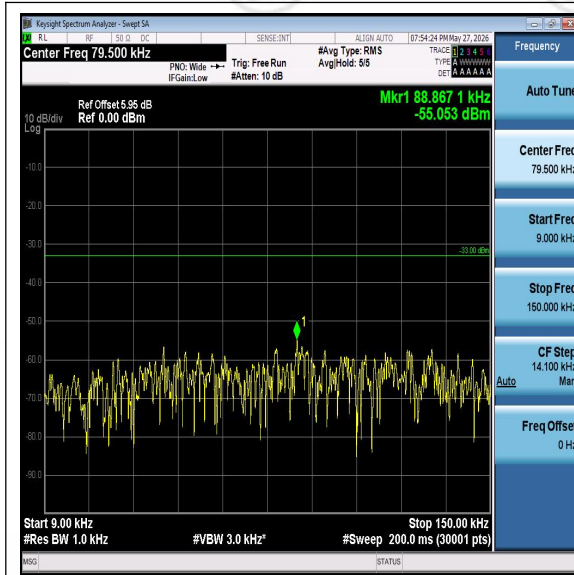
Band5-5MHz-QPSK-20625-0.009-0.15-PASS
