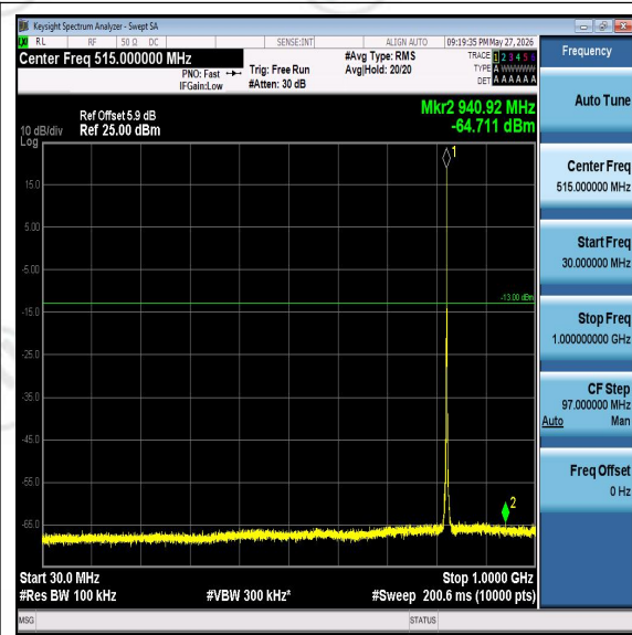
Band5-10MHz-QPSK-20450-30-1000-PASS
