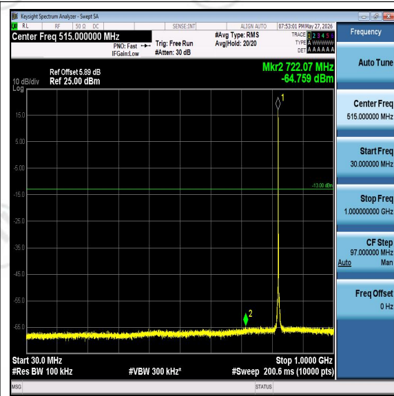
Band5-5MHz-16QAM-20425-30-1000-PASS
