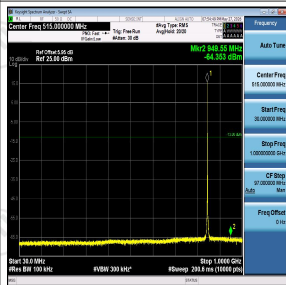
Band5-5MHz-QPSK-20625-30-1000-PASS
