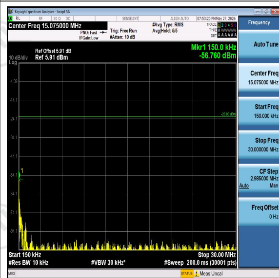
Band5-5MHz-QPSK-20525-0.15-30-PASS
