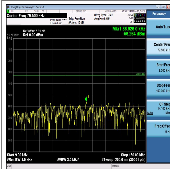
Band5-5MHz-QPSK-20525-0.009-0.15-PASS
