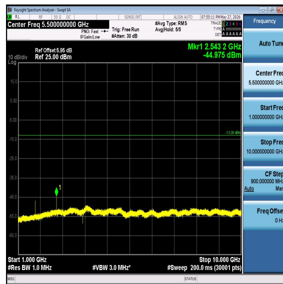
Band5-5MHz-16QAM-20625-1000-10000-PASS
