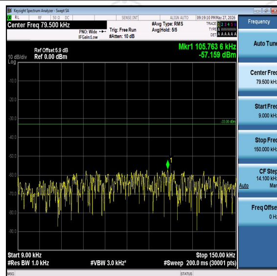
Band5-10MHz-QPSK-20450-0.009-0.15-PASS
