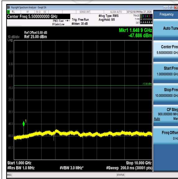
Band5-5MHz-16QAM-20425-1000-10000-PASS
