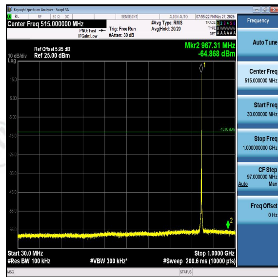
Band5-5MHz-16QAM-20625-30-1000-PASS
