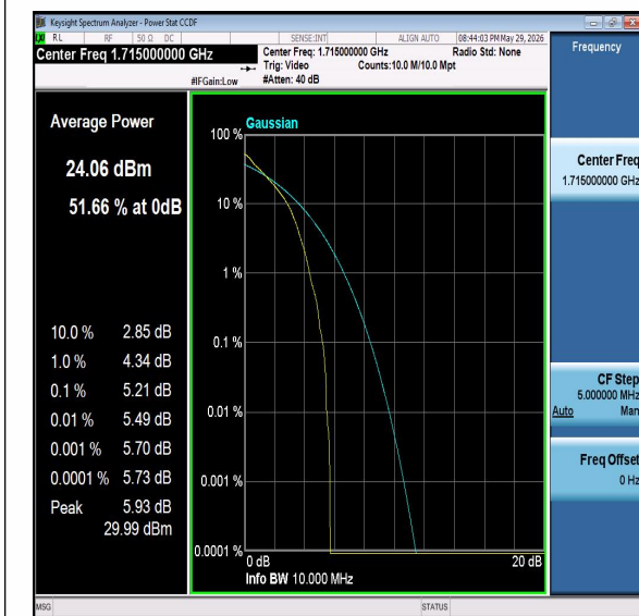
Band66-10MHz-QPSK-132022-PASS
