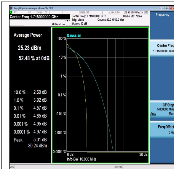
Band66-10MHz-QPSK-132022-PASS
