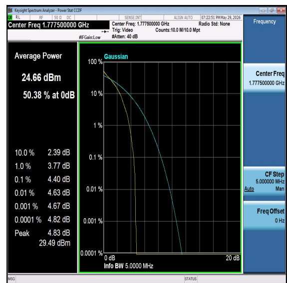
Band66-5MHz-16QAM-132647-PASS
