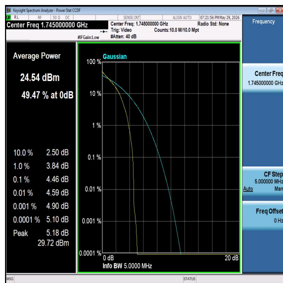
Band66-5MHz-16QAM-132322-PASS
