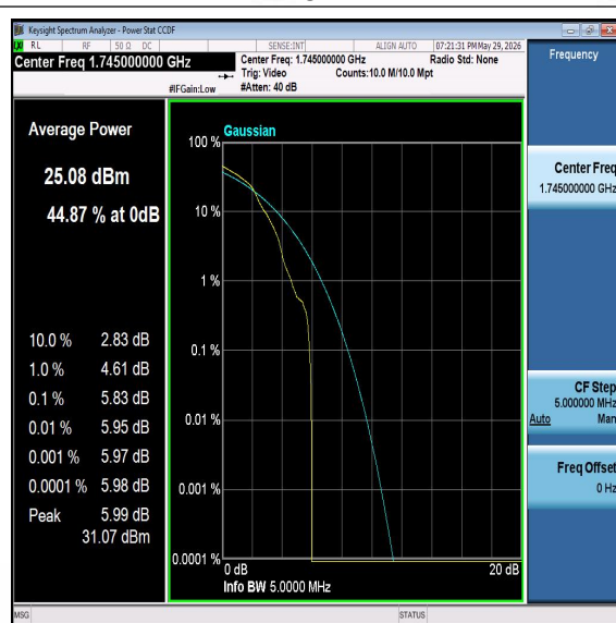
Band66-5MHz-16QAM-132322-PASS
