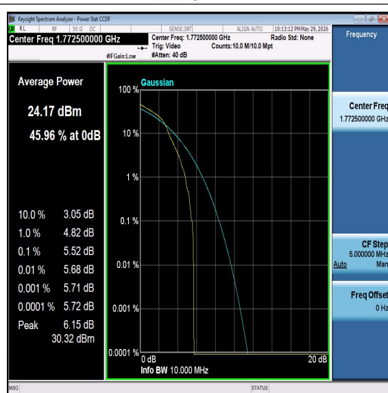
Band66-15MHz-16QAM-132597-PASS
