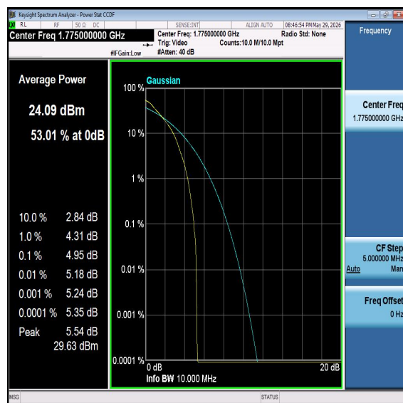
Band66-10MHz-16QAM-132622-PASS
