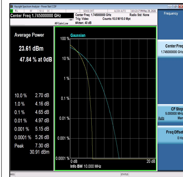
Band66-15MHz-QPSK-132322-PASS
