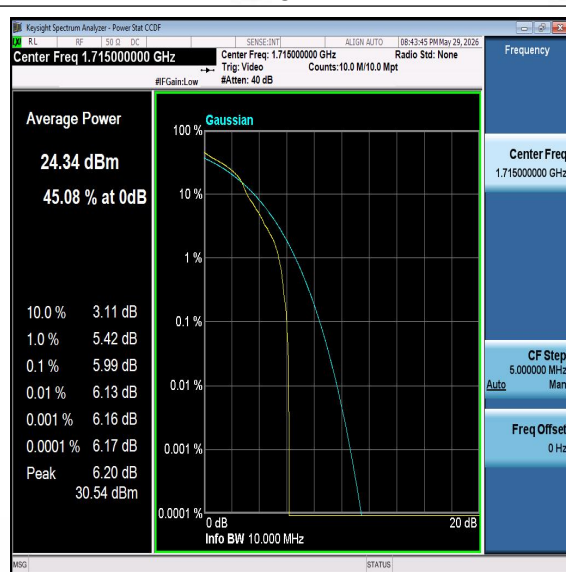
Band66-10MHz-16QAM-132022-PASS
