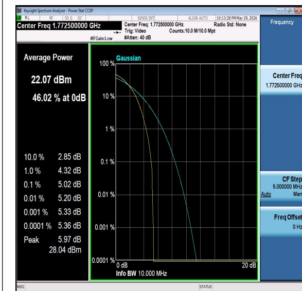
Band66-15MHz-QPSK-132597-PASS
