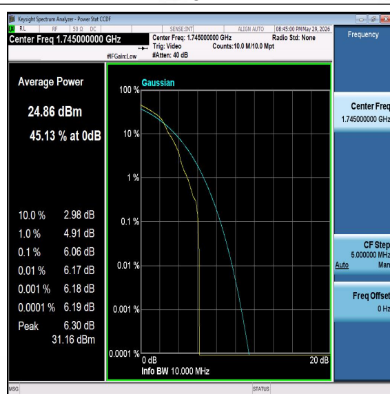
Band66-10MHz-16QAM-132322-PASS
