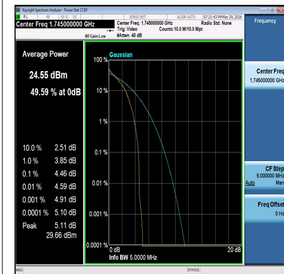
Band66-5MHz-QPSK-132322-PASS
