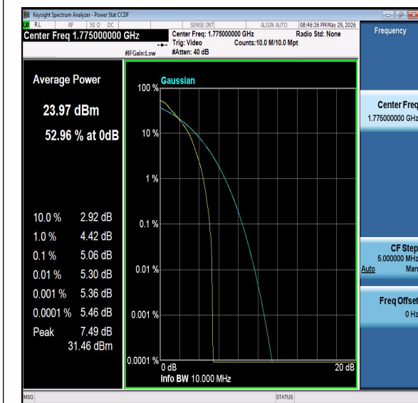
Band66-10MHz-QPSK-132622-PASS
