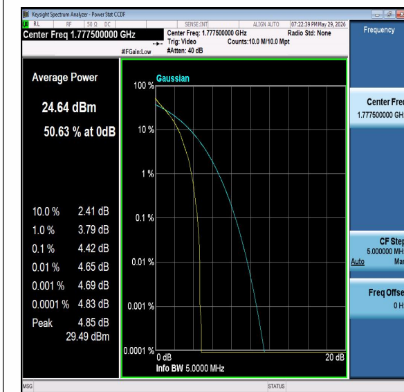
Band66-5MHz-QPSK-132647-PASS
