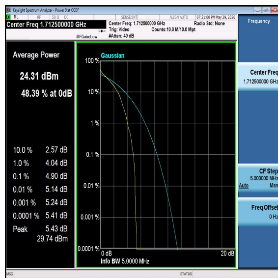
Band66-5MHz-16QAM-131997-PASS
