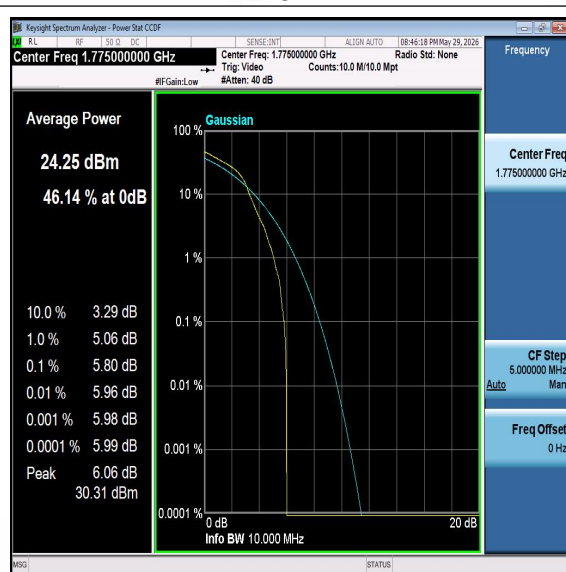
Band66-10MHz-16QAM-132622-PASS
