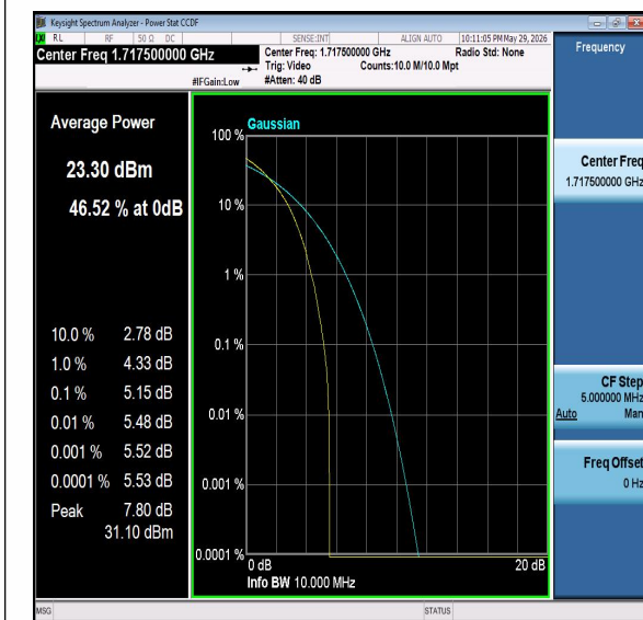
Band66-15MHz-QPSK-132047-PASS
