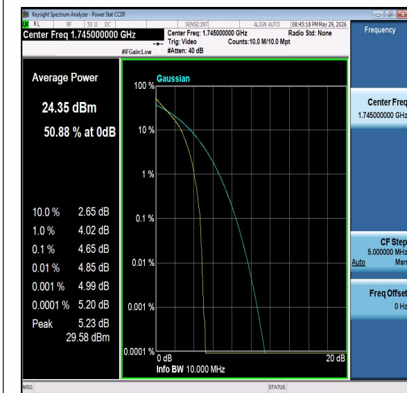
Band66-10MHz-QPSK-132322-PASS
