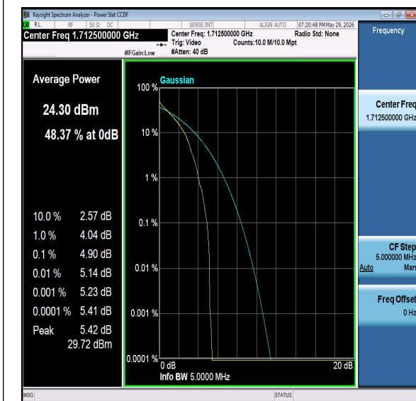
Band66-5MHz-QPSK-131997-PASS
