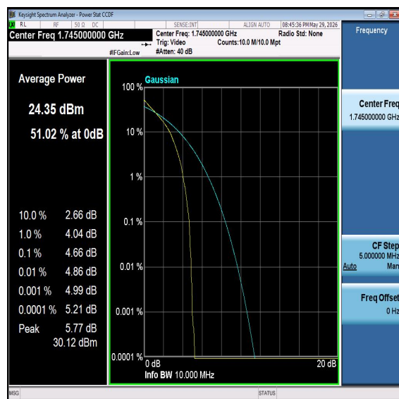
Band66-10MHz-16QAM-132322-PASS
