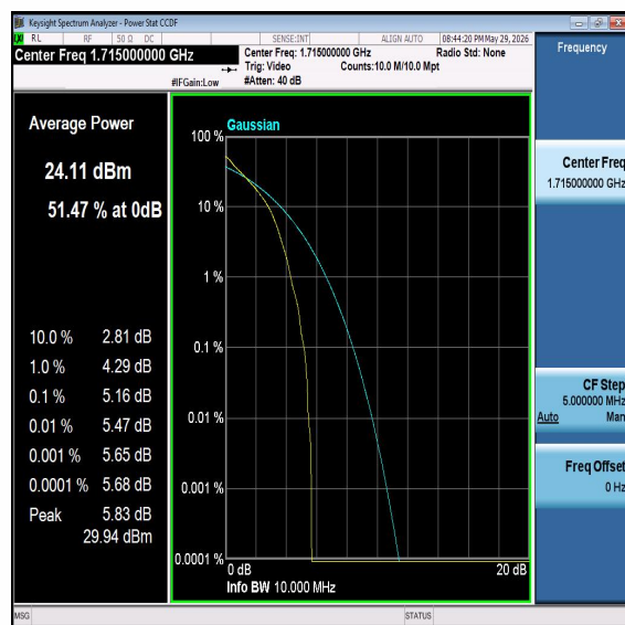
Band66-10MHz-16QAM-132022-PASS
