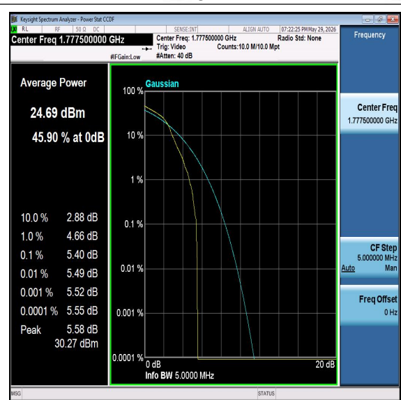
Band66-5MHz-16QAM-132647-PASS
