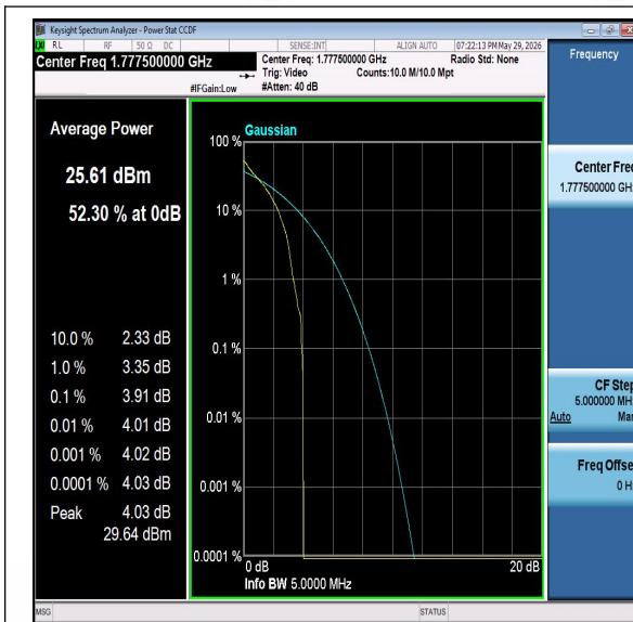
Band66-5MHz-QPSK-132647-PASS
