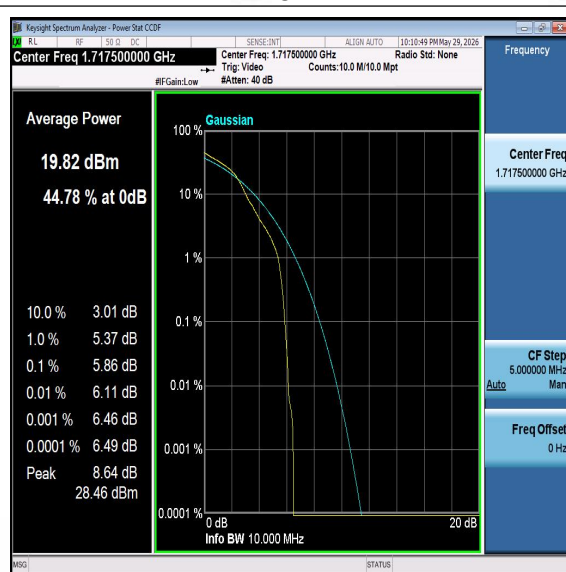
Band66-15MHz-16QAM-132047-PASS
