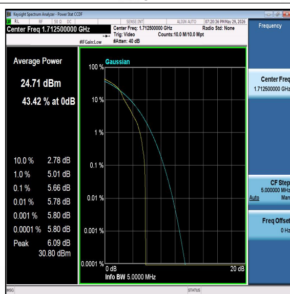
Band66-5MHz-16QAM-131997-PASS
