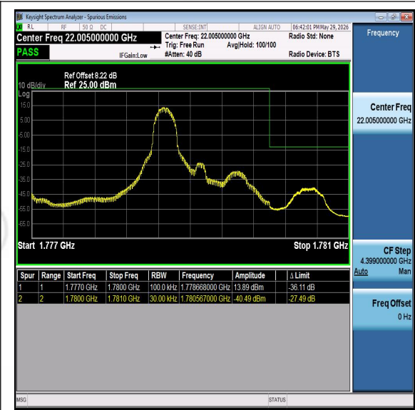
Band66-3MHz-QPSK-132657-PASS
