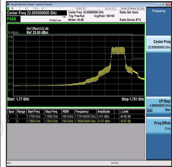
Band66-10MHz-QPSK-132622-PASS
