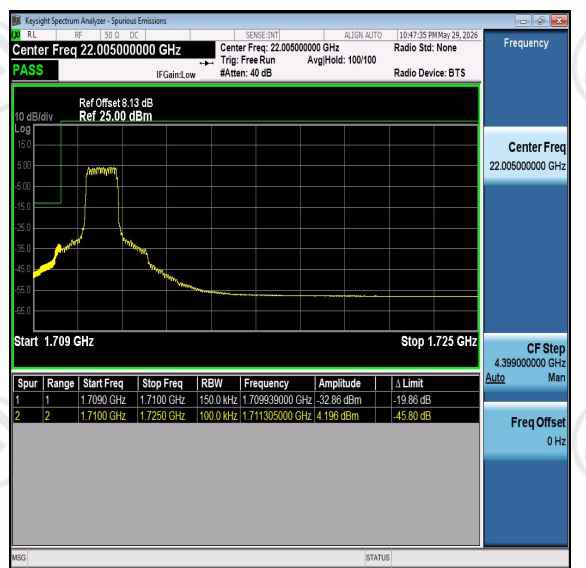
Band66-15MHz-16QAM-132047-PASS
