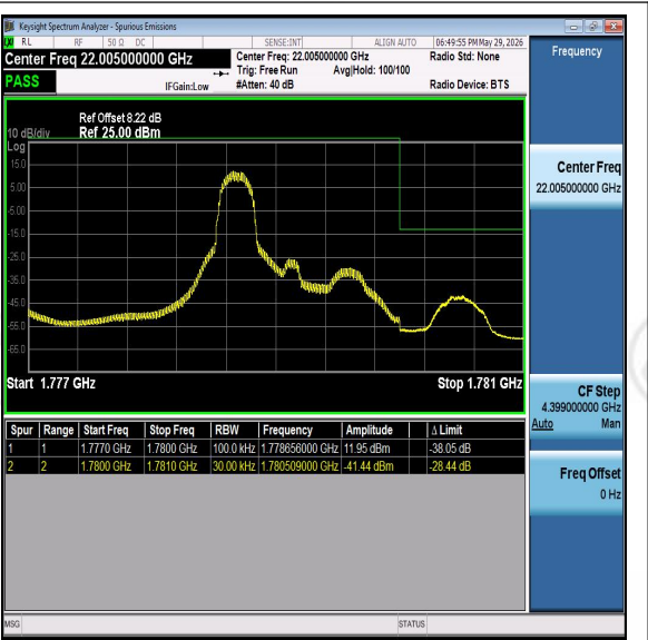
Band66-3MHz-16QAM-132657-PASS
