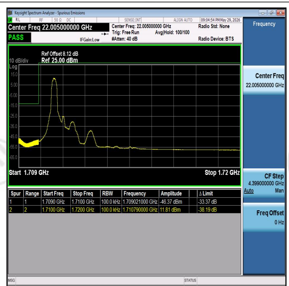
Band66-10MHz-16QAM-132022-PASS
