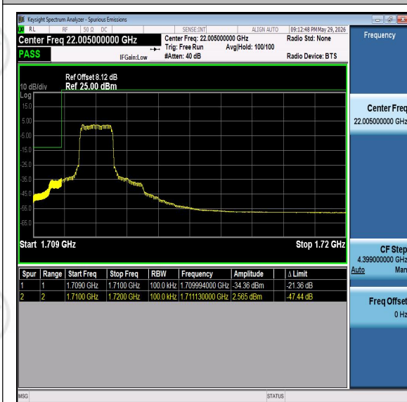
Band66-10MHz-QPSK-132022-PASS
