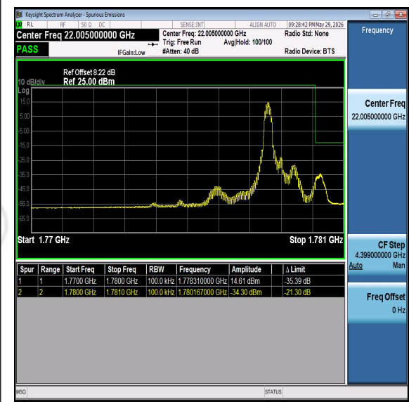
Band66-10MHz-QPSK-132622-PASS
