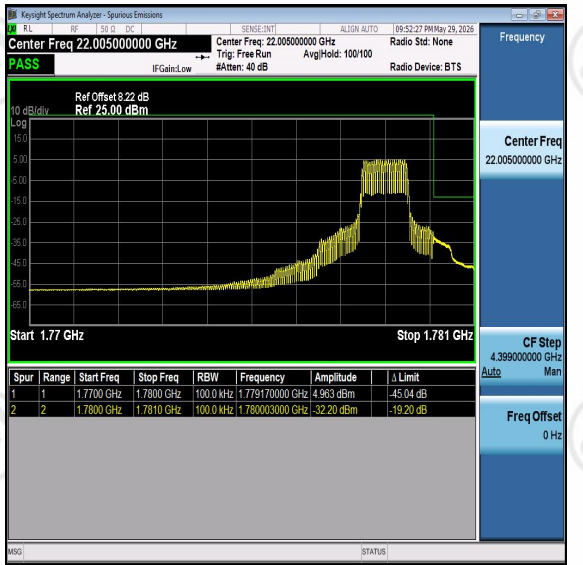
Band66-10MHz-16QAM-132622-PASS
