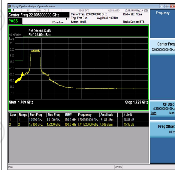
Band66-15MHz-QPSK-132047-PASS
