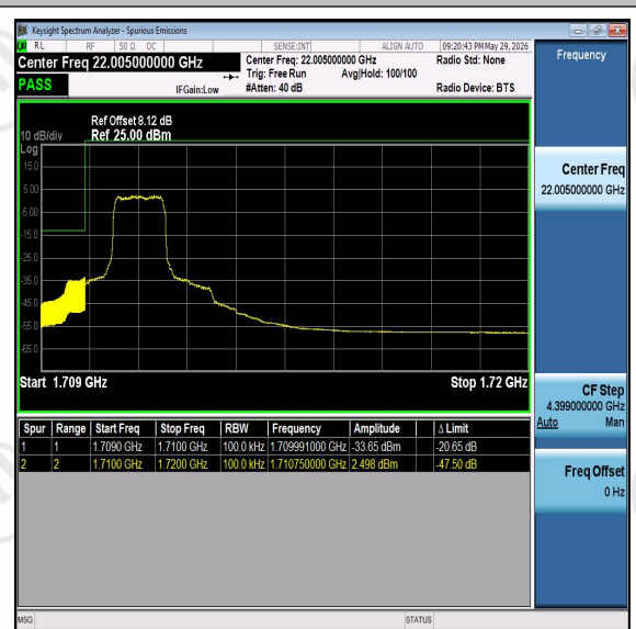
Band66-10MHz-16QAM-132022-PASS
