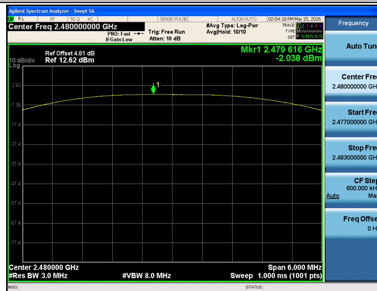
BLE_2Mbps_2480
