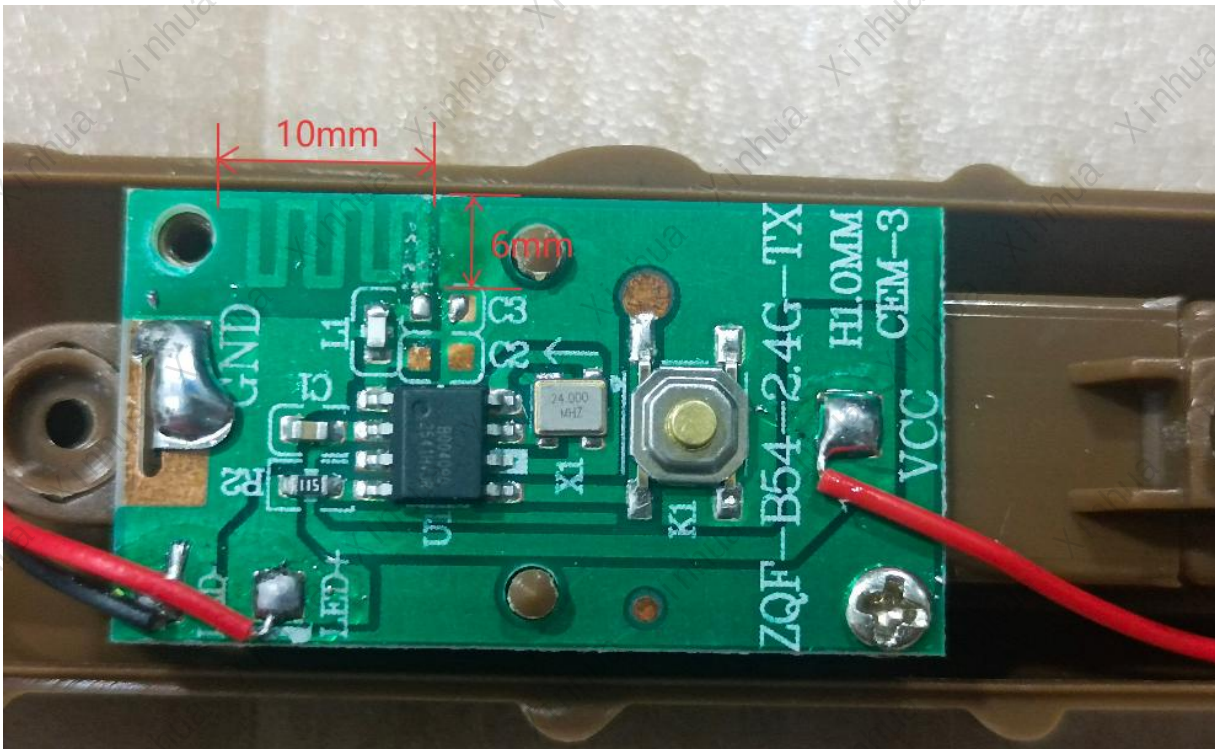
Antenna Dimensions
