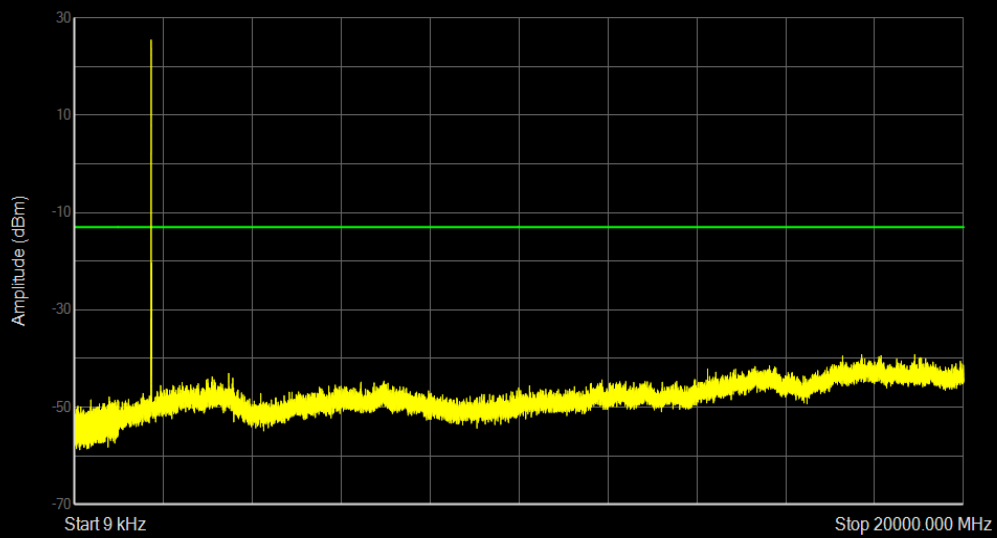
Band66 16QAM BW=5MHz Channel=132322 RB Size=1 Position=#0
