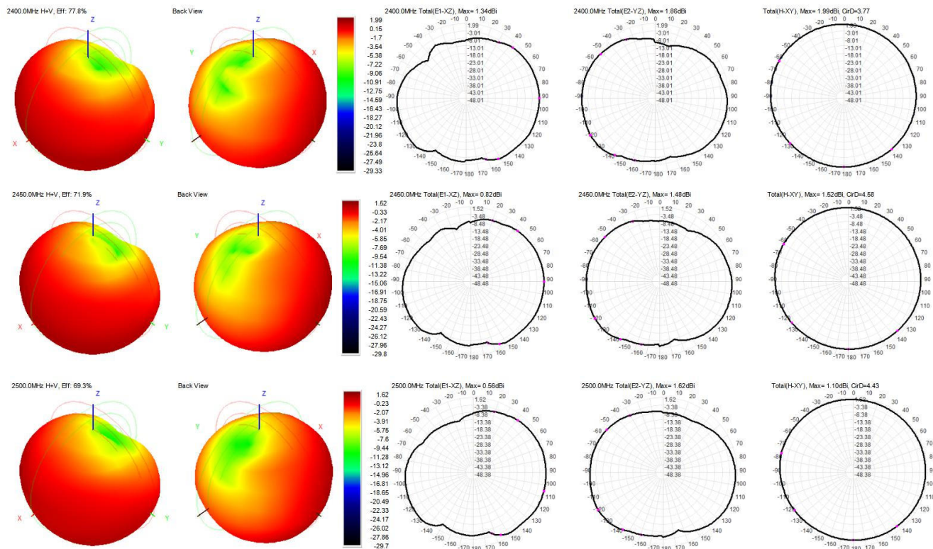
Antenna field type diagram
