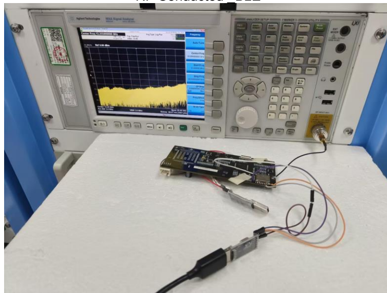
RF Conducted BLE
