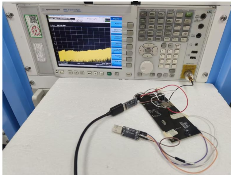
RF Conducted WIFI
