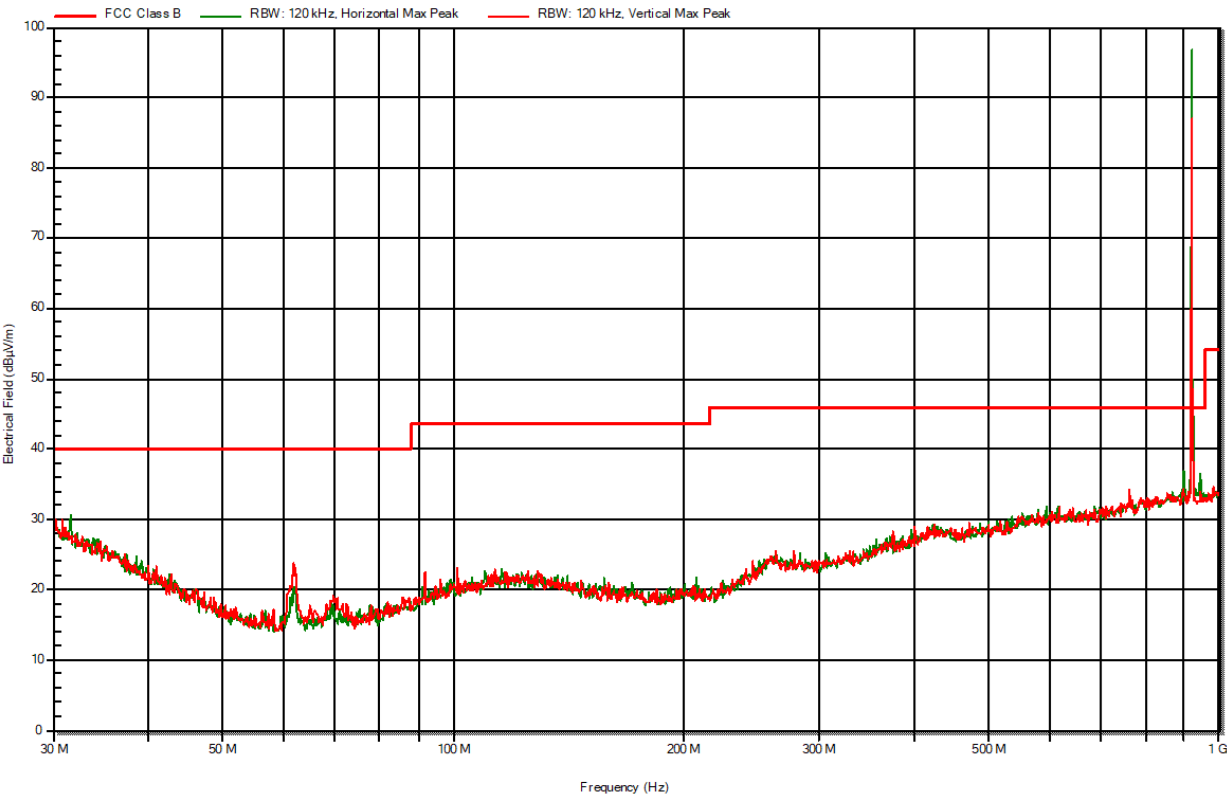
Figure 3 Electric field emissions Plot, 30MHz to 1GHz, Operation on channel 5 920MHz - Peak detector scan
