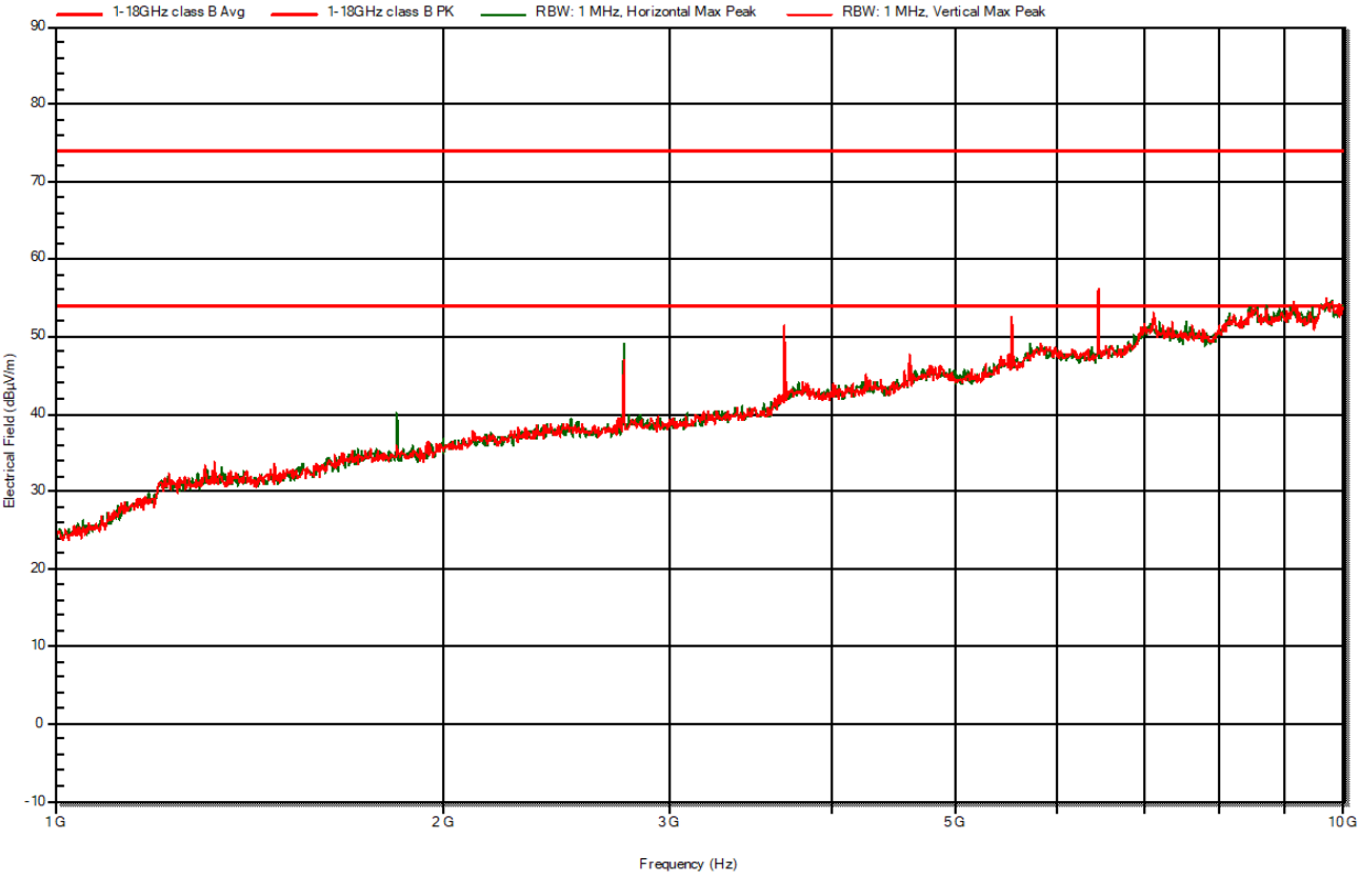
Figure 6 Electric field emissions Plot, 1GHz to 10GHz, Operation on channel 5 920MHz - Peak detector scan
