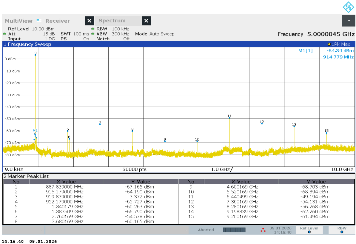
Figure 9 Conducted emissions 9kHz to 10GHz. Operation on channel 5 920MHz.
