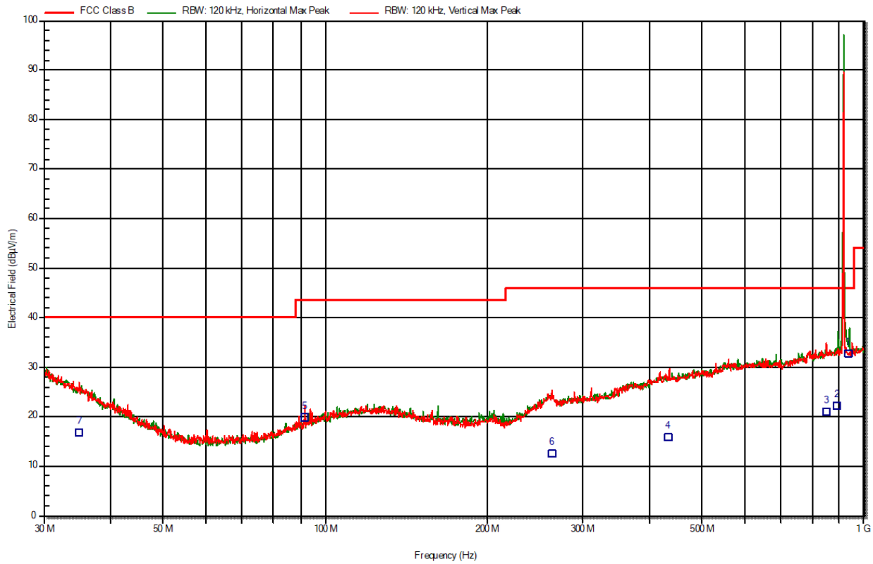
Figure 2 Electric field emissions Plot, 30MHz to 1GHz, Operation on channel 0 915MHz
