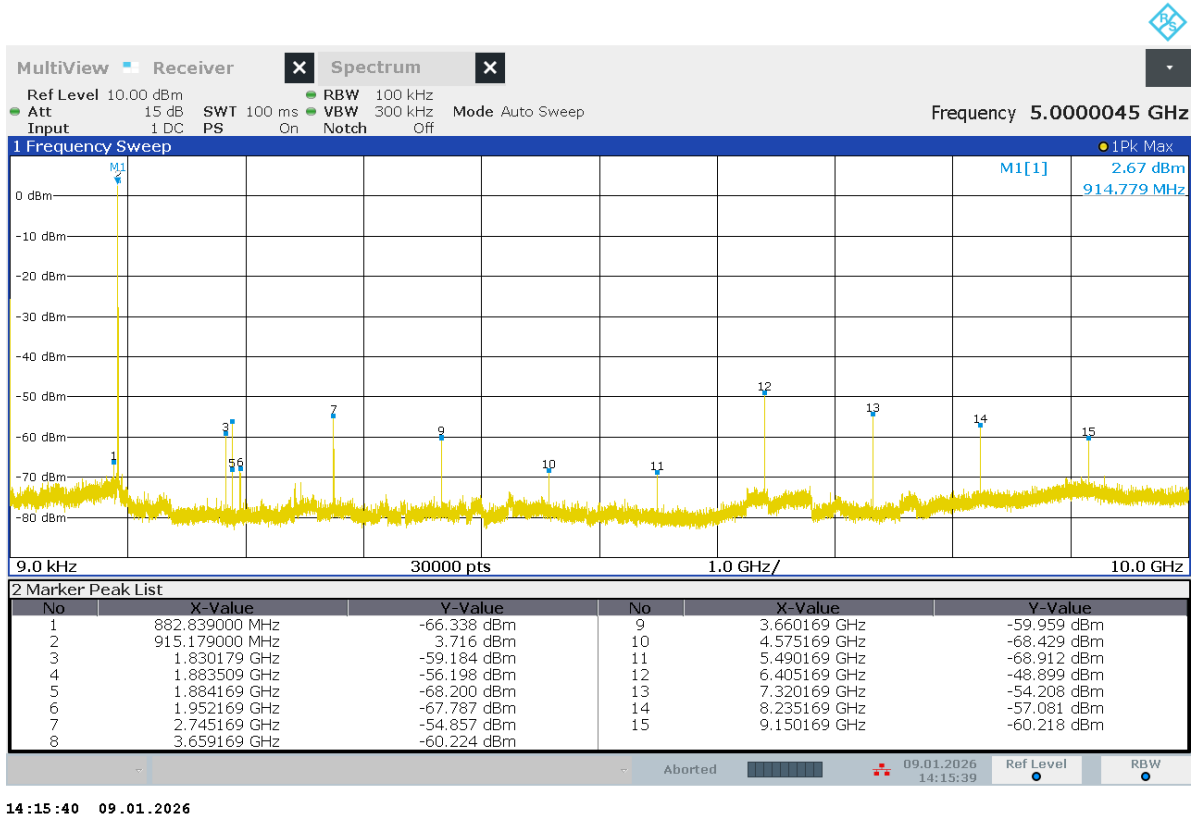
Figure 8 Conducted emissions 9kHz to 10GHz. Operation on channel 0 915MHz.
