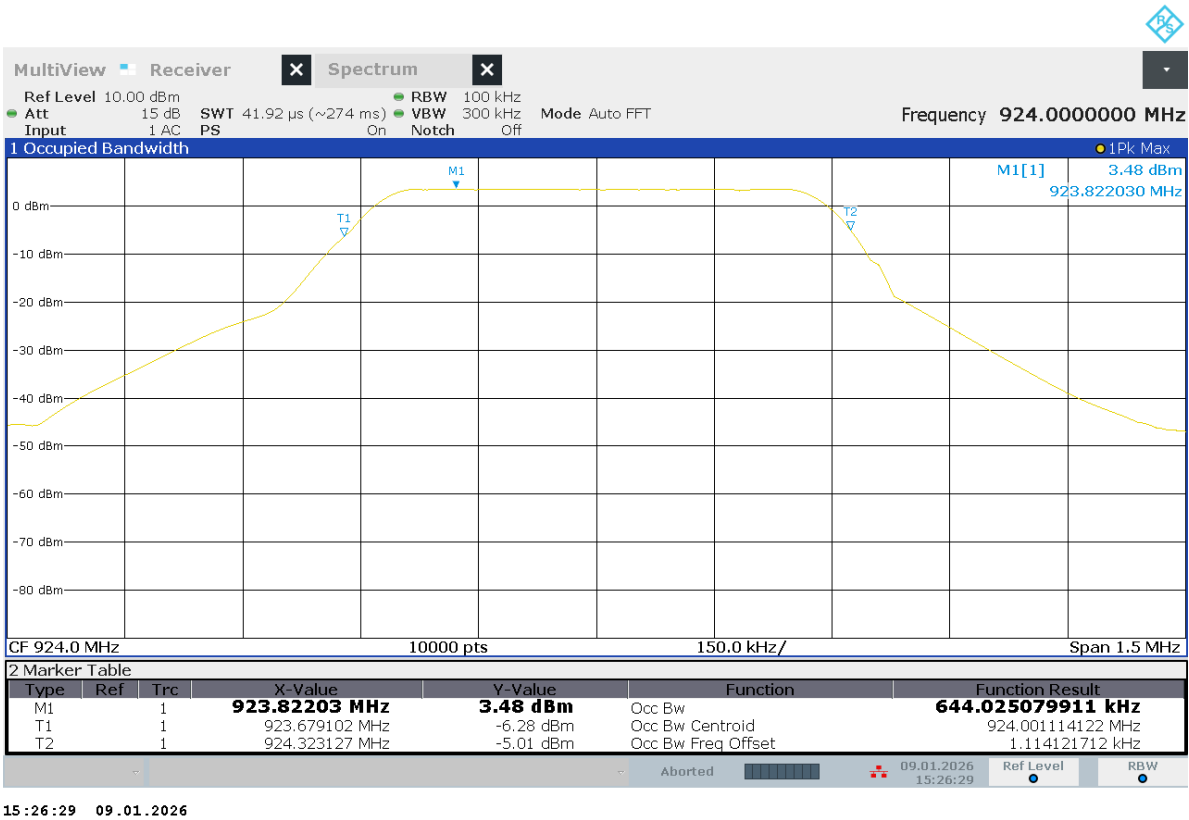
Figure 16 99% Occupied Bandwidth. Operation on channel 9 924MHz
