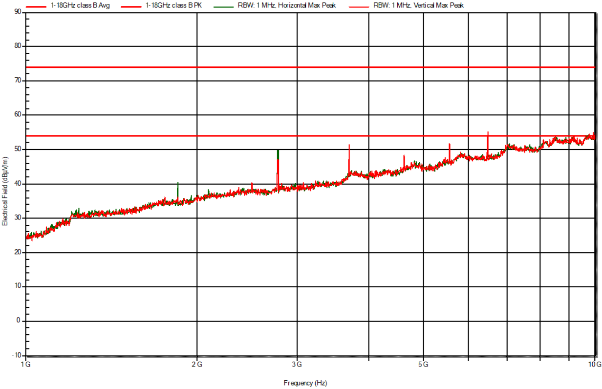
Figure 7 Electric field emissions Plot, 1GHz to 10GHz, Operation on channel 9 924MHz – Peak detector scan
