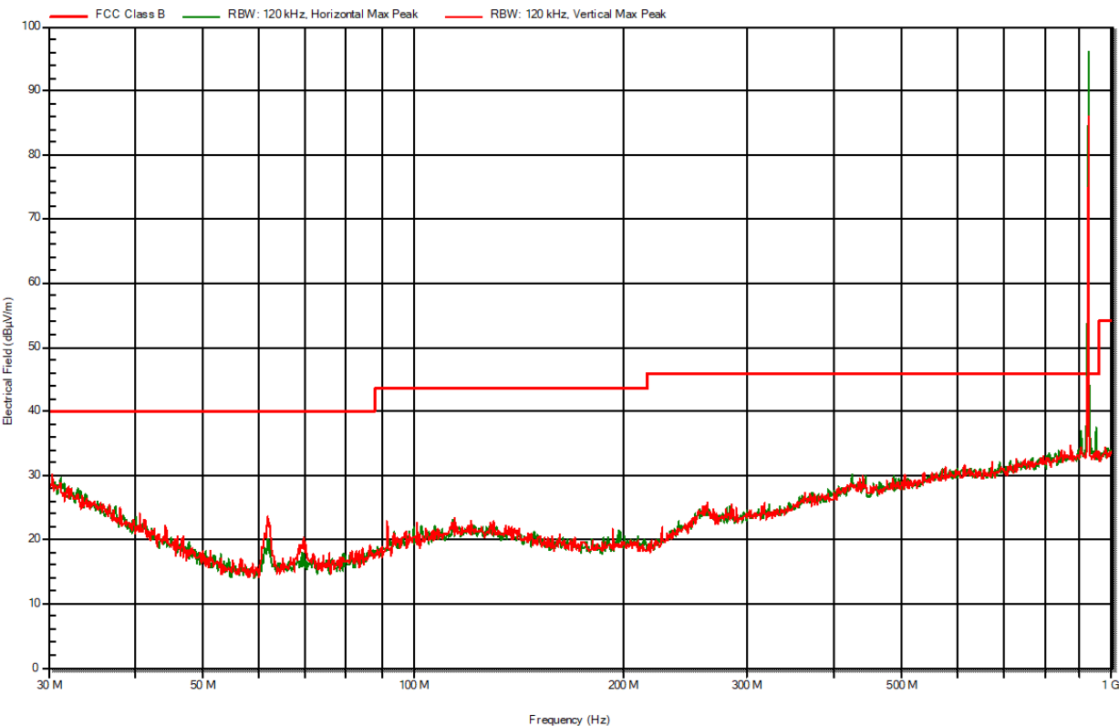
Figure 4 Electric field emissions Plot, 30MHz to 1GHz, Operation on channel 9 924MHz - Peak detector scan
