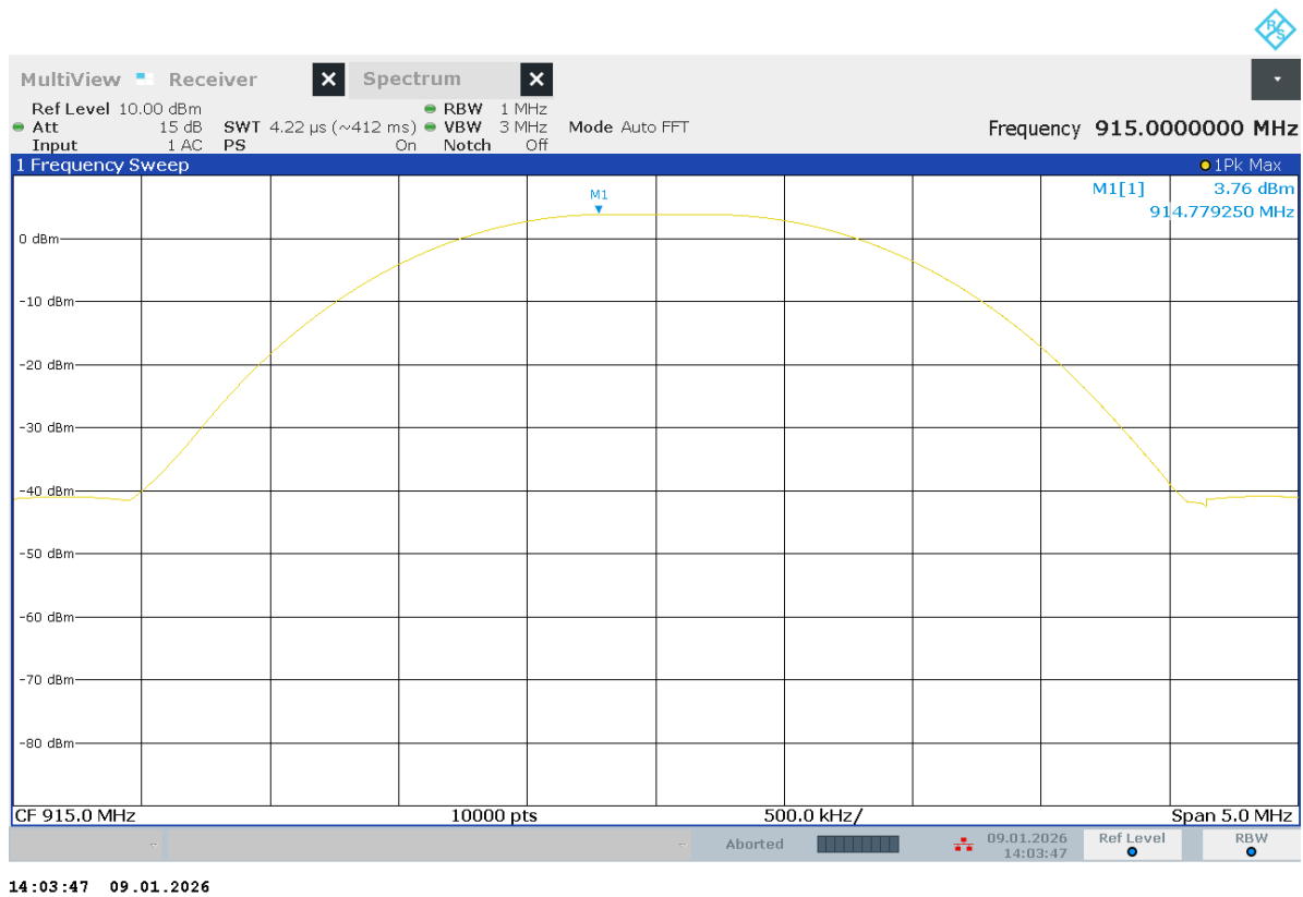
Figure 17 Peak output power, Operation on channel 0 915MHz
