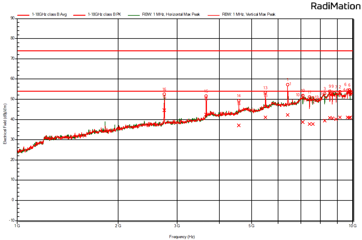
Figure 5 Electric field emissions Plot, 1GHz to 10GHz. Operation on channel 0 915MHz
