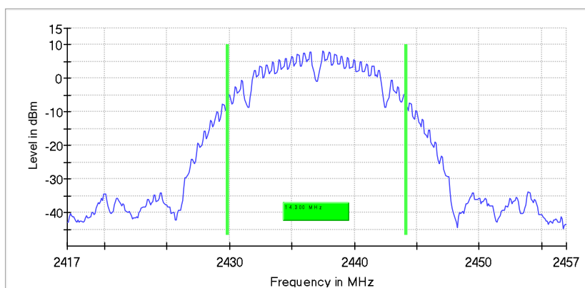
99 % Bandwidth
