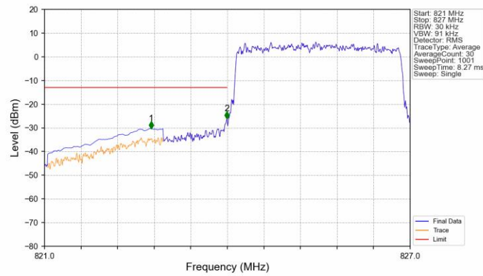
Band26b_3MHz_QPSK_LCH_825.5MHz_RB_15_0_NTNV
