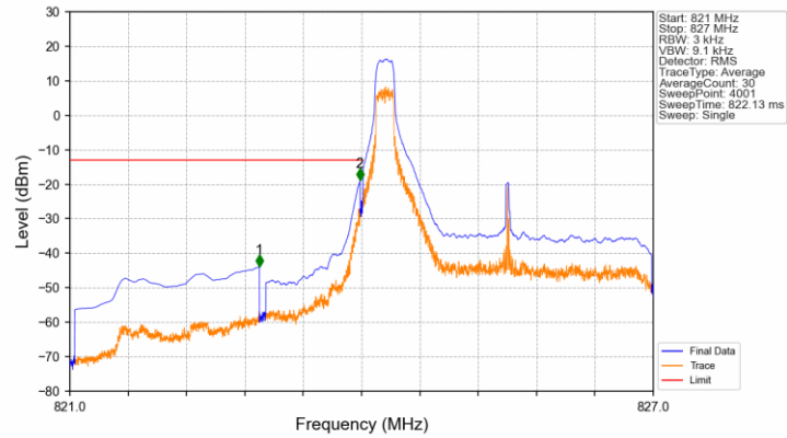
Band26b_3MHz_QPSK_LCH_825.5MHz_RB_1_0_NTNV
