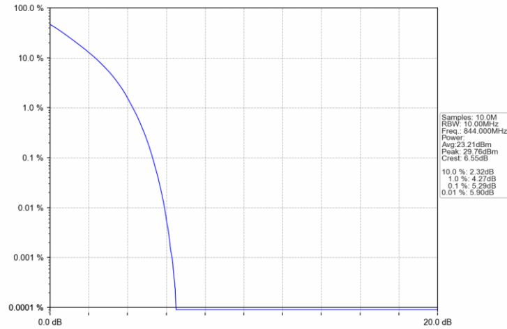
Band26b_10MHz_QPSK_HCH_844MHz_RB_50_0_NTNV
