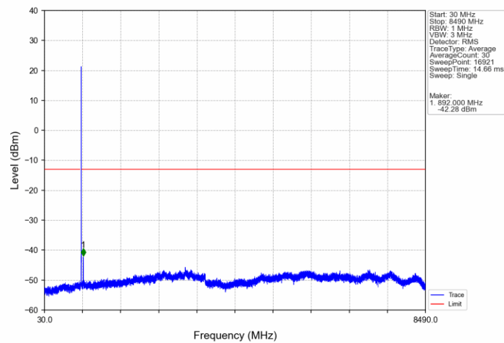
Band26b_3MHz_16QAM_HCH_847.5MHz_RB_1_0_NTNV
