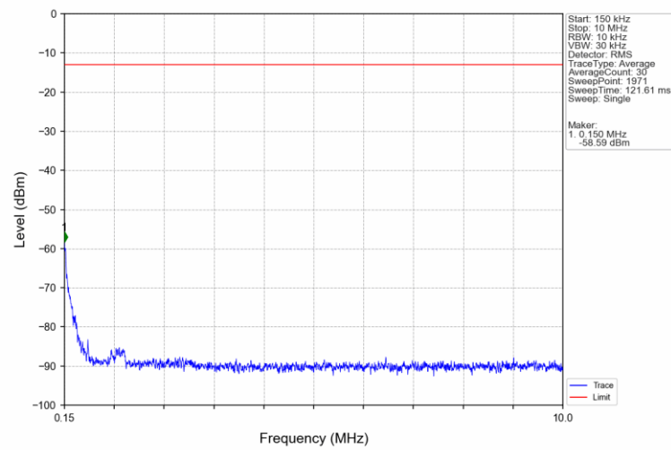
Band26b_3MHz_16QAM_MCH_836.5MHz_RB_1_0_NTNV
