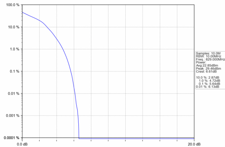
Band26b_10MHz_16QAM_LCH_829MHz_RB_50_0_NTNV
