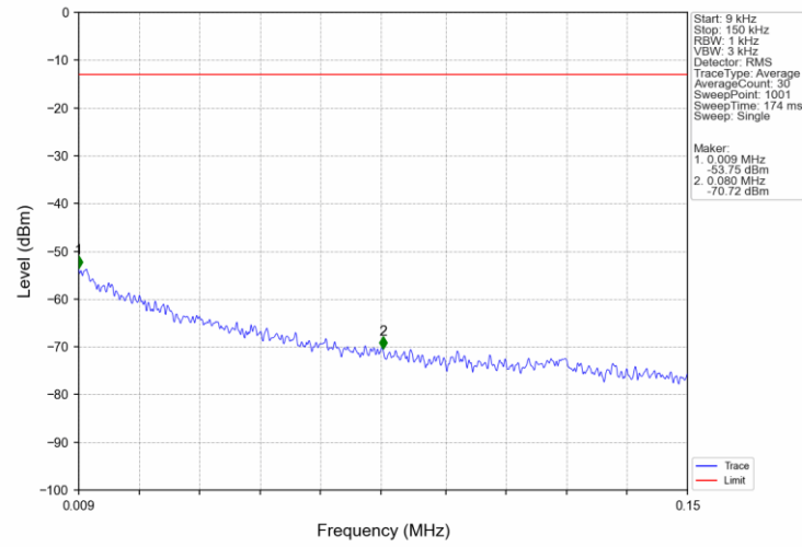
Band26b_3MHz_16QAM_MCH_836.5MHz_RB_1_0_NTNV
