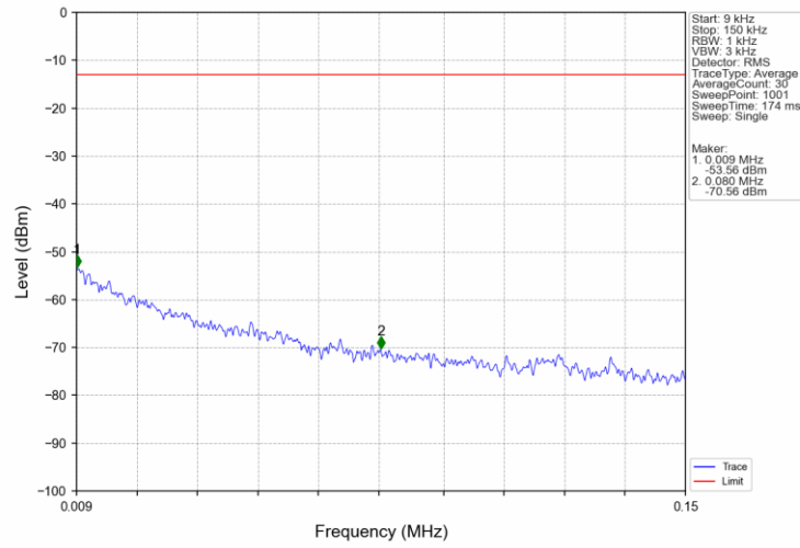
Band26b_3MHz_16QAM_HCH_847.5MHz_RB_1_0_NTNV
