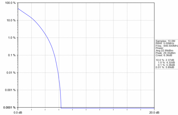
Band26b_5MHz_QPSK_HCH_846.5MHz_RB_25_0_NTNV
