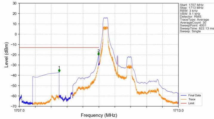
Band4_1.4MHz_QPSK_LCH_1710.7MHz_RB_1_0_NTNV
