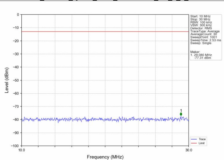
Band4_1.4MHz_QPSK_MCH_1732.5MHz_RB_1_0_NTNV
