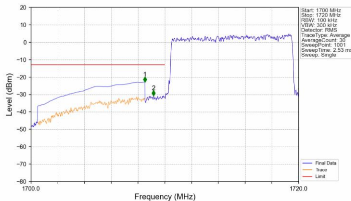
Band66_10MHz_16QAM_LCH_1715MHz_RB_50_0_NTNV
