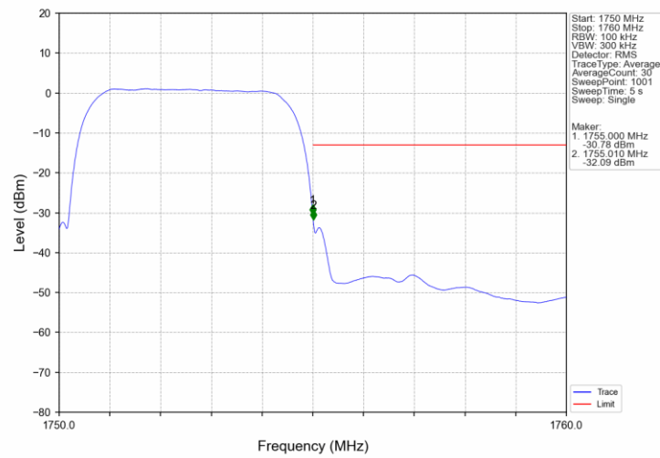
Band4_RMC_HCH_1752.6MHz_12.2kbps_RMC_NTNV
