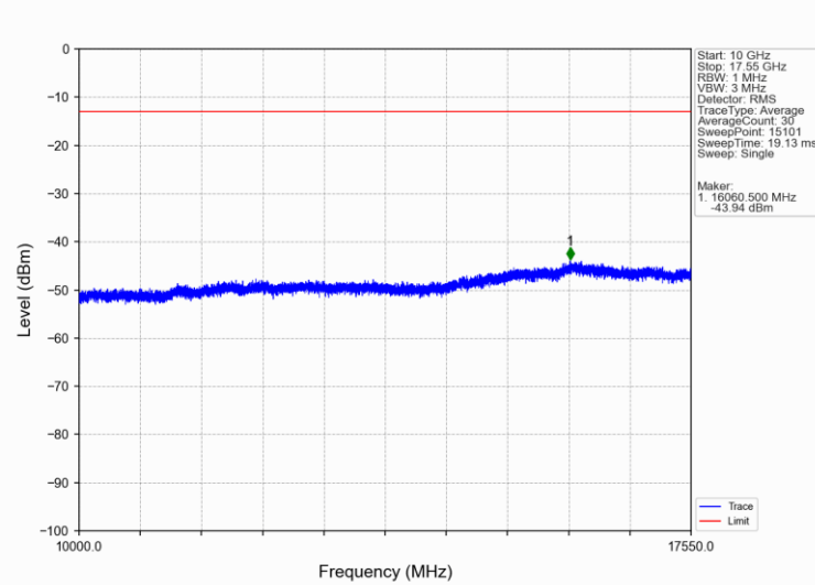
Band4_RMC_MCH_1732.6MHz_12.2kbps_RMC_NTNV
