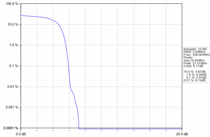
Band5 HSDPA MCH 836.6MHz Subtest 1 NTNV
