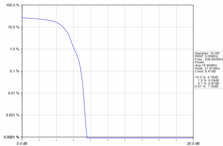
Band5 HSUPA MCH 836.6MHz Subtest 1 NTN
