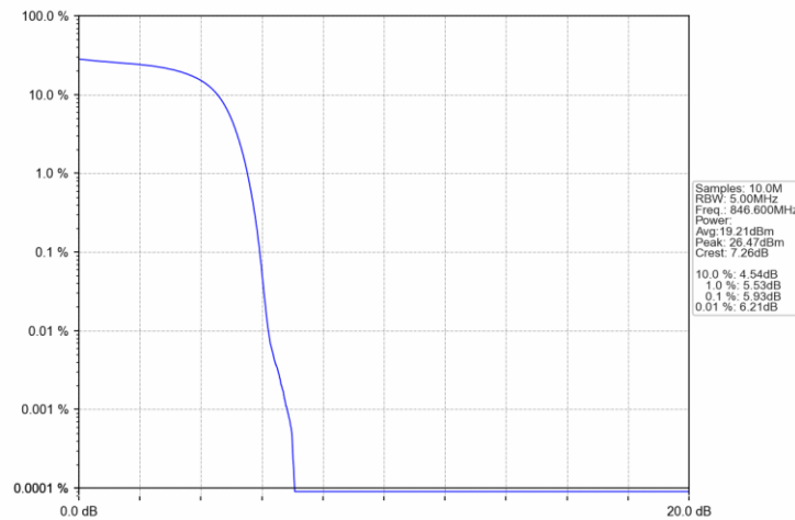
Band5 HSDPA HCH 846.6MHz Subtest 1 NTNV
