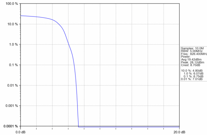
Band5 HSUPA LCH 826.4MHz Subtest 1 NTN
