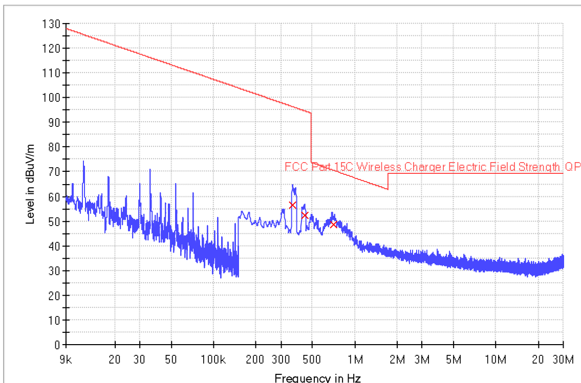
FCC Part 9K-30M(dBuV)
