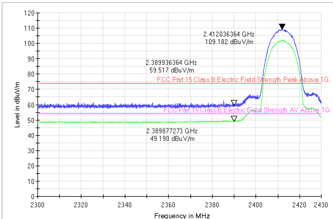
Electric Field Strength 1-18GdBuV TX Band Edge+EIRP
