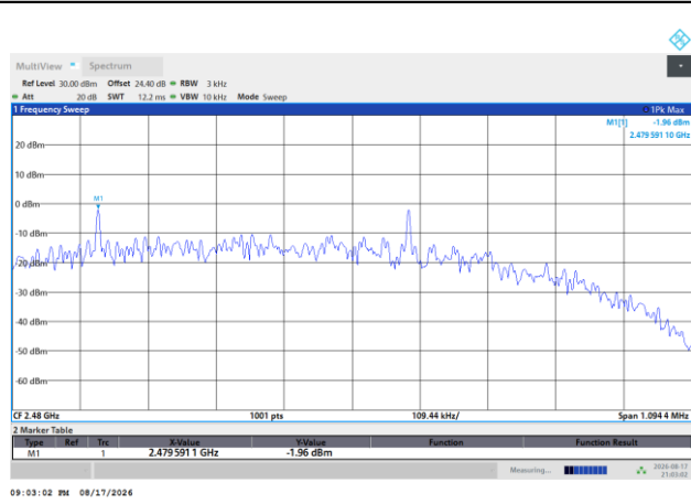
Power Density (dBm/3kHz) Plot Channel 39
