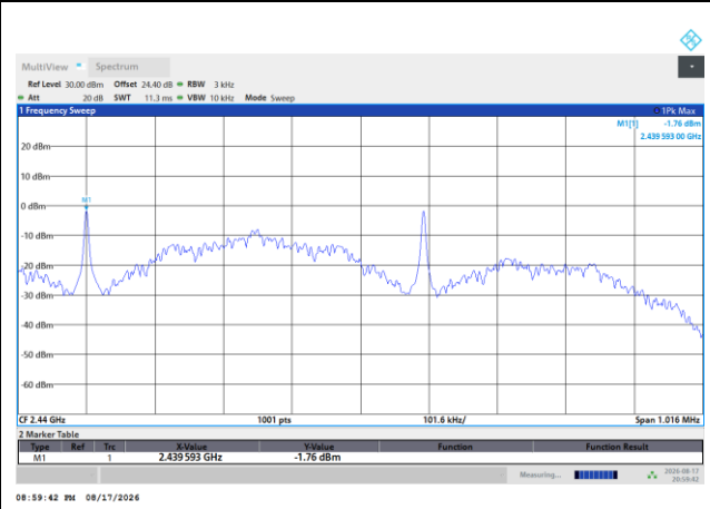
Power Density (dBm/3kHz) Plot Channel 19
