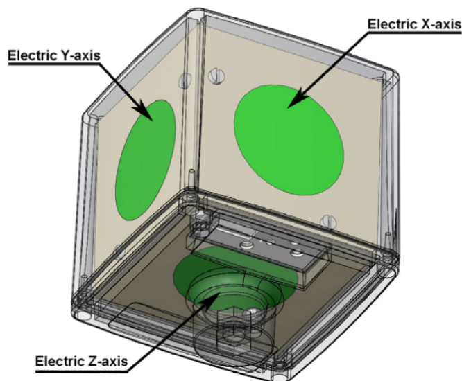
EHP-200A/EHP-200AC axes
