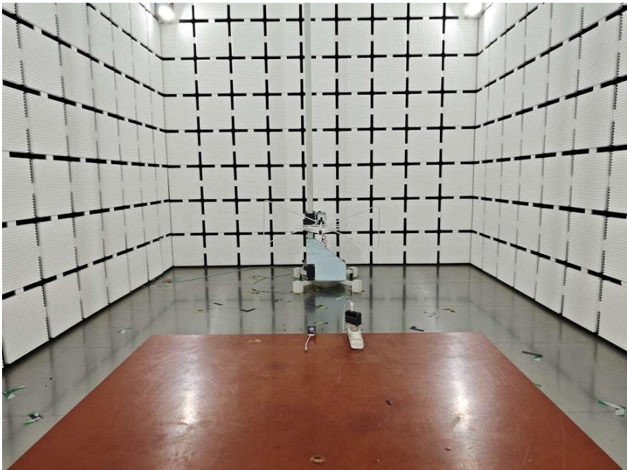
Radiated Emission Test View 4
