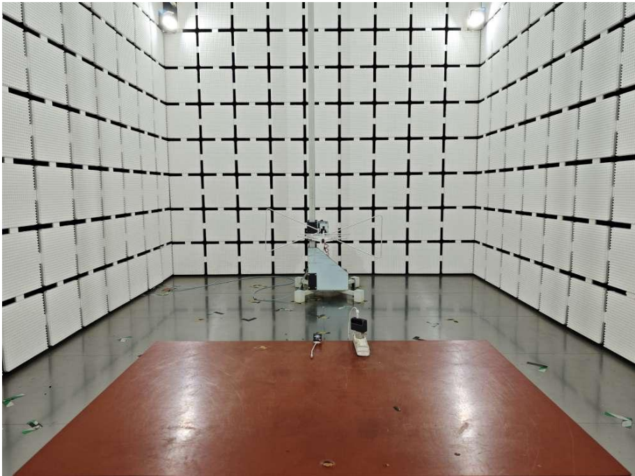
Radiated Emission Test View 3
