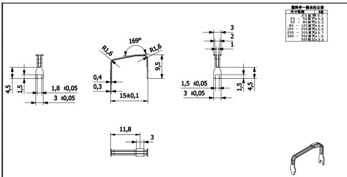
Antenna Top View [With Ruler]
