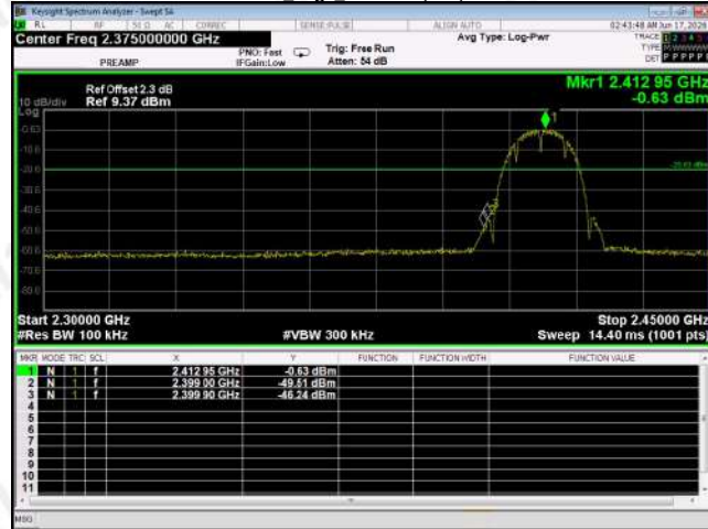
Band edge Emission,11b,Lowest
