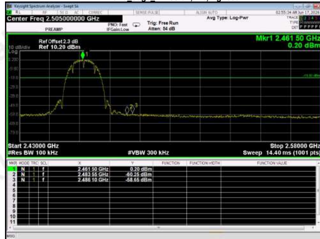
Band edge Emission,11b,Highest
