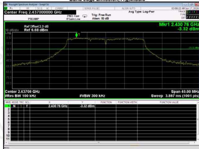
Band edge Emission,11g,Middle
