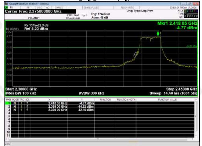
Band edge Emission,11g,Lowest
