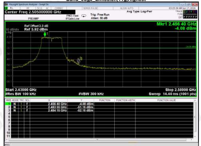
Band edge Emission,11g,Highest
