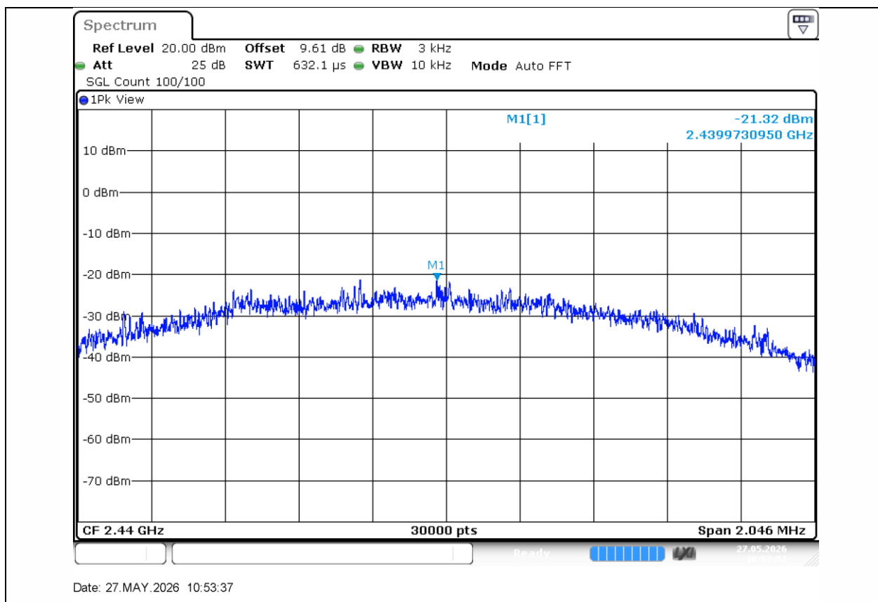
BLE_2M-Ant1-2440-PASS
