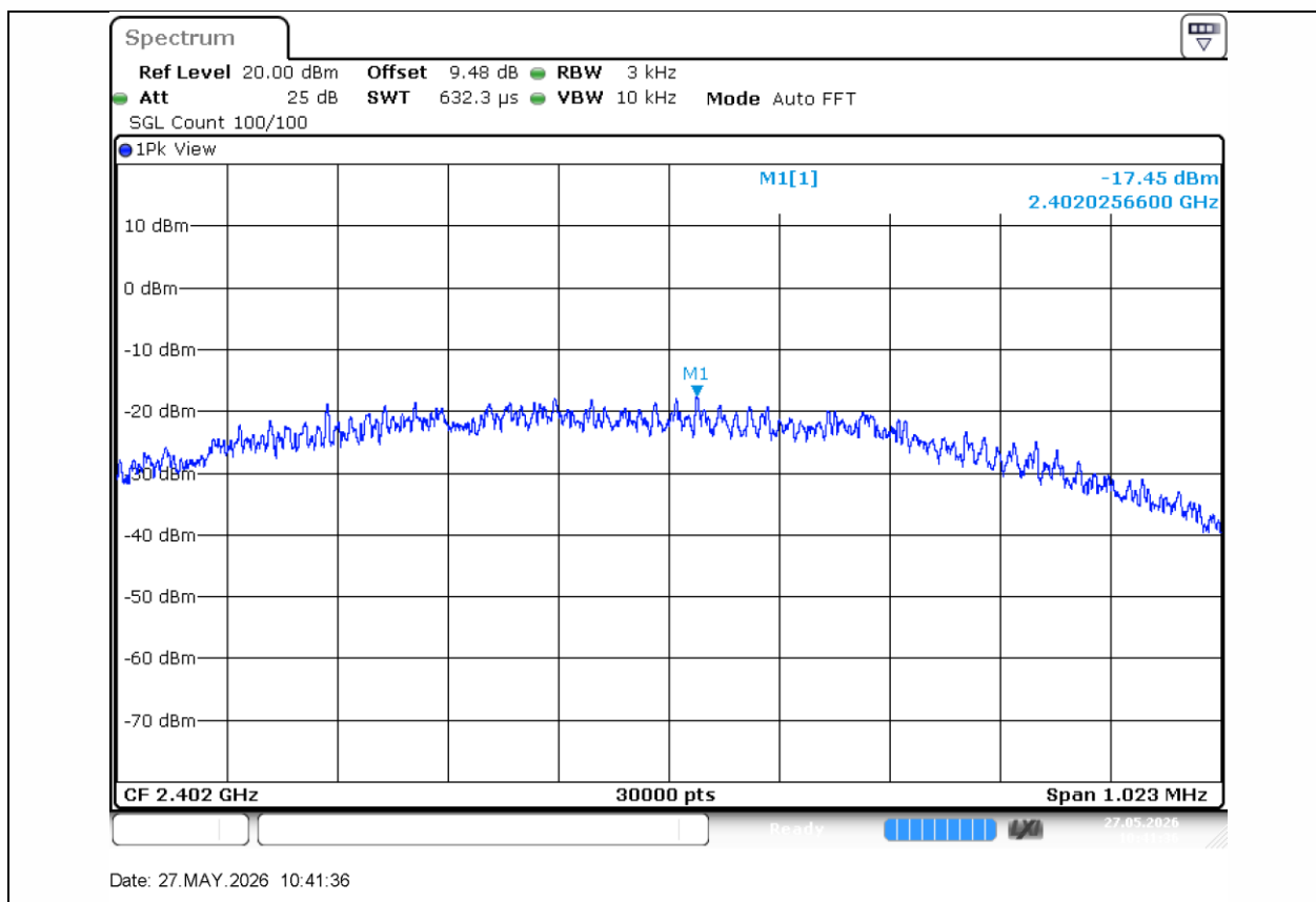
BLE_1M-Ant1-2402-PASS
