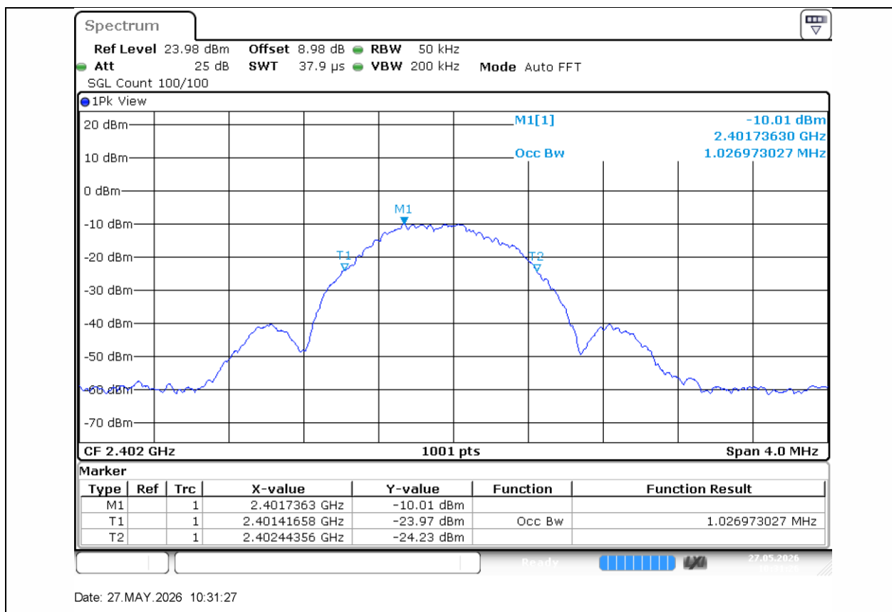
BLE_1M-Ant1-2402
