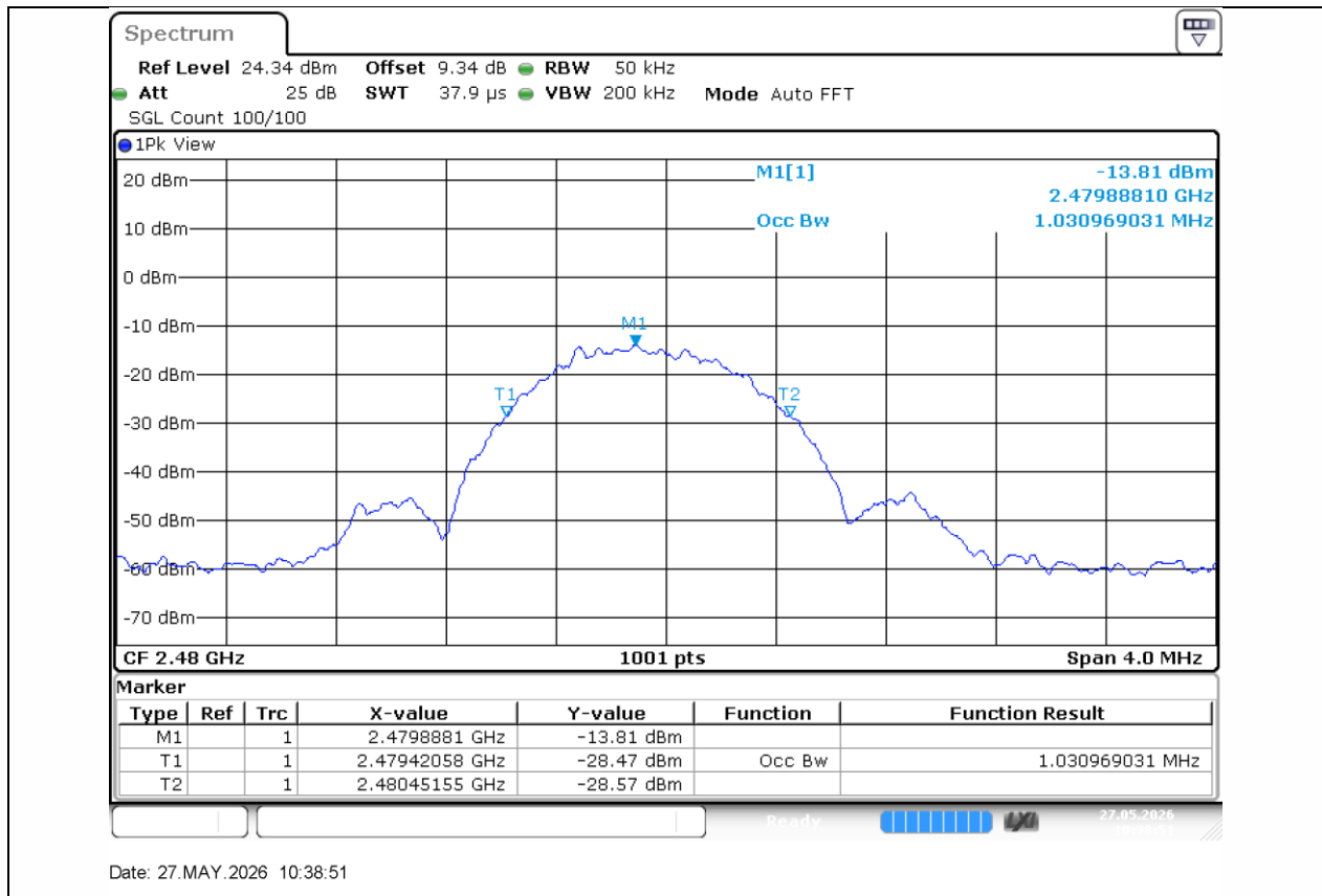
BLE_1M-Ant1-2480
