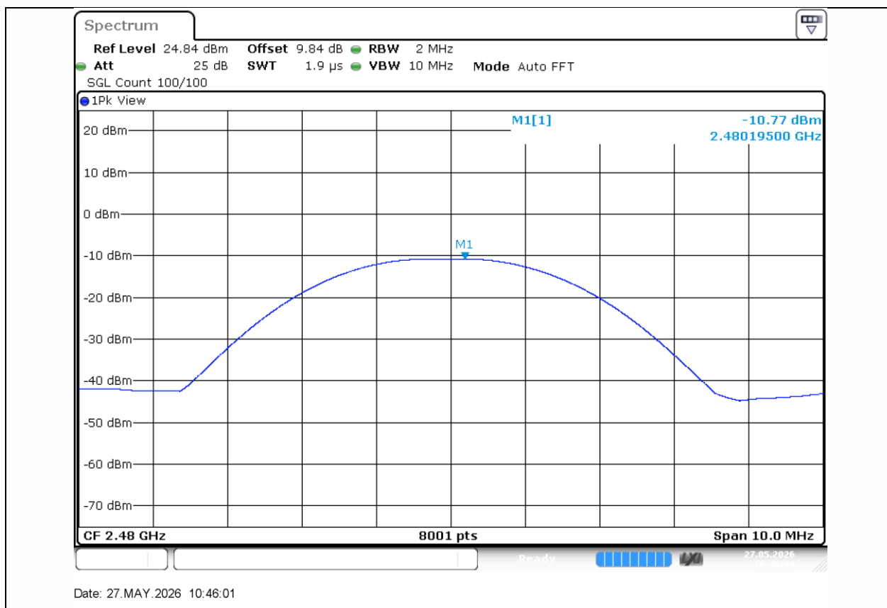
BLE_1M-Ant1-2480-PASS
