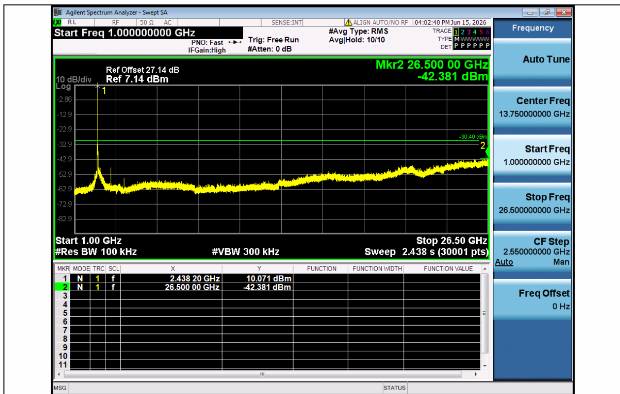
11G-Ant1-2437-1000~26500-PASS
