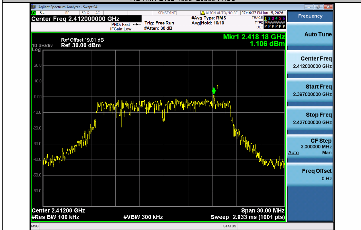
11G-Ant1-2412-0~Reference-PASS
