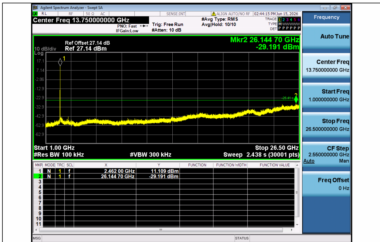
11B-Ant1-2462-1000~26500-PASS
