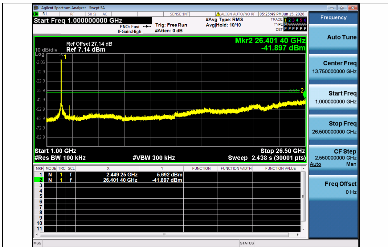
11N40SISO-Ant1-2437-1000~26500-PASS
