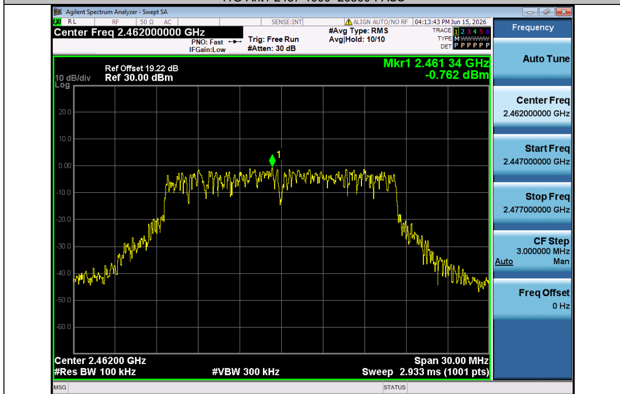
11G-Ant1-2462-0~Reference-PASS
