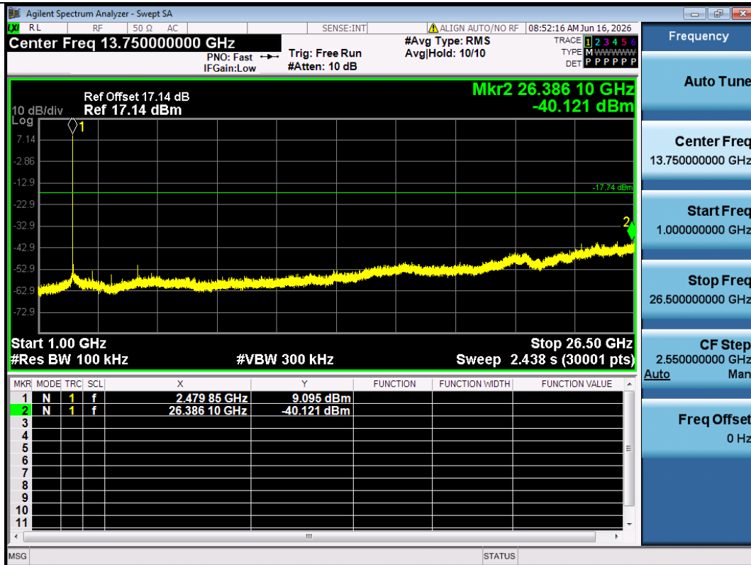
BLE_1M-Ant1-2480-1000~26500-PASS
