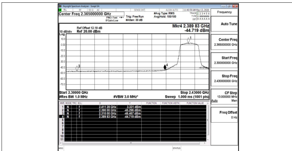
11G_Ant1_Low_2412_Peak
