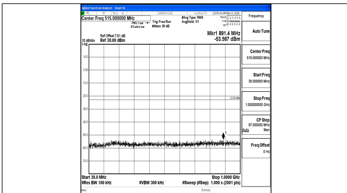
Band4_10MHz_16QAM_20350_1RB#0_30~1000_30~1000
