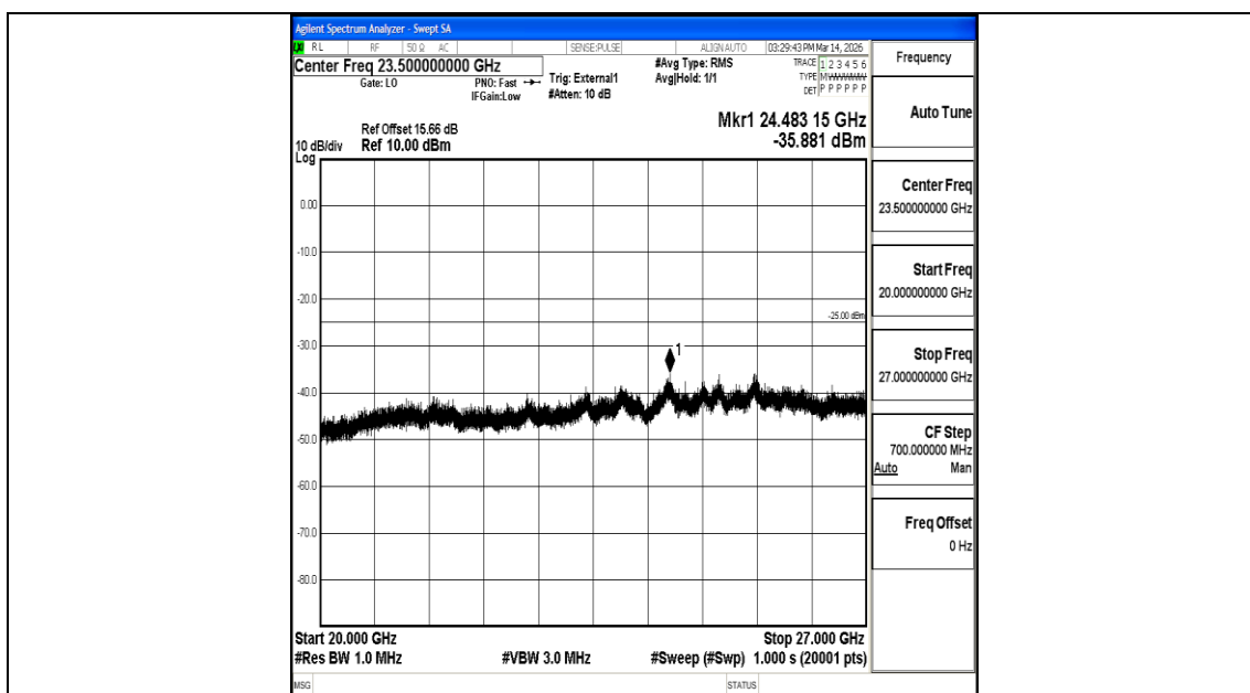
Band41_15MHz_QPSK_39725_1RB#0_20000~27000_20000~27000
