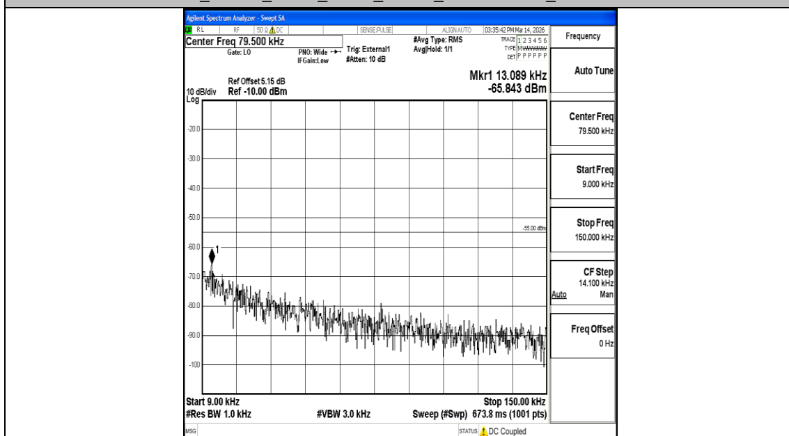
Band41_15MHz_16QAM_39725_1RB#0_0.009~0.15_0.009~0.15
