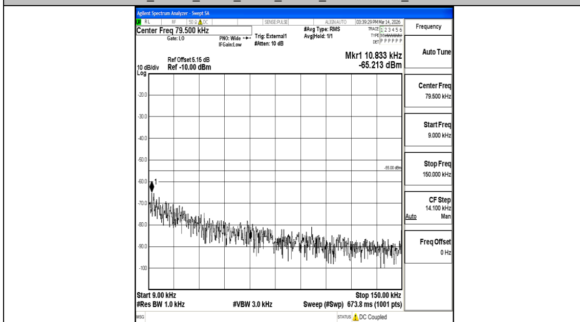
Band41_15MHz_16QAM_40620_1RB#0_0.009~0.15_0.009~0.15
