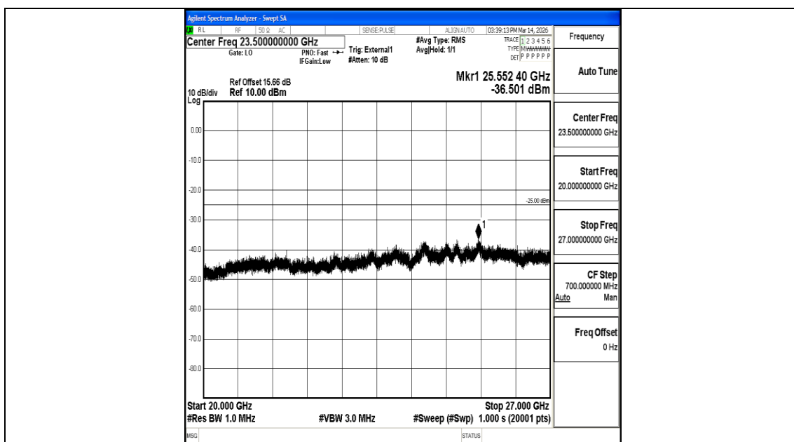
Band41_15MHz_QPSK_40620_1RB#0_20000~27000_20000~27000
