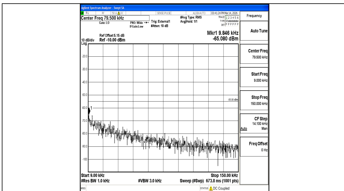
Band41_15MHz_QPSK_41515_1RB#0_0.009~0.15_0.009~0.15
