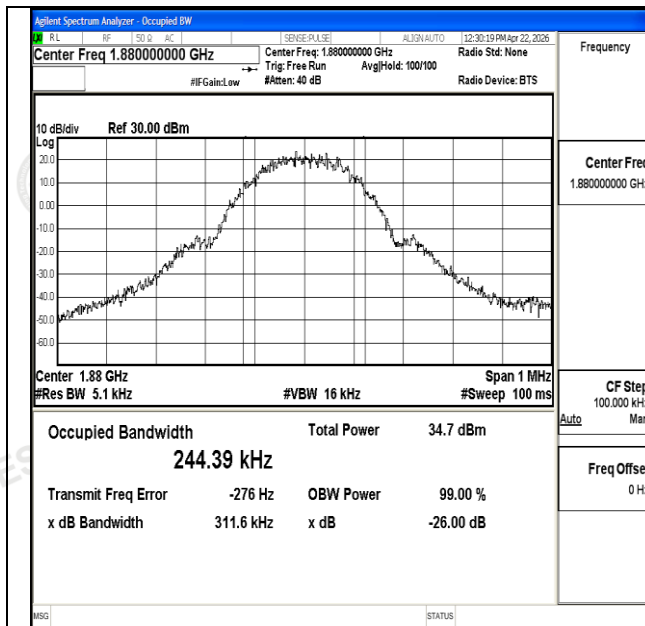
Channel 661 / 1880.0 MHz
