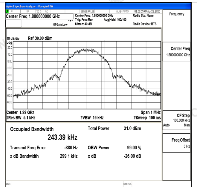
Channel 661 / 1880.0 MHz
