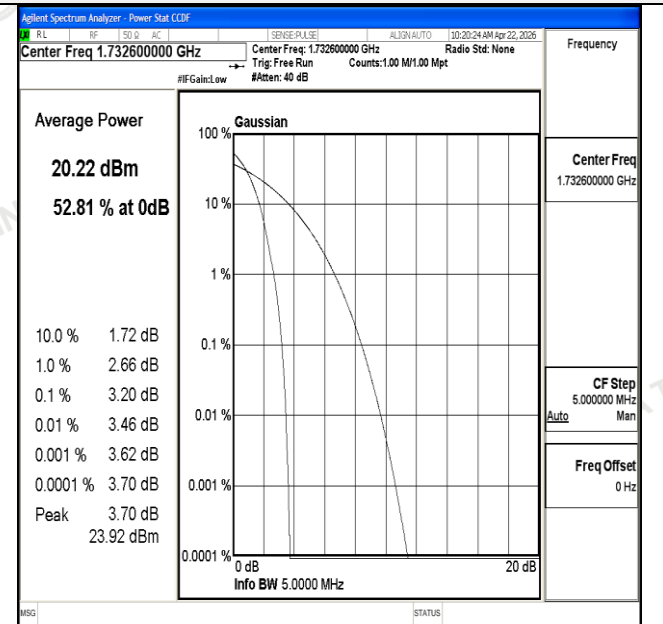
Channel 1413 / 1732.6 MHz
