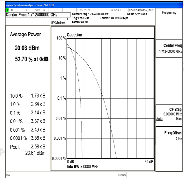
Channel 1312 / 1712.4 MHz
