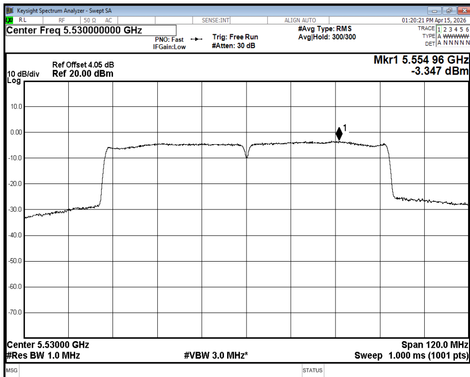
PSD NVNT ac80 5530MHz Ant1
