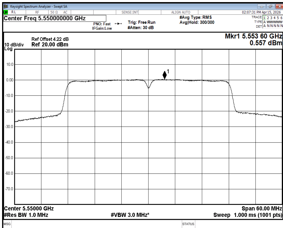
PSD NVNT ac40 5550MHz Ant1
