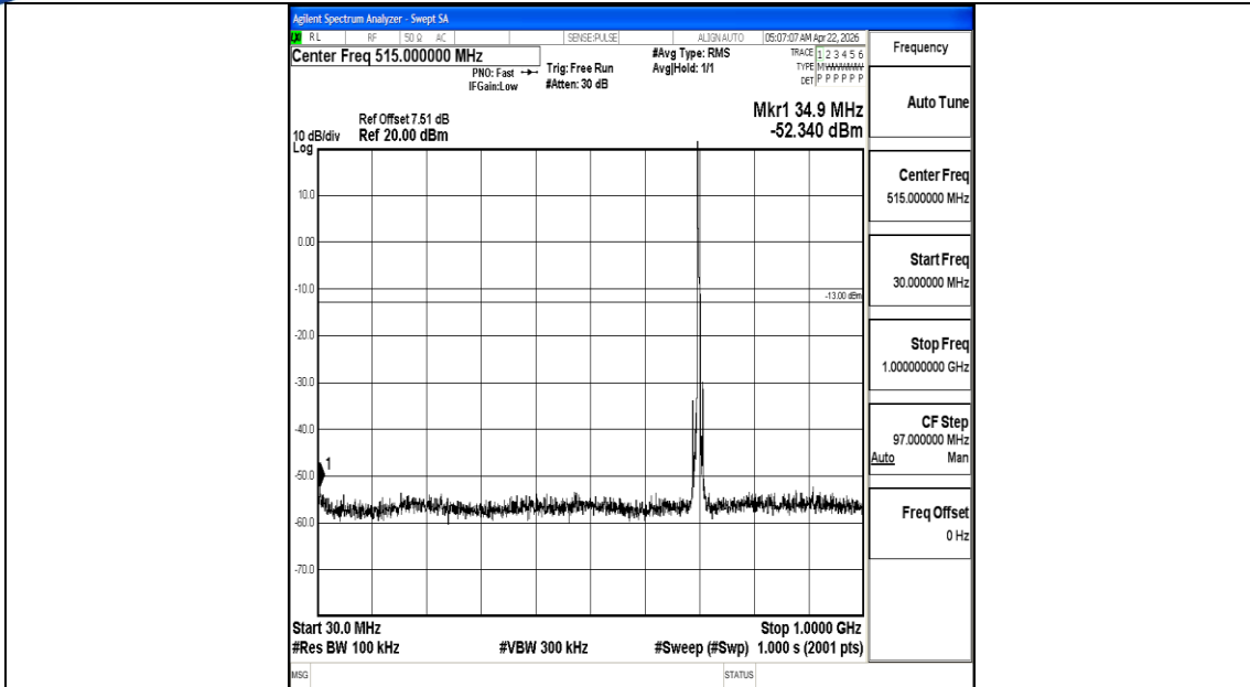
Band12_5MHz_QPSK_23095_1RB#0_30~1000_30~1000
