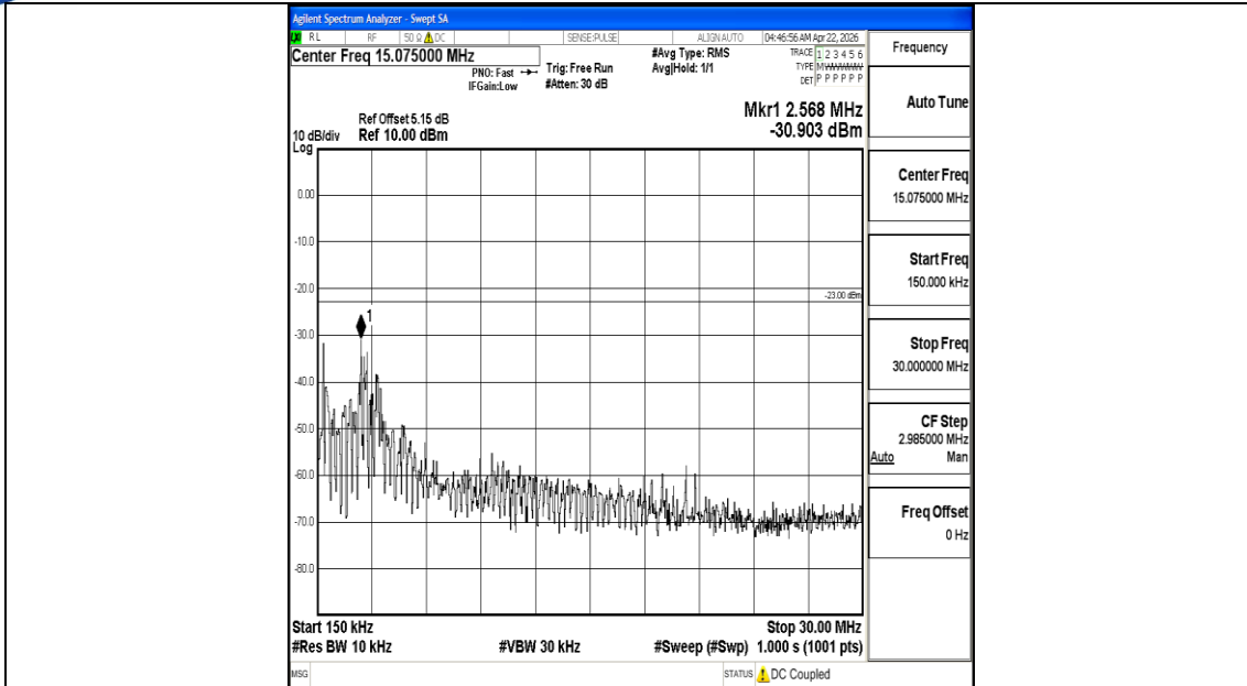
Band12_3MHz_16QAM_23165_1RB#0_0.15~30_0.15~30
