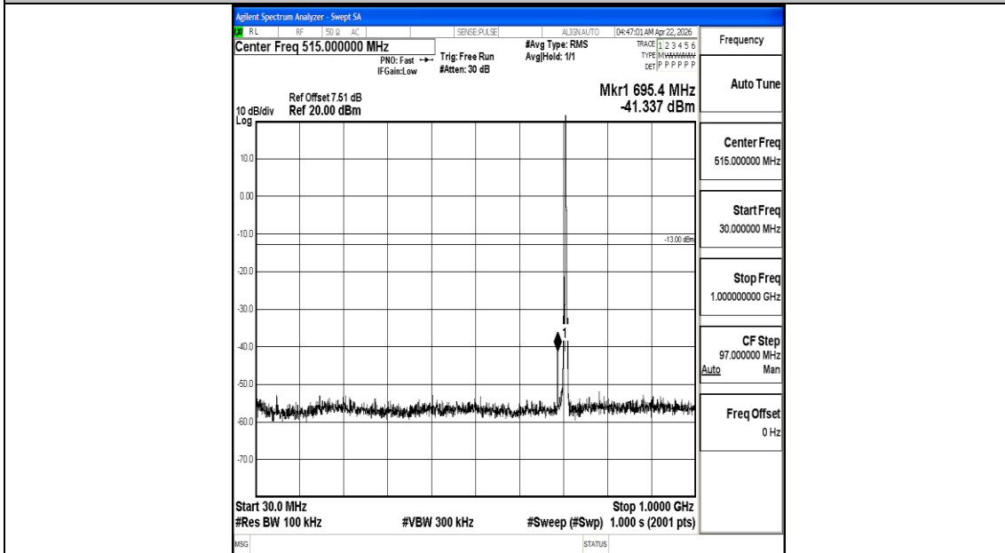
Band12_3MHz_16QAM_23165_1RB#0_30~1000_30~1000
