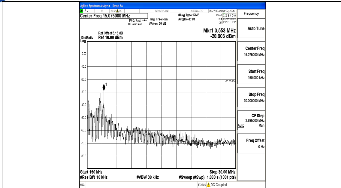
Band12_10MHz_16QAM_23095_1RB#0_0.15~30_0.15~30
