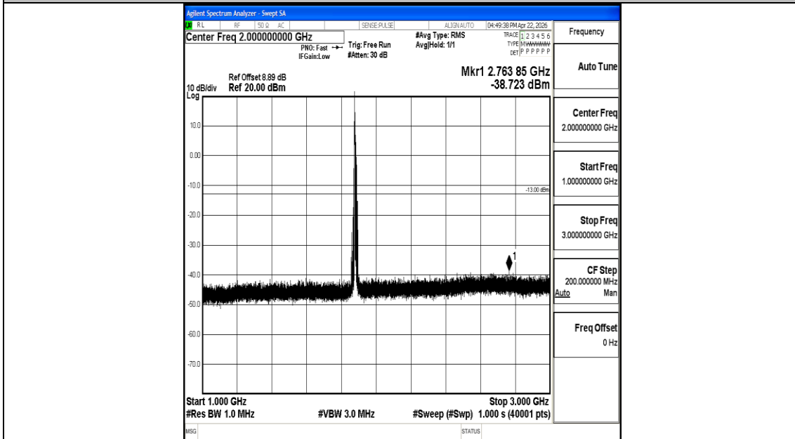
Band2_10MHz_16QAM_18900_1RB#0_1000~3000_1000~3000
