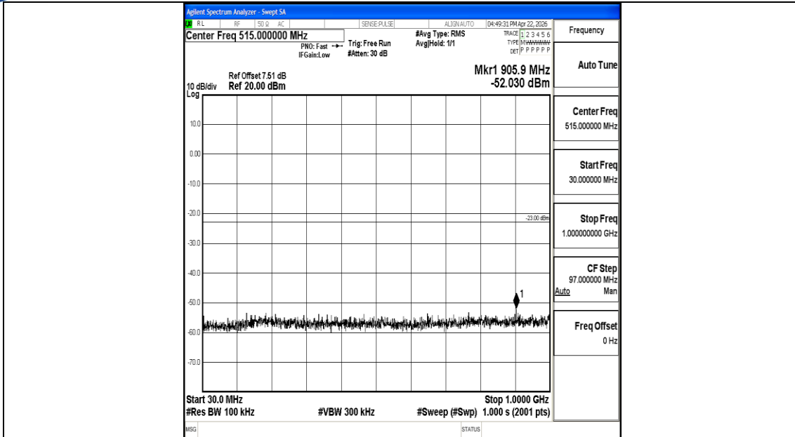
Band2_10MHz_16QAM_18900_1RB#0_30~1000_30~1000
