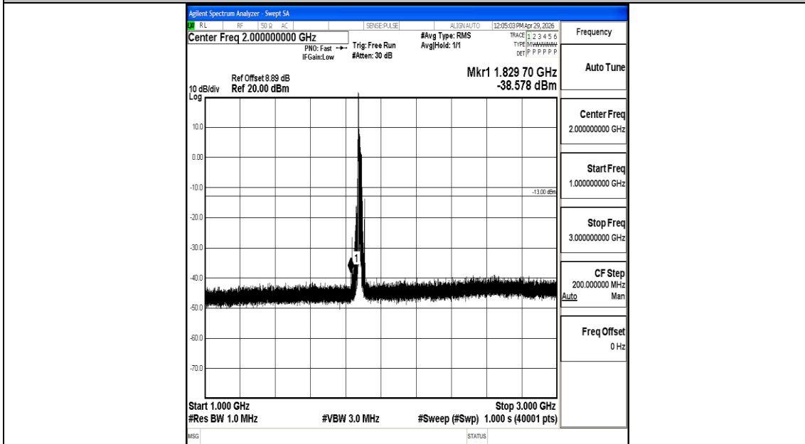
Band2_20MHz_16QAM_18900_1RB#0_1000~3000_1000~3000
