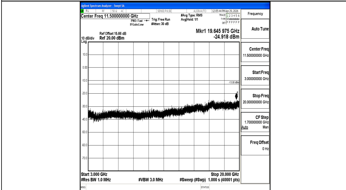
Band2_20MHz_QPSK_19100_1RB#0_3000~20000_3000~20000
