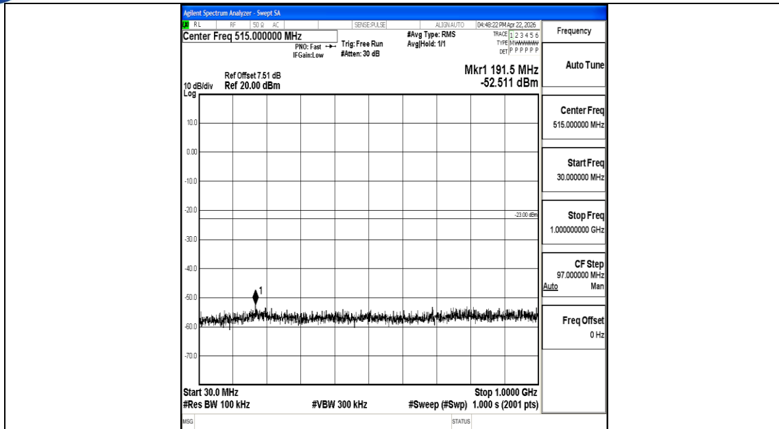
Band2_10MHz_16QAM_18650_1RB#0_30~1000_30~1000
