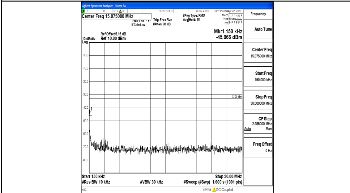
Band2_15MHz_16QAM_19125_1RB#0_0.15~30_0.15~30
