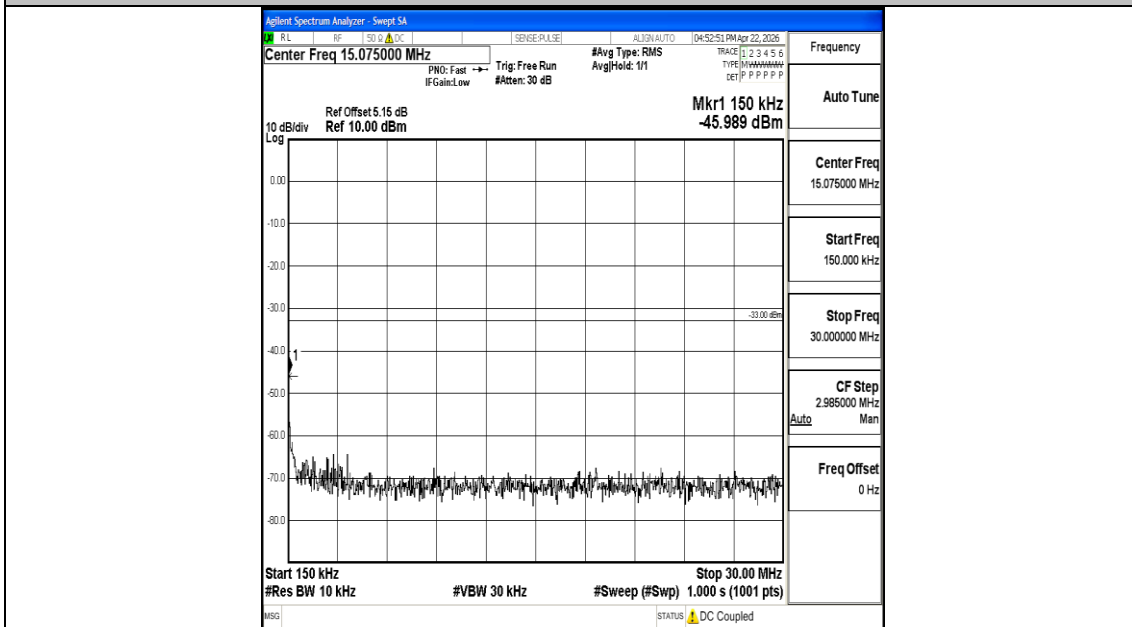
Band2_15MHz_16QAM_18900_1RB#0_0.15~30_0.15~30
