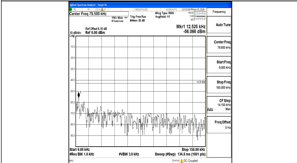
Band2_20MHz_QPSK_18700_1RB#0_0.009~0.15_0.009~0.15
