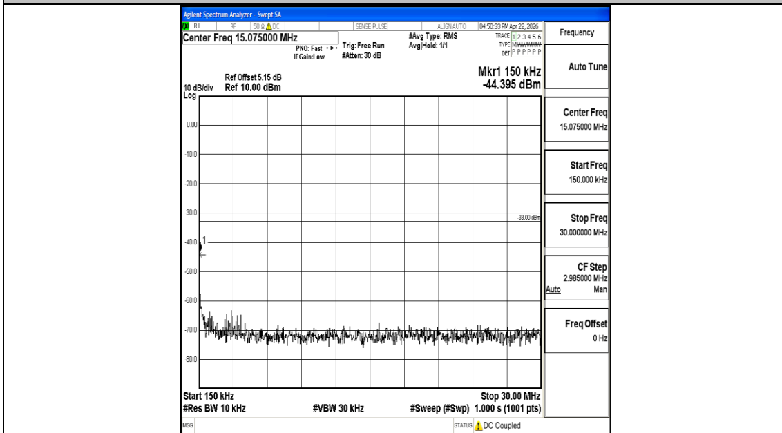
Band2_10MHz_16QAM_19150_1RB#0_0.15~30_0.15~30
