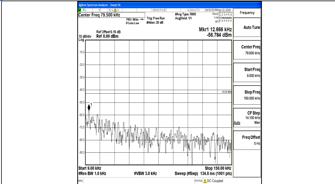
Band2_15MHz_16QAM_19125_1RB#0_0.009~0.15_0.009~0.15
