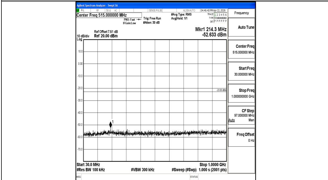
Band2_5MHz_QPSK_19175_1RB#0_30~1000_30~1000
