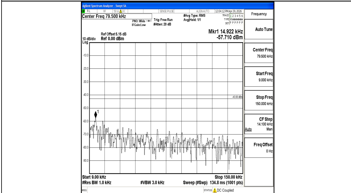
Band2_20MHz_QPSK_18900_1RB#0_0.009~0.15_0.009~0.15
