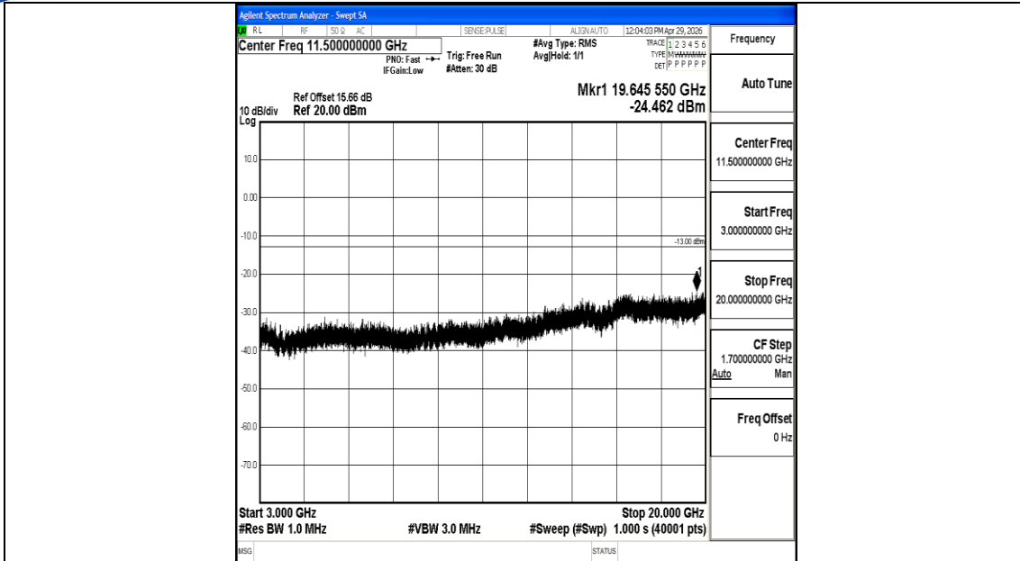
Band2_20MHz_16QAM_18700_1RB#0_3000~20000_3000~20000
