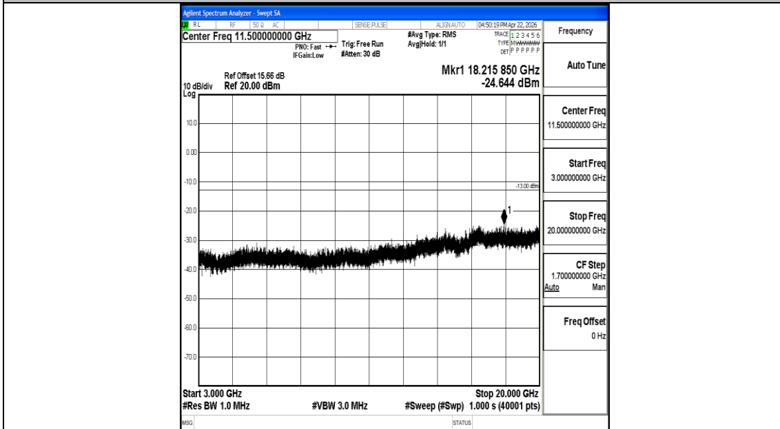
Band2_10MHz_QPSK_19150_1RB#0_3000~20000_3000~20000
