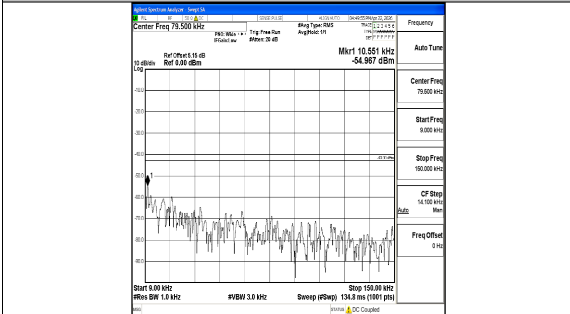
Band2_10MHz_QPSK_19150_1RB#0_0.009~0.15_0.009~0.15
