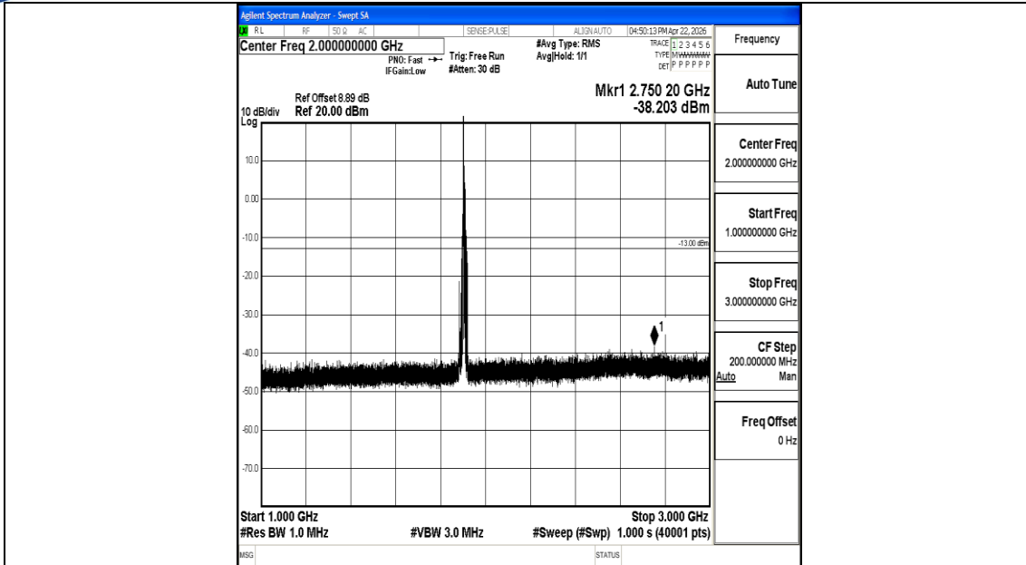
Band2_10MHz_QPSK_19150_1RB#0_1000~3000_1000~3000
