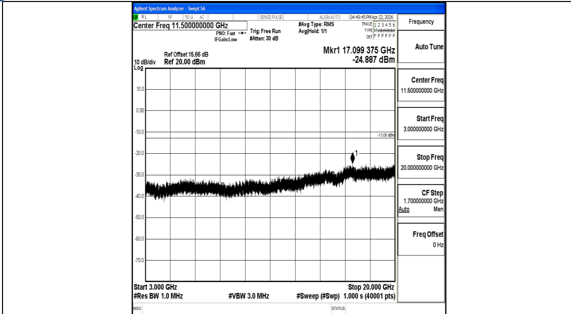
Band2_10MHz_16QAM_18900_1RB#0_3000~20000_3000~20000
