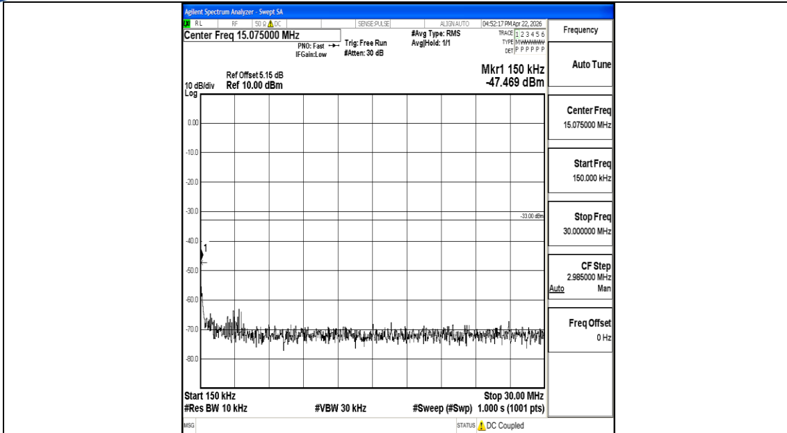
Band2_15MHz_QPSK_18900_1RB#0_0.15~30_0.15~30
