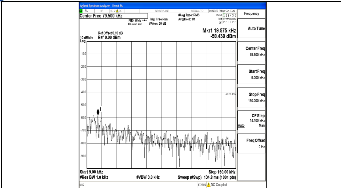
Band2_10MHz_16QAM_19150_1RB#0_0.009~0.15_0.009~0.15
