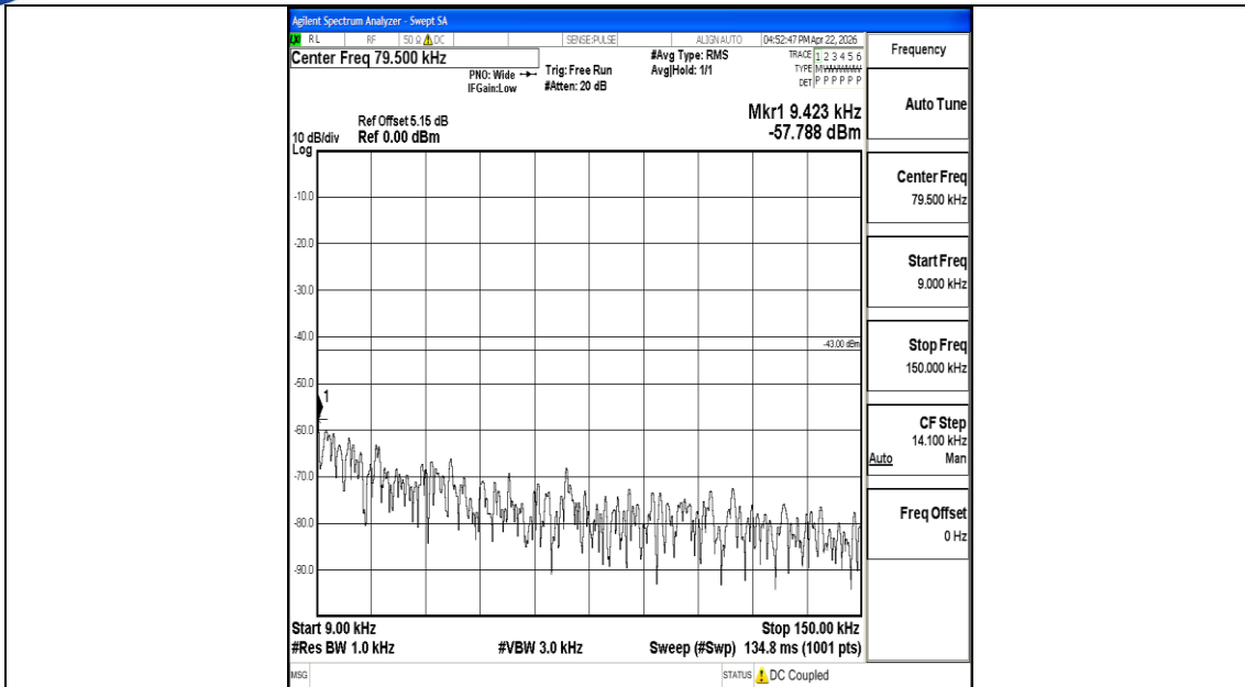
Band2_15MHz_16QAM_18900_1RB#0_0.009~0.15_0.009~0.15
