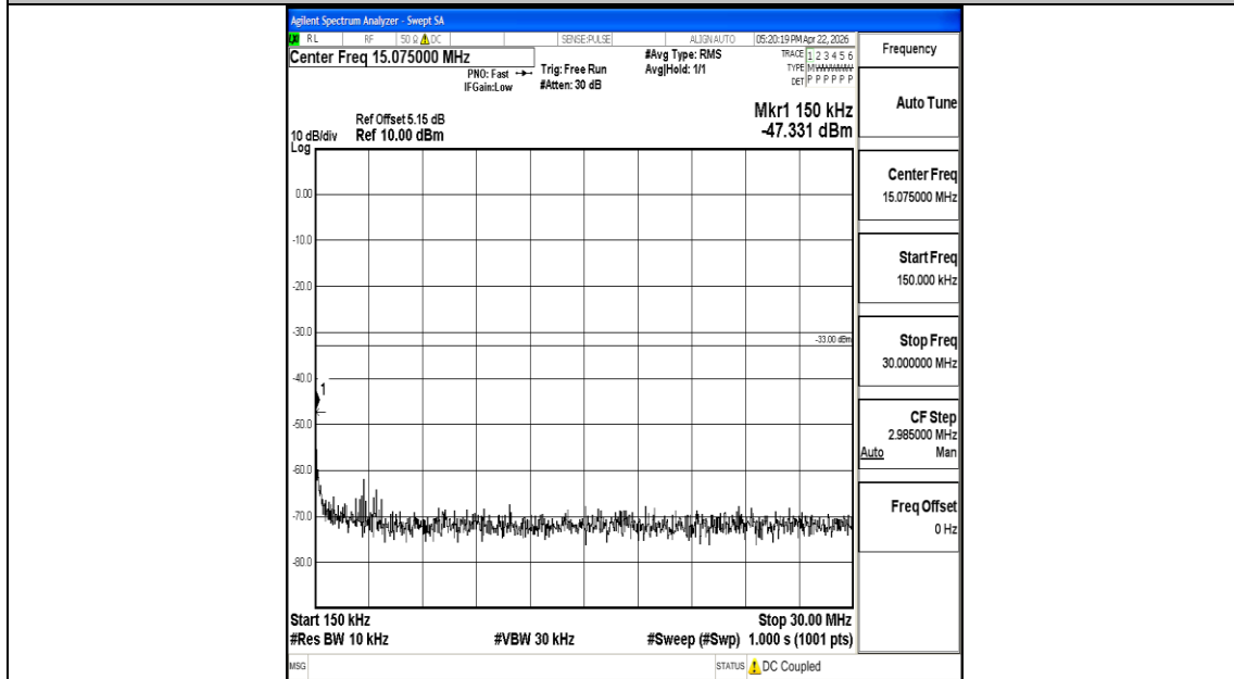
Band4_20MHz_16QAM_20050_1RB#0_0.15~30_0.15~30
