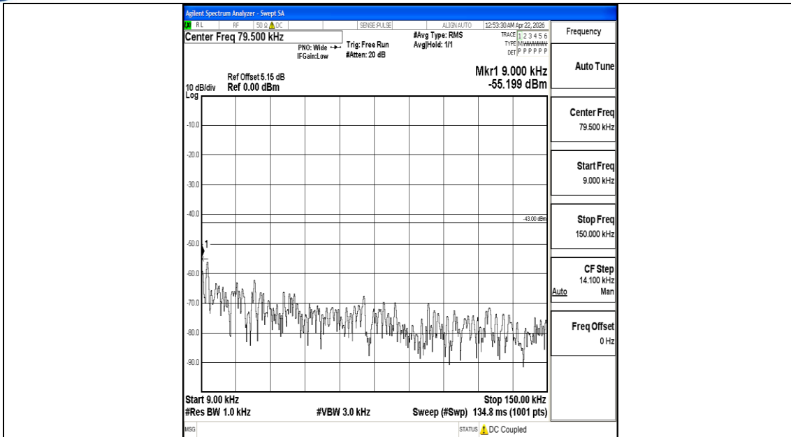
Band4_15MHz_16QAM_20025_1RB#0_0.009~0.15_0.009~0.15
