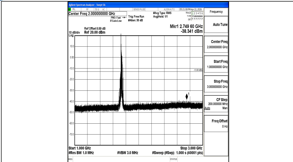
Band4_20MHz_QPSK_20175_1RB#0_1000~3000_1000~3000
