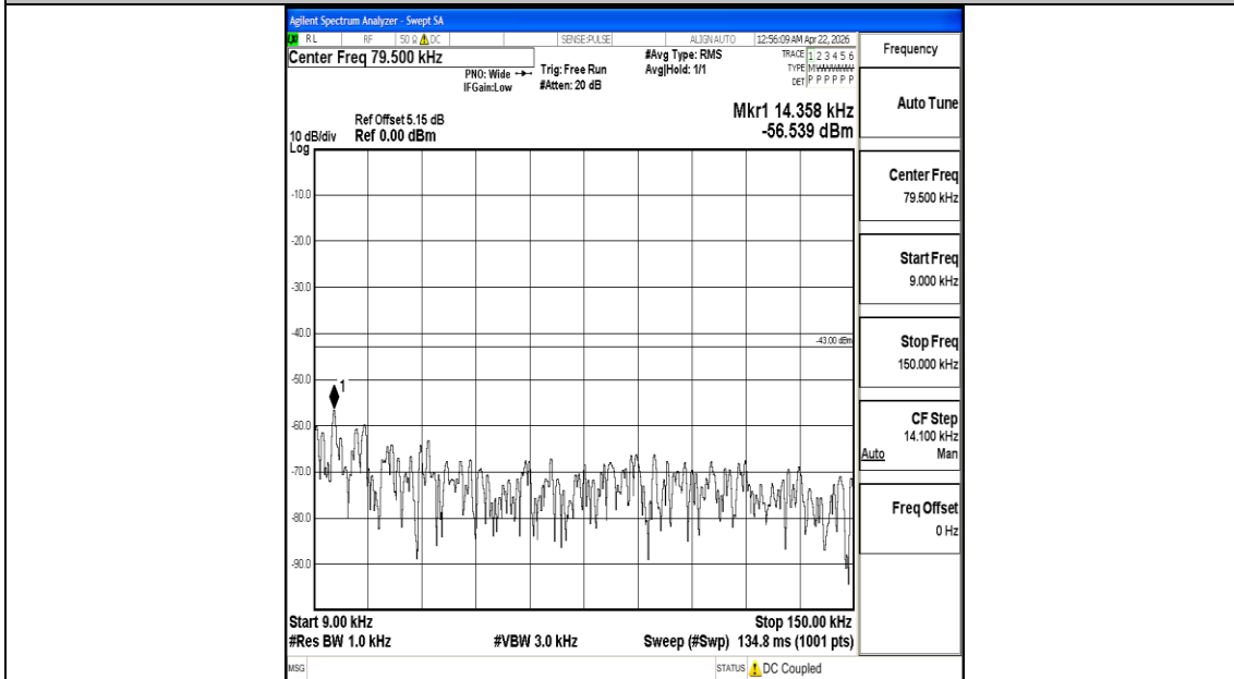
Band4_15MHz_QPSK_20175_1RB#0_0.009~0.15_0.009~0.15
