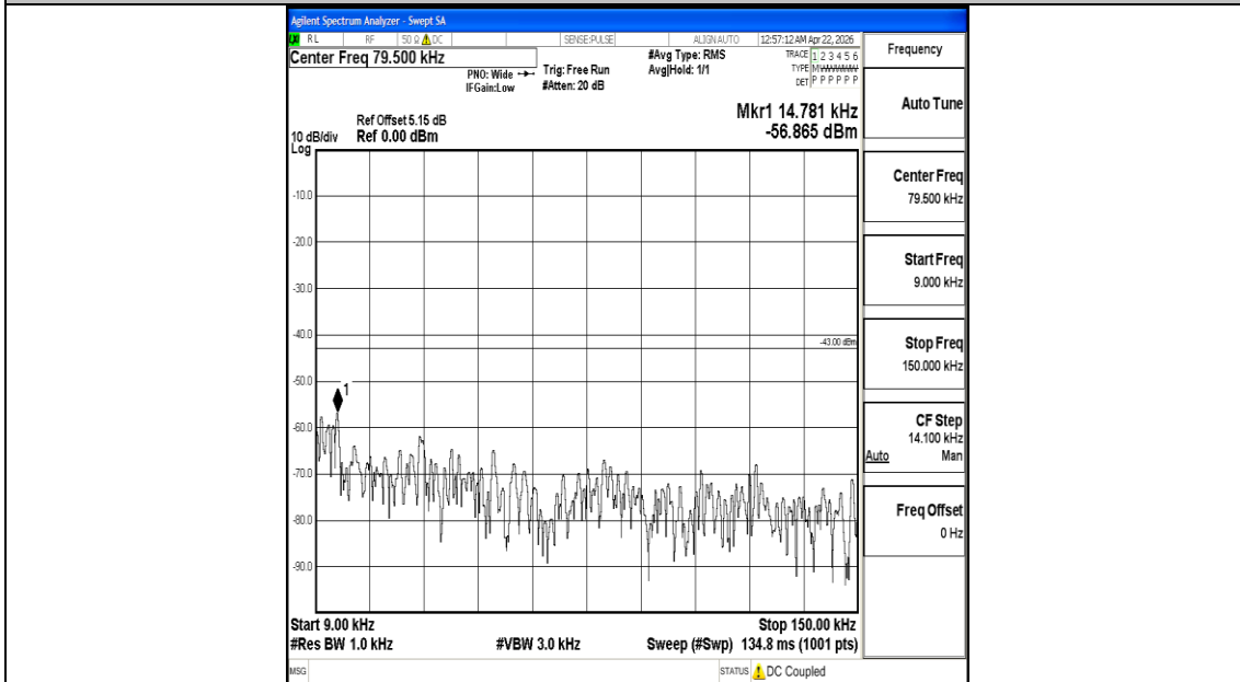
Band4_15MHz_QPSK_20325_1RB#0_0.009~0.15_0.009~0.15
