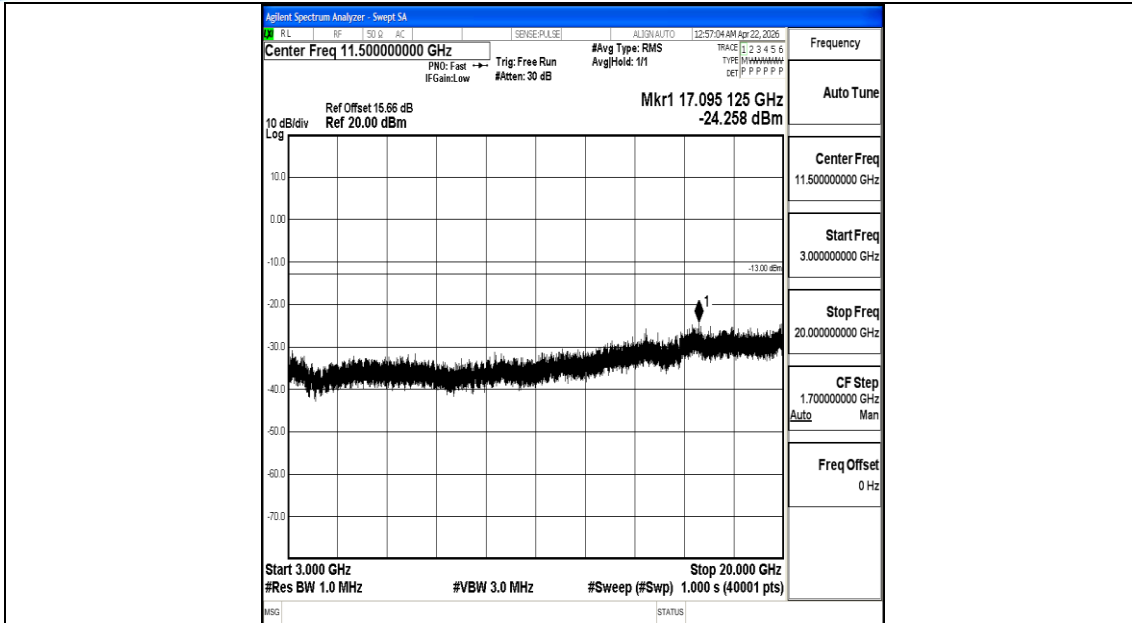
Band4_15MHz_16QAM_20175_1RB#0_3000~20000_3000~20000
