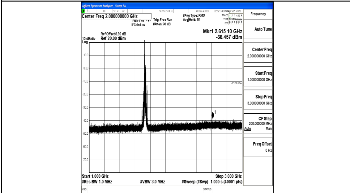
Band4_20MHz_16QAM_20175_1RB#0_1000~3000_1000~3000
