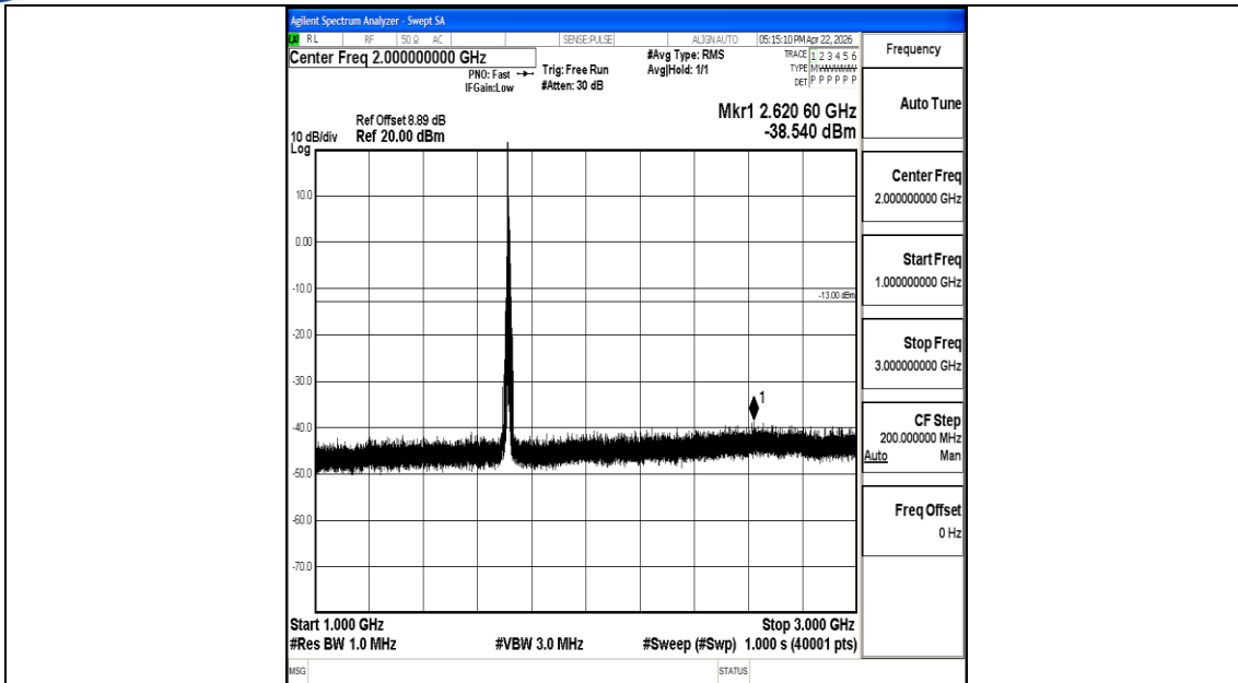
Band4_10MHz_QPSK_20000_1RB#0_1000~3000_1000~3000
