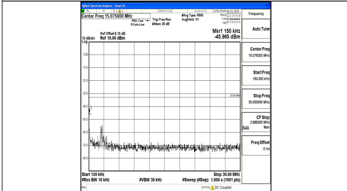
Band4_15MHz_16QAM_20175_1RB#0_0.15~30_0.15~30
