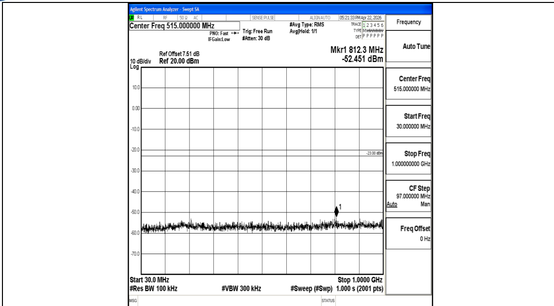
Band4_20MHz_16QAM_20175_1RB#0_30~1000_30~1000
