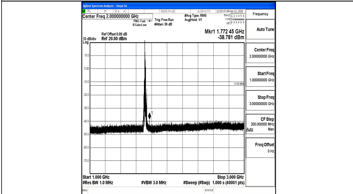
Band4_15MHz_16QAM_20025_1RB#0_1000~3000_1000~3000
