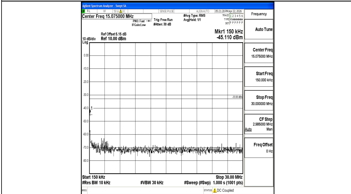
Band4_20MHz_16QAM_20175_1RB#0_0.15~30_0.15~30
