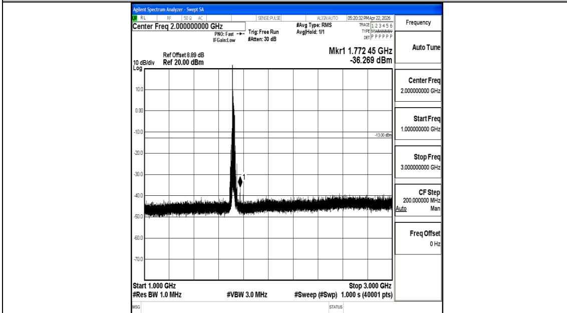
Band4_20MHz_16QAM_20050_1RB#0_1000~3000_1000~3000
