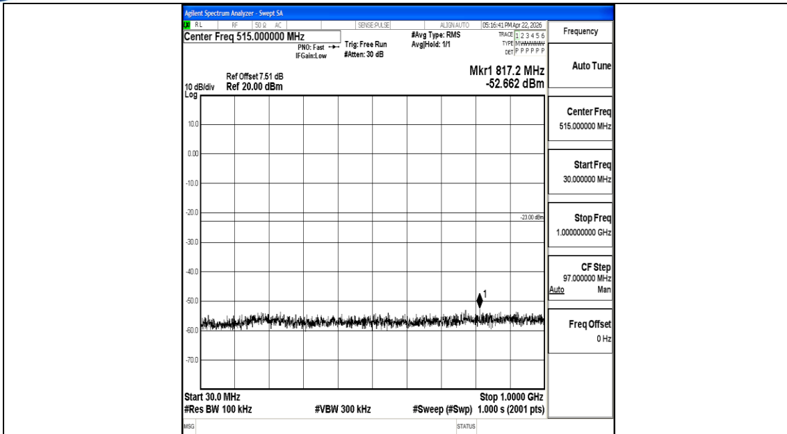
Band4_10MHz_16QAM_20175_1RB#0_30~1000_30~1000
