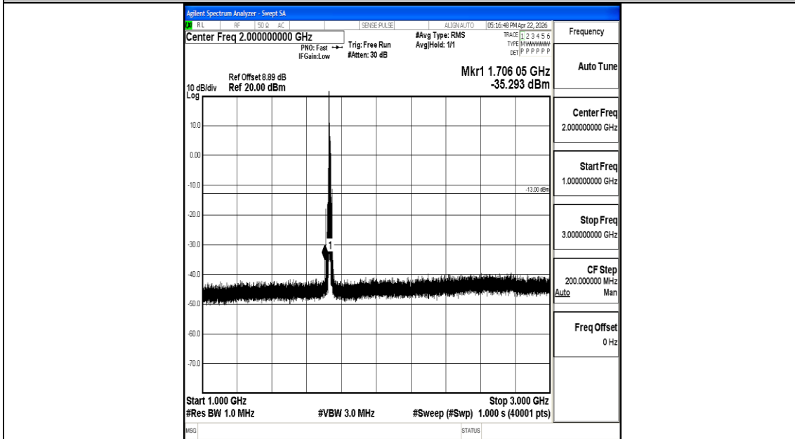
Band4_10MHz_16QAM_20175_1RB#0_1000~3000_1000~3000
