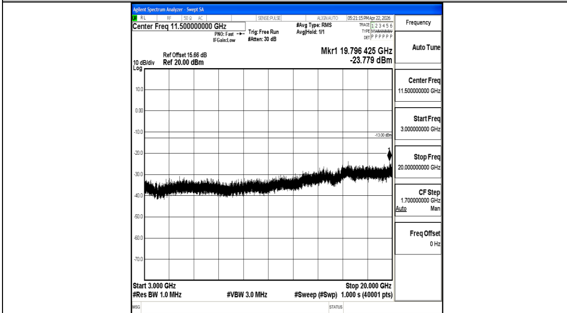
Band4_20MHz_QPSK_20175_1RB#0_3000~20000_3000~20000
