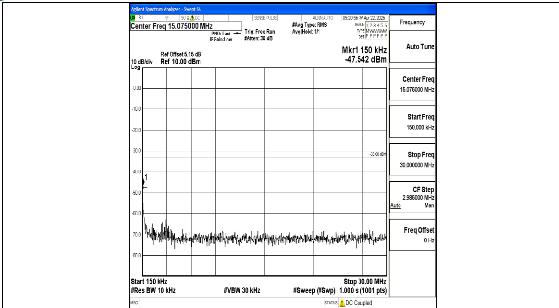
Band4_20MHz_QPSK_20175_1RB#0_0.15~30_0.15~30
