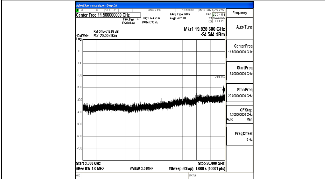
Band4_10MHz_QPSK_20000_1RB#0_3000~20000_3000~20000
