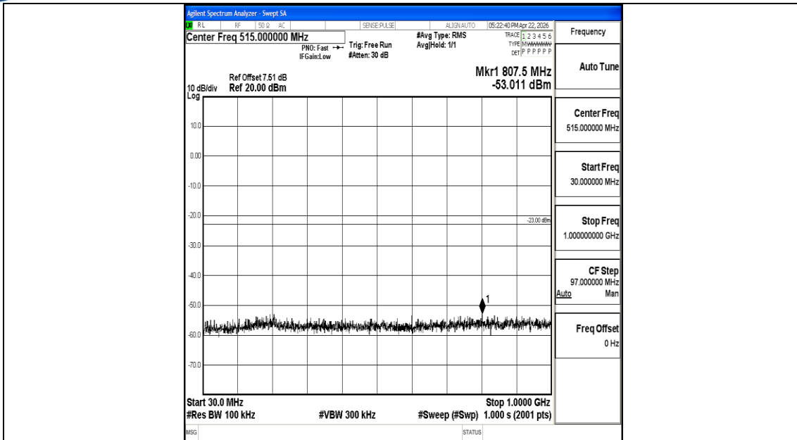
Band4_20MHz_16QAM_20300_1RB#0_30~1000_30~1000
