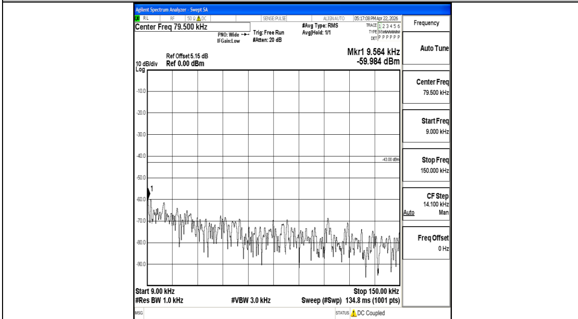
Band4_10MHz_QPSK_20350_1RB#0_0.009~0.15_0.009~0.15
