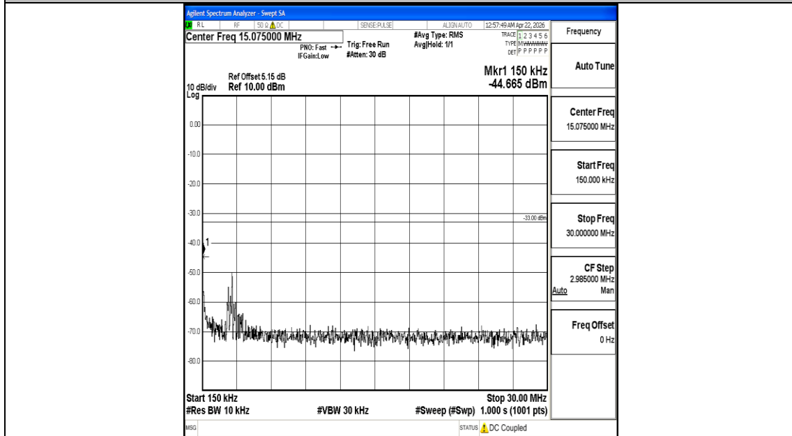
Band4_15MHz_16QAM_20325_1RB#0_0.15~30_0.15~30
