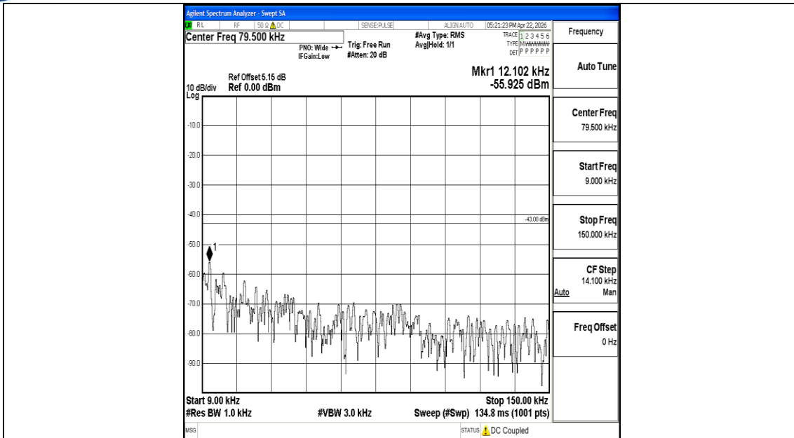
Band4_20MHz_16QAM_20175_1RB#0_0.009~0.15_0.009~0.15
