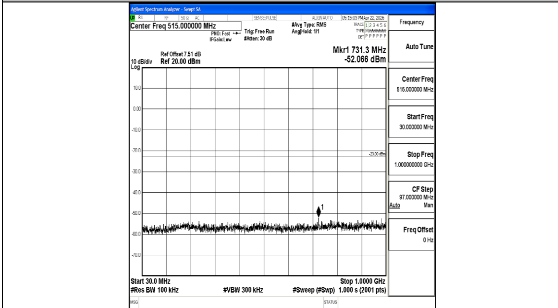
Band4_10MHz_QPSK_20000_1RB#0_30~1000_30~1000
