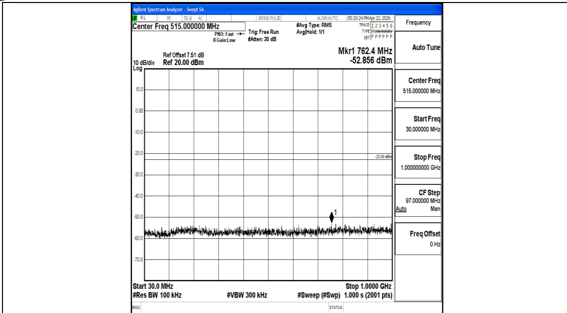
Band4_20MHz_16QAM_20050_1RB#0_30~1000_30~1000
