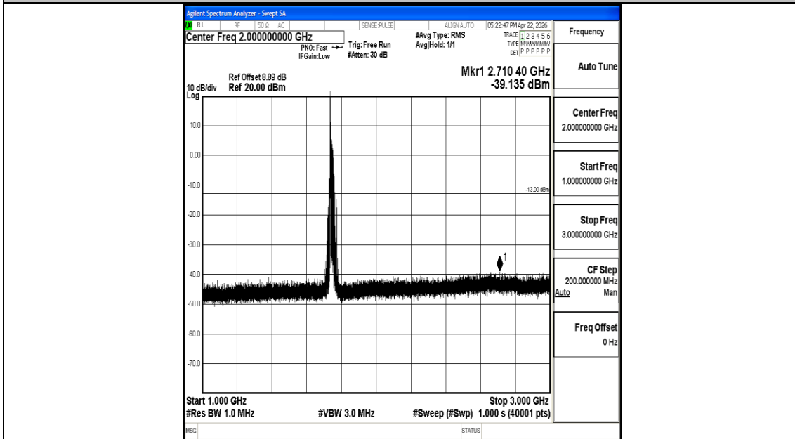
Band4_20MHz_16QAM_20300_1RB#0_1000~3000_1000~3000
