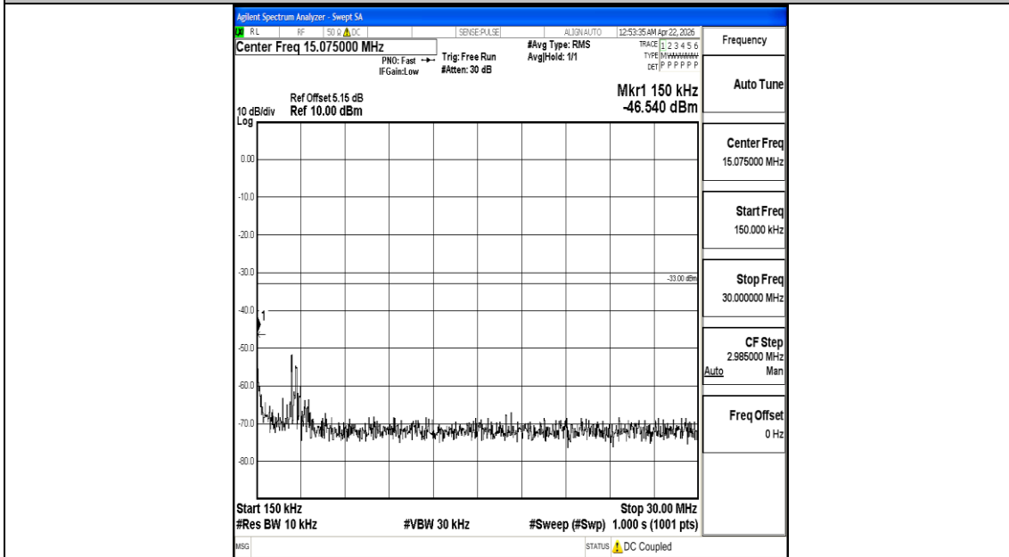
Band4_15MHz_16QAM_20025_1RB#0_0.15~30_0.15~30
