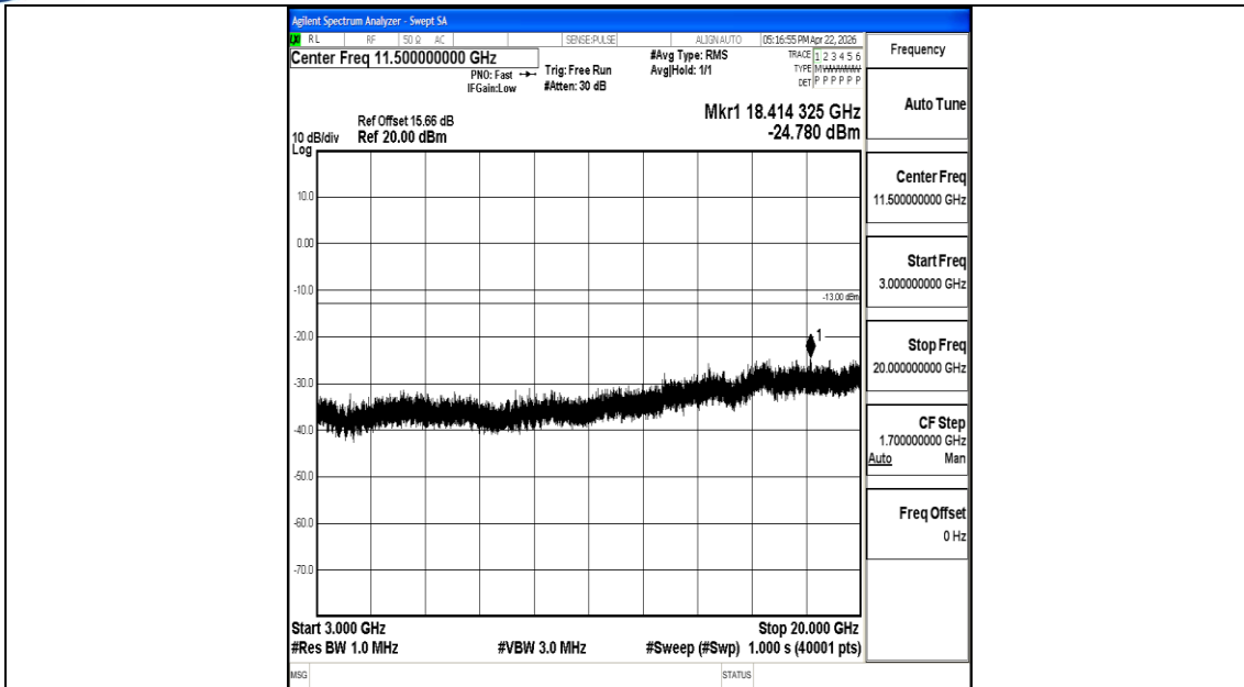
Band4_10MHz_16QAM_20175_1RB#0_3000~20000_3000~20000
