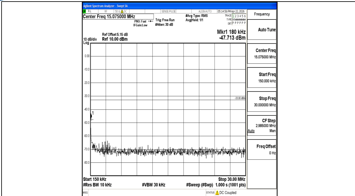
Band4_10MHz_QPSK_20000_1RB#0_0.15~30_0.15~30
