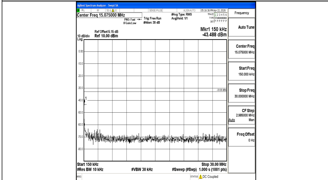
Band4_10MHz_16QAM_20175_1RB#0_0.15~30_0.15~30
