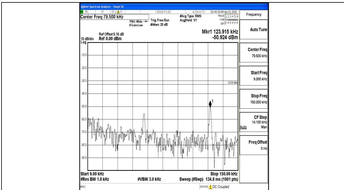
Band5_10MHz_QPSK_20450_1RB#0_0.009~0.15_0.009~0.15
