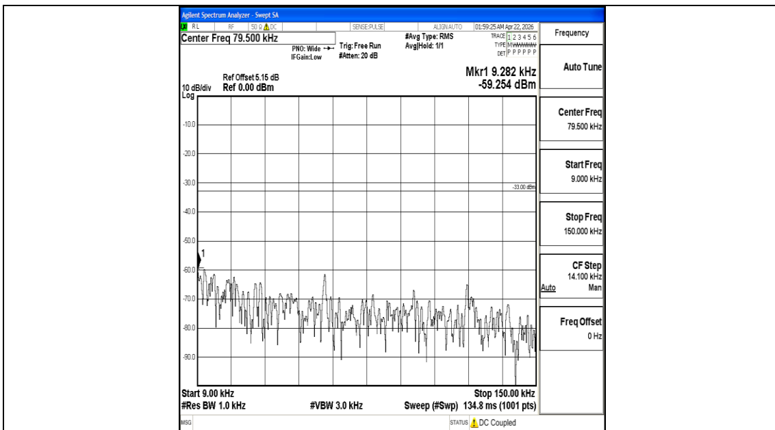
Band5_3MHz_QPSK_20415_1RB#0_0.009~0.15_0.009~0.15
