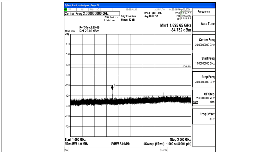
Band5_1.4MHz_16QAM_20643_1RB#0_1000~3000_1000~3000
