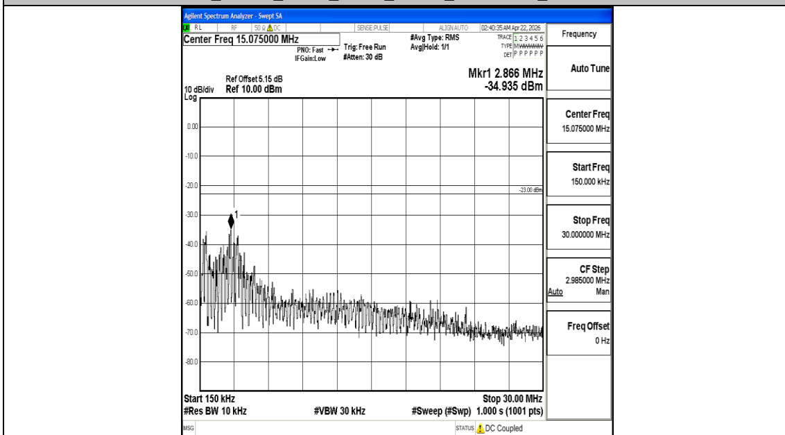
Band5_10MHz_QPSK_20450_1RB#0_0.15~30_0.15~30
