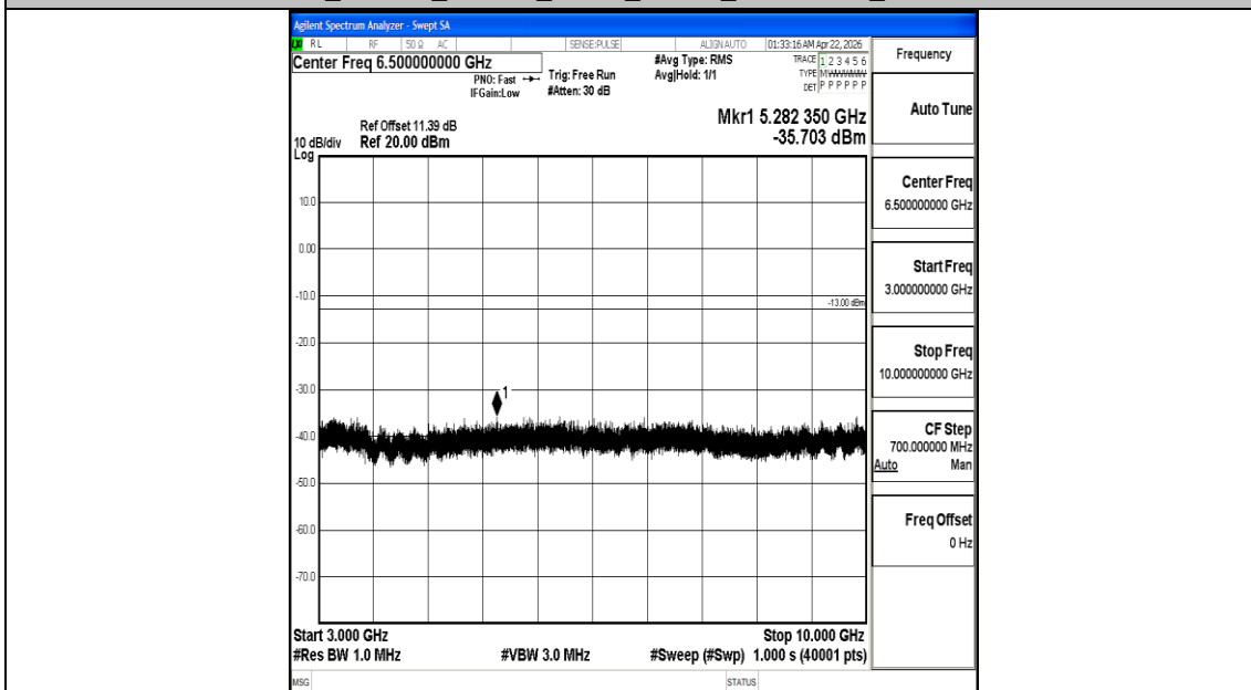
Band5_1.4MHz_16QAM_20643_1RB#0_3000~10000_3000~10000
