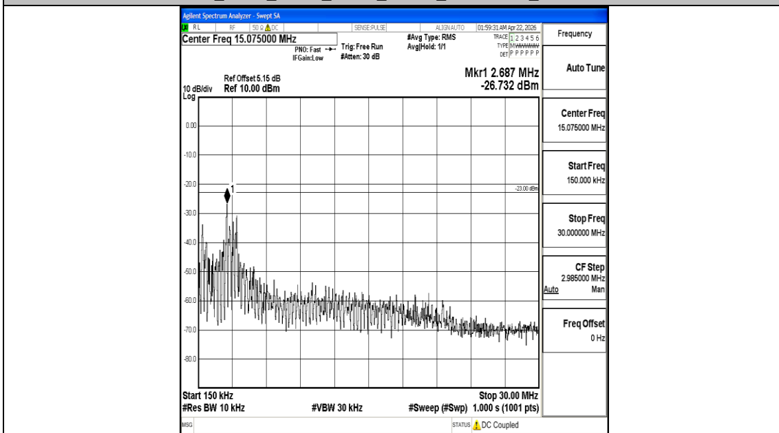
Band5_3MHz_QPSK_20415_1RB#0_0.15~30_0.15~30
