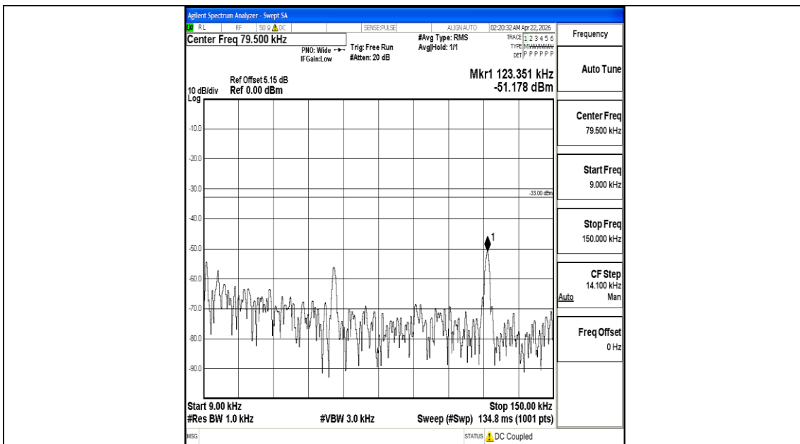
Band5_5MHz_QPSK_20425_1RB#0_0.009~0.15_0.009~0.15
