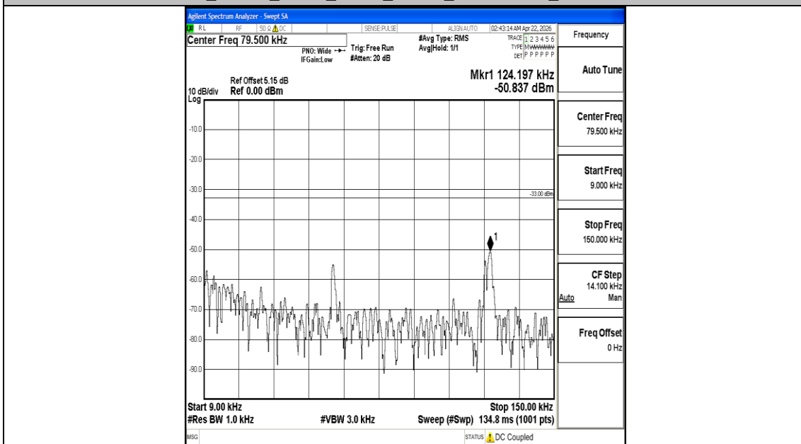
Band5_10MHz_16QAM_20600_1RB#0_0.009~0.15_0.009~0.15
