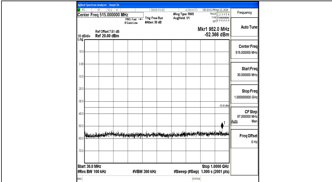
Band7_10MHz_QPSK_21400_1RB#0_30~1000_30~1000
