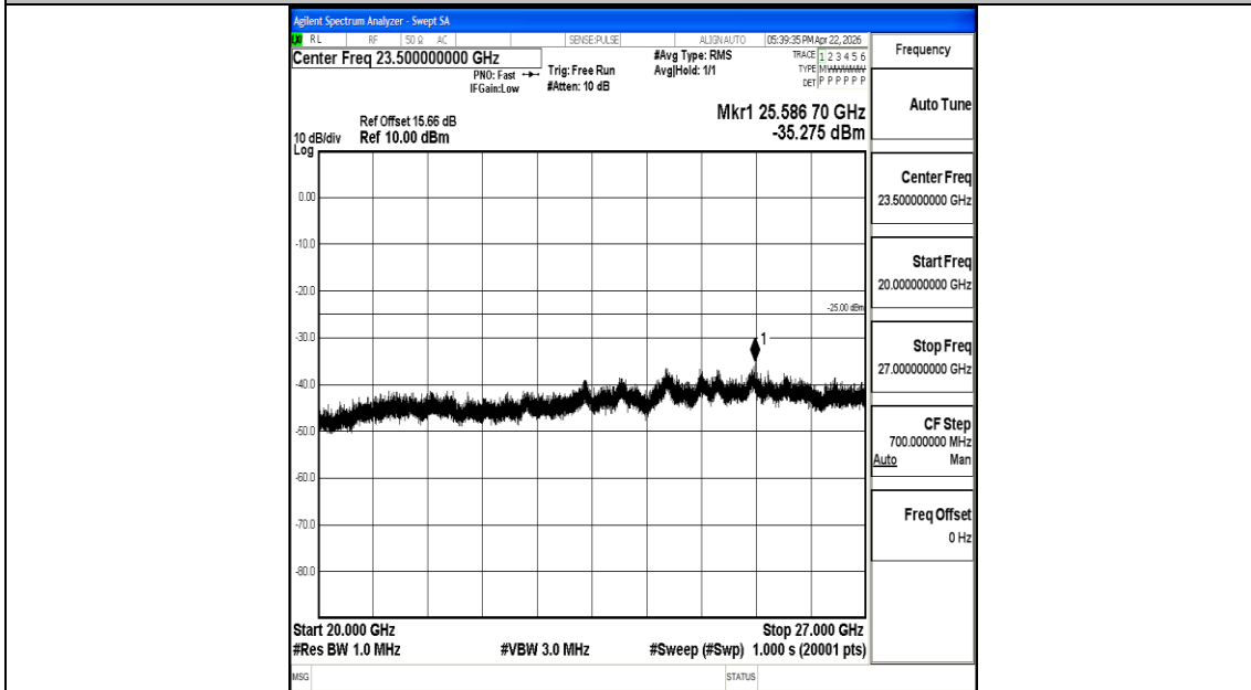
Band7_20MHz_16QAM_21350_1RB#0_20000~27000_20000~27000
