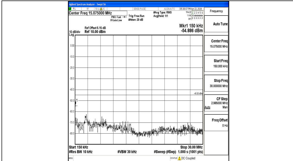
Band7_20MHz_16QAM_21100_1RB#0_0.15~30_0.15~30
