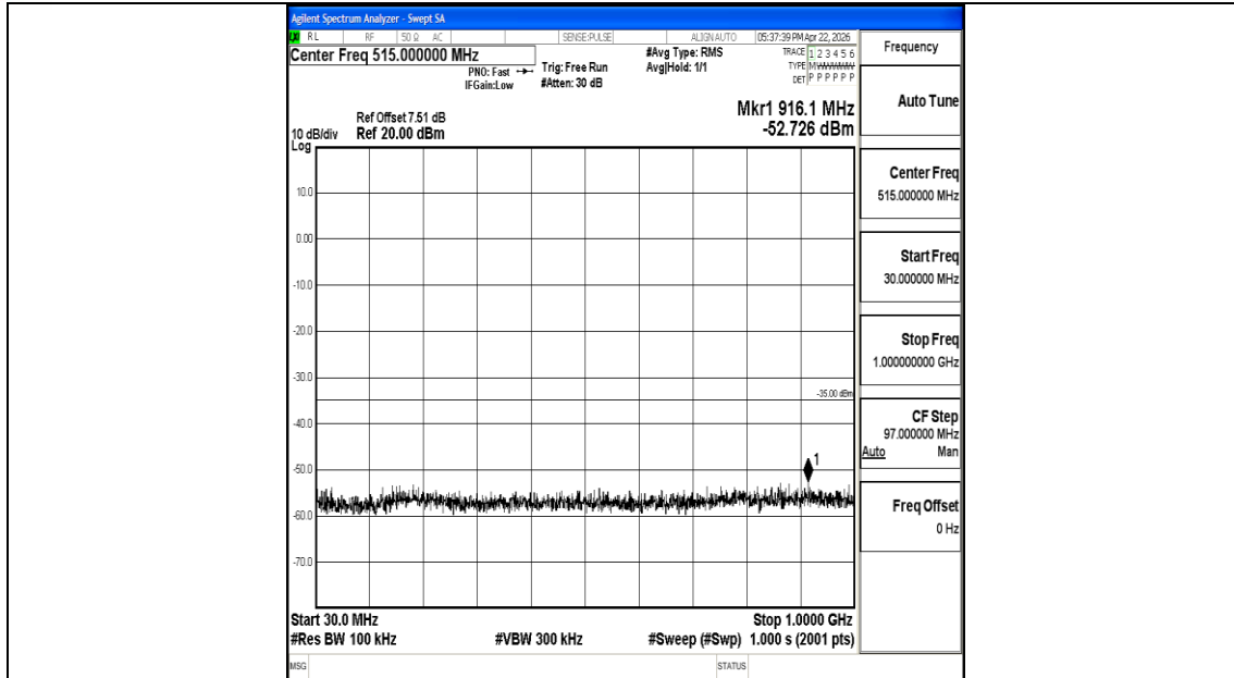
Band7_20MHz_QPSK_21100_1RB#0_30~1000_30~1000
