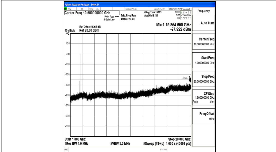
Band7_15MHz_QPSK_21100_1RB#0_1000~20000_1000~20000
