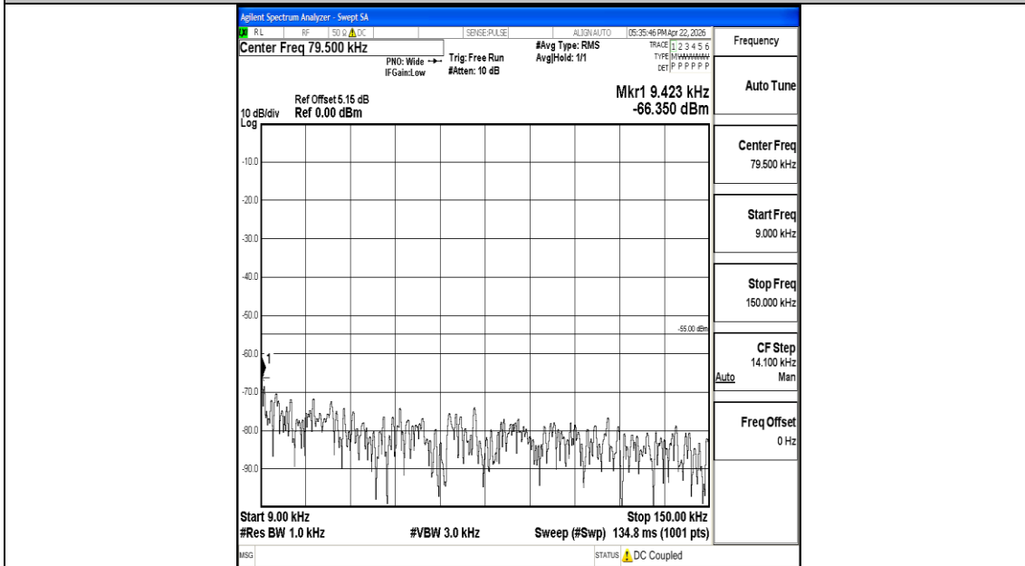
Band7_15MHz_16QAM_21375_1RB#0_0.009~0.15_0.009~0.15
