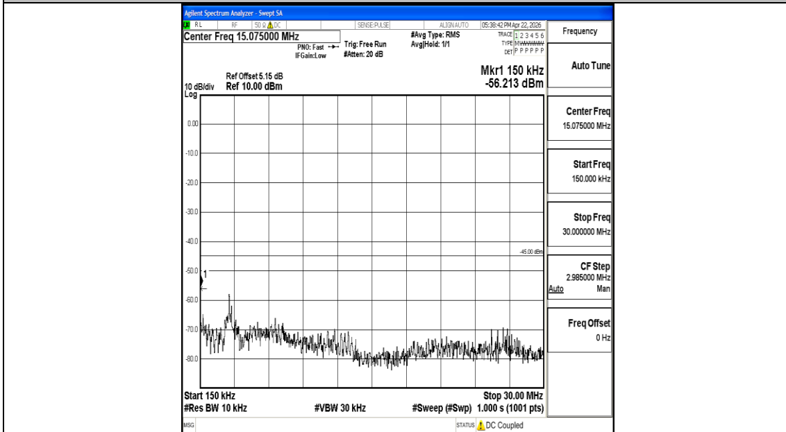
Band7_20MHz_QPSK_21350_1RB#0_0.15~30_0.15~30
