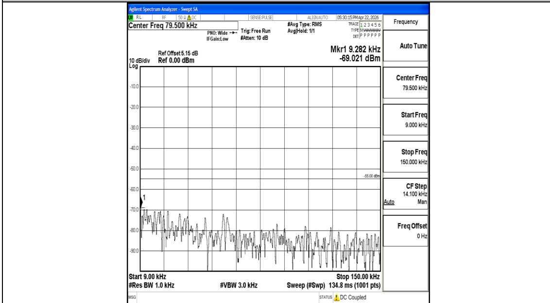
Band7_10MHz_16QAM_20800_1RB#0_0.009~0.15_0.009~0.15
