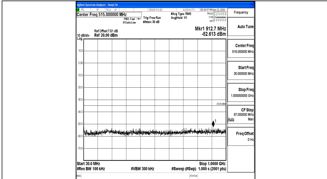
Band7_10MHz_QPSK_21100_1RB#0_30~1000_30~1000
