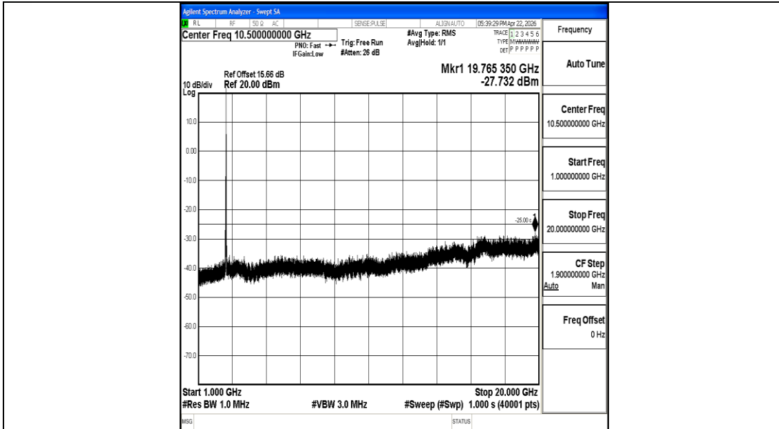
Band7_20MHz_16QAM_21350_1RB#0_1000~20000_1000~20000
