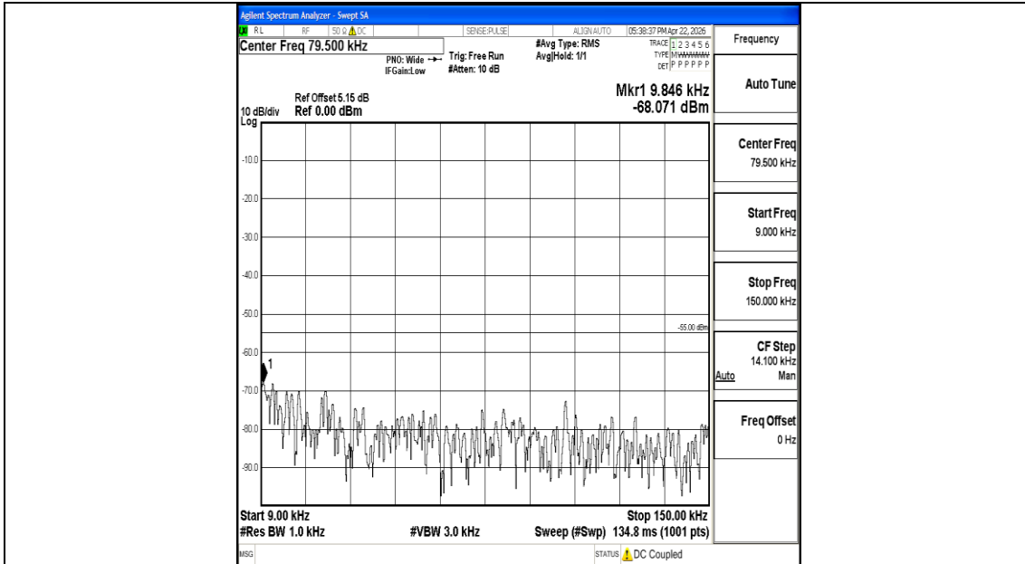
Band7_20MHz_QPSK_21350_1RB#0_0.009~0.15_0.009~0.15
