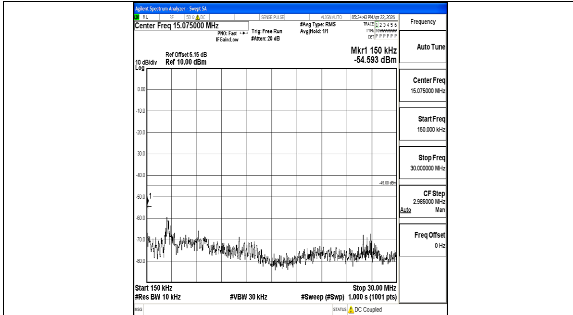
Band7_15MHz_16QAM_21100_1RB#0_0.15~30_0.15~30
