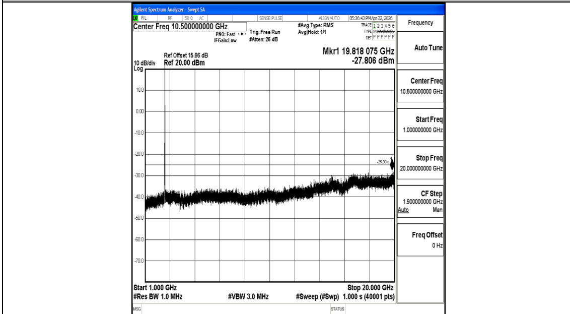
Band7_20MHz_QPSK_20850_1RB#0_1000~20000_1000~20000
