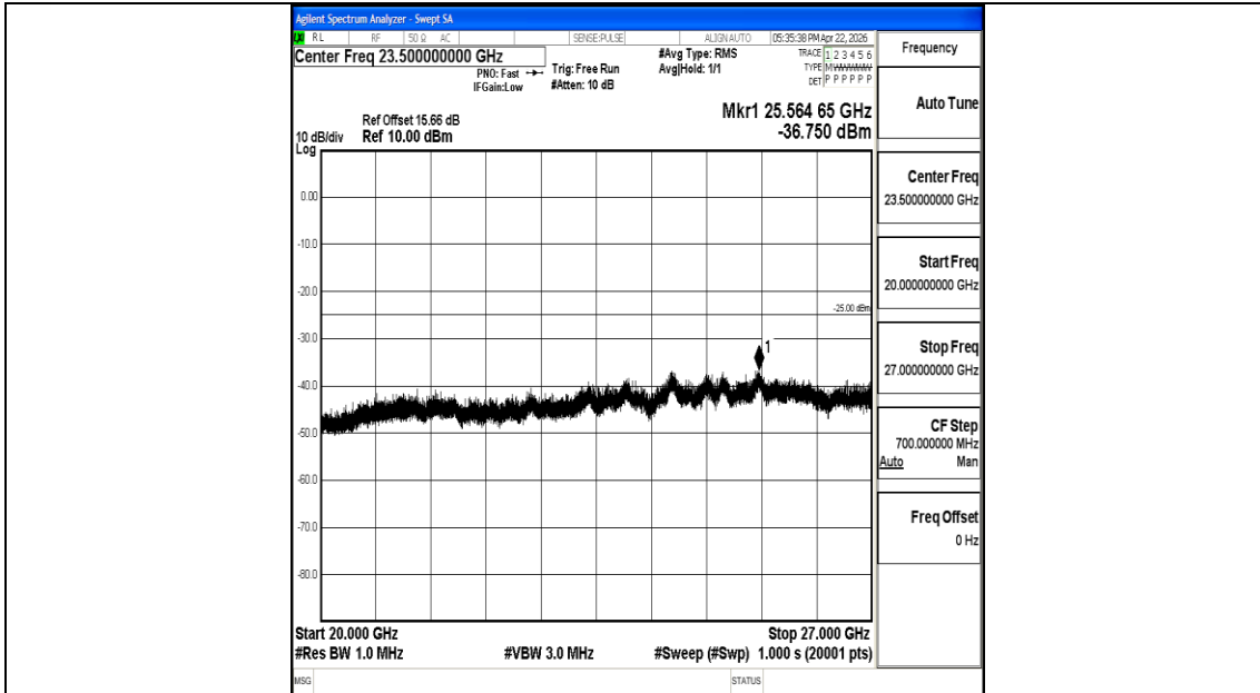
Band7_15MHz_QPSK_21375_1RB#0_20000~27000_20000~27000
