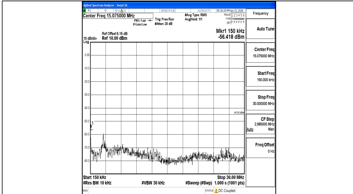
Band7_10MHz_16QAM_20800_1RB#0_0.15~30_0.15~30
