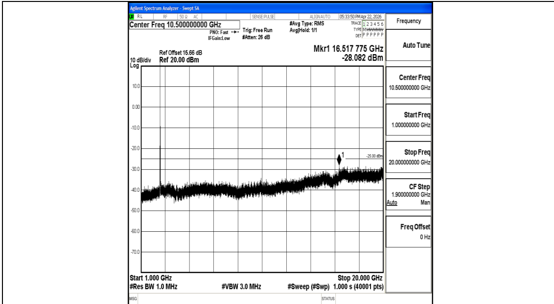
Band7_15MHz_16QAM_20825_1RB#0_1000~20000_1000~20000
