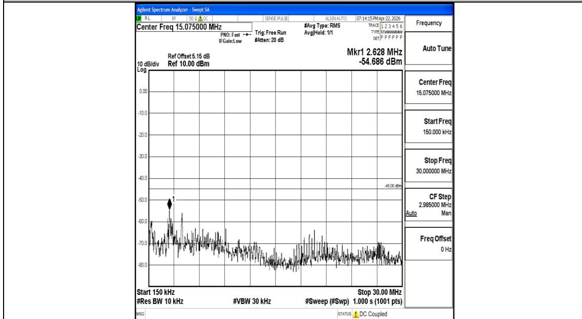
Band7_5MHz_16QAM_21425_1RB#0_0.15~30_0.15~30
