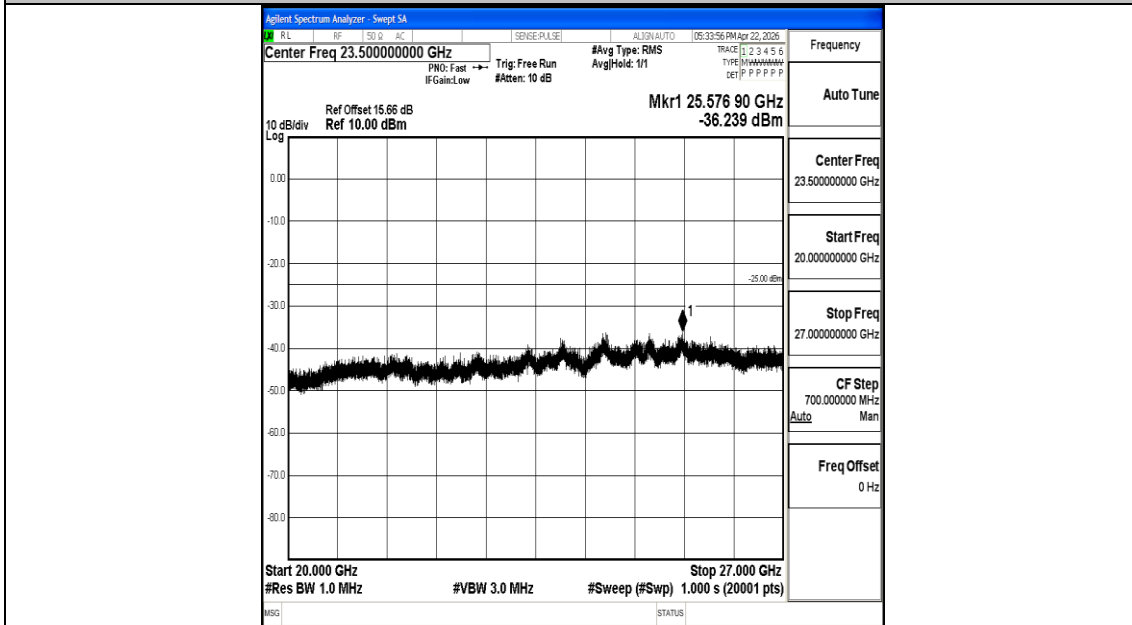
Band7_15MHz_16QAM_20825_1RB#0_20000~27000_20000~27000
