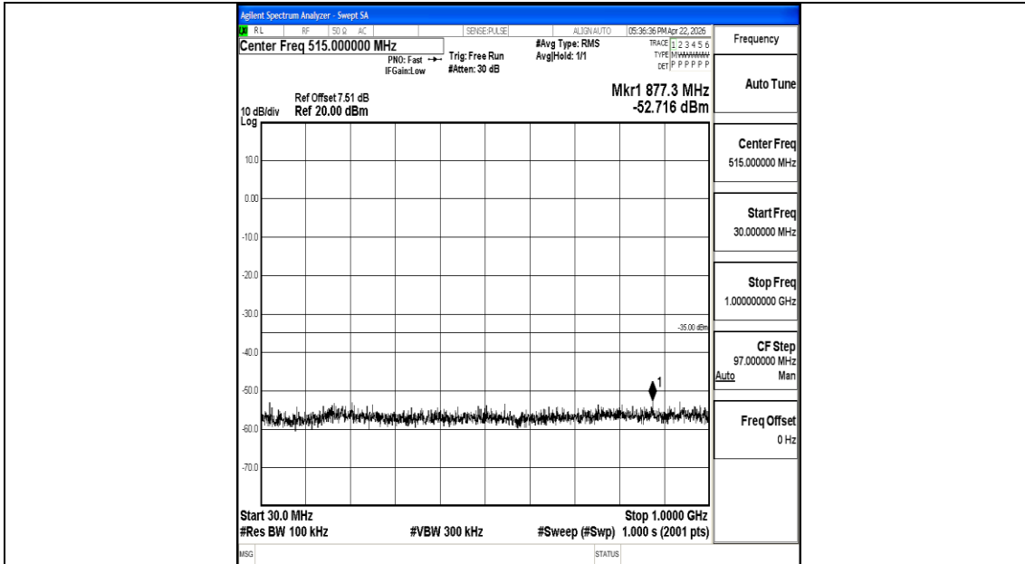
Band7_20MHz_QPSK_20850_1RB#0_30~1000_30~1000
