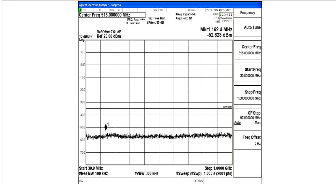
Band7_15MHz_QPSK_20825_1RB#0_30~1000_30~1000
