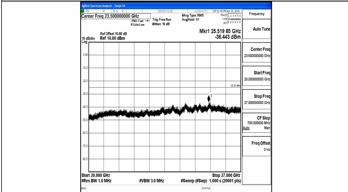
Band7_10MHz_16QAM_21100_1RB#0_20000~27000_20000~27000
