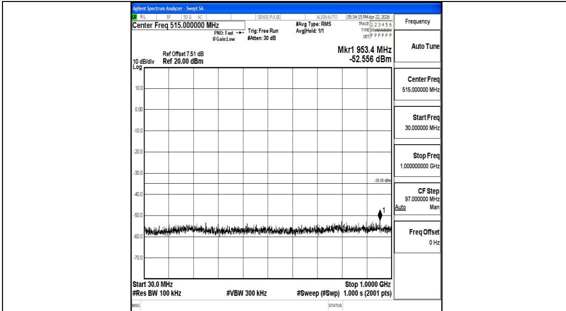
Band7_15MHz_QPSK_21100_1RB#0_30~1000_30~1000
