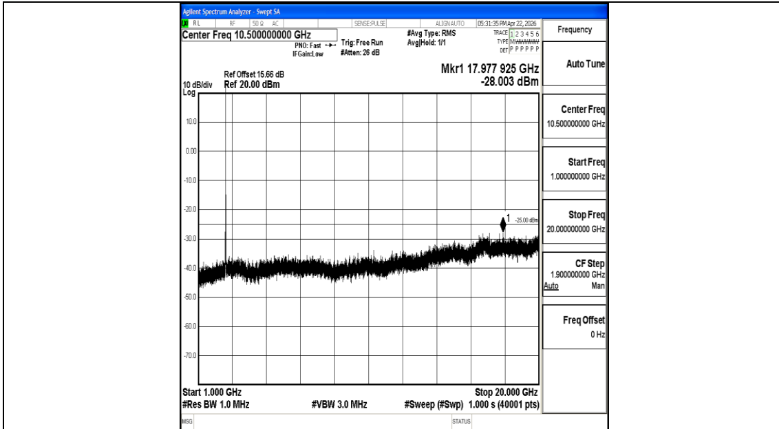
Band7_10MHz_16QAM_21100_1RB#0_1000~20000_1000~20000
