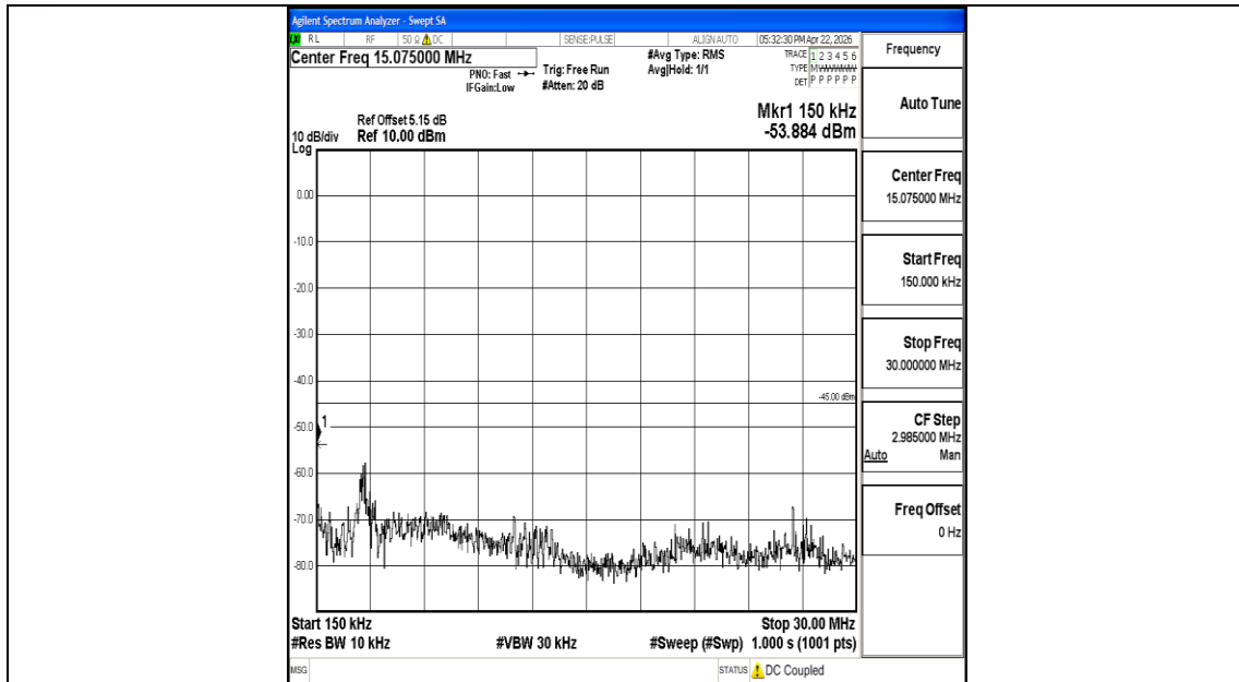
Band7_10MHz_16QAM_21400_1RB#0_0.15~30_0.15~30
