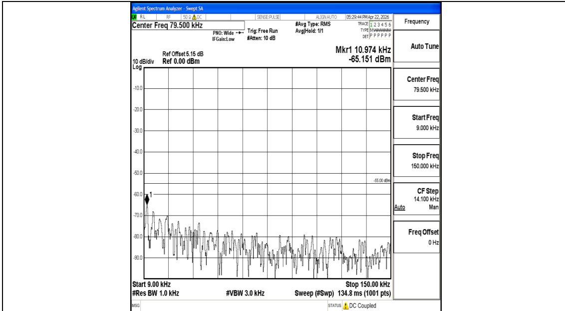
Band7_10MHz_QPSK_20800_1RB#0_0.009~0.15_0.009~0.15
