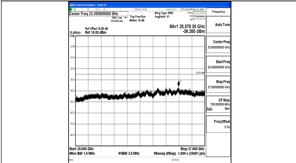
Band7_5MHz_QPSK_21425_1RB#0_20000~27000_20000~27000
