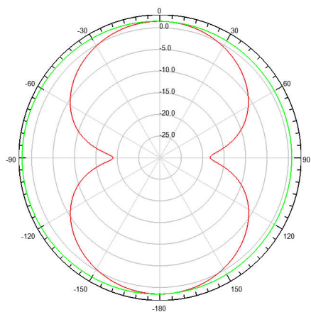
2D 增益模式 2D Gain Pattern (2450 MHz)
