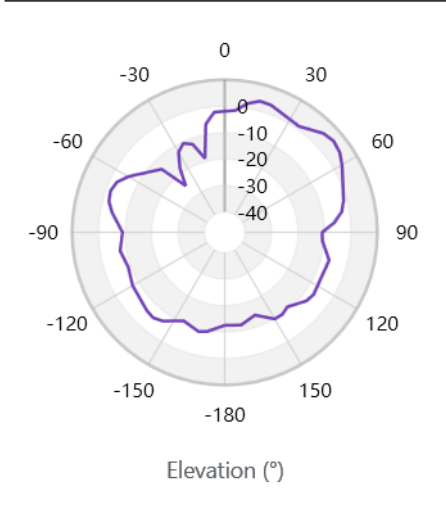
[Gain] Elevation cut (ElectricField)
