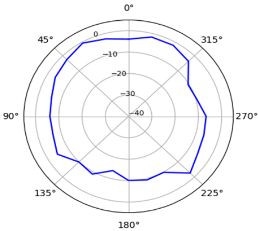
XY-Plane 2500 MHz
