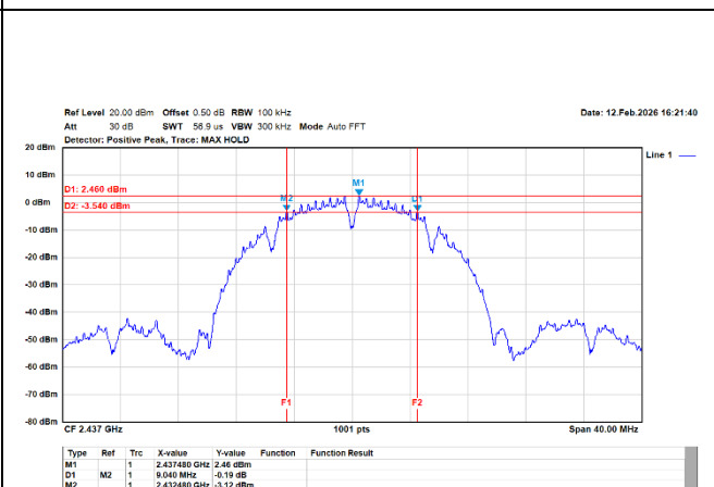
802.11b/20MHz/1M/2437MHz/Ch6/Ant.1
