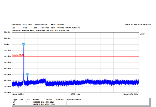
802.11g/20MHz/6M/2437MHz/Ch6/Ant.1
