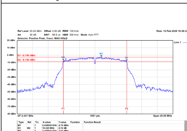
802.11g/20MHz/6M/2437MHz/Ch6/Ant.1
