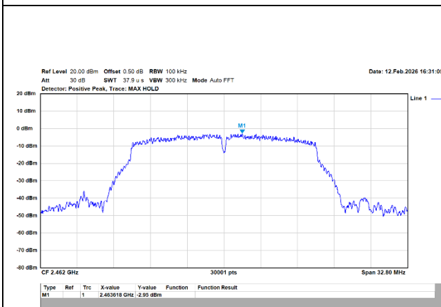
802.11g/20MHz/6M/2462MHz/Ch11/Ant.1 (Ref.)
