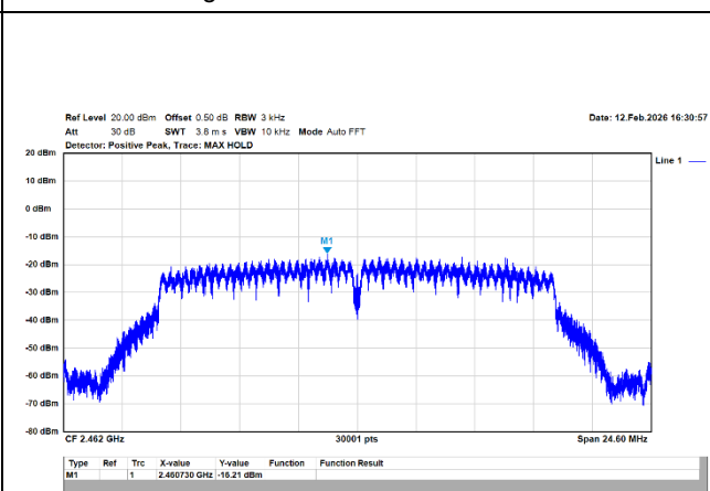
802.11g/20MHz/6M/2462MHz/Ch11/Ant.1
