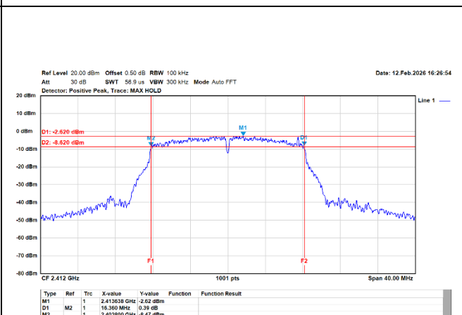
802.11g/20MHz/6M/2412MHz/Ch1/Ant.1
