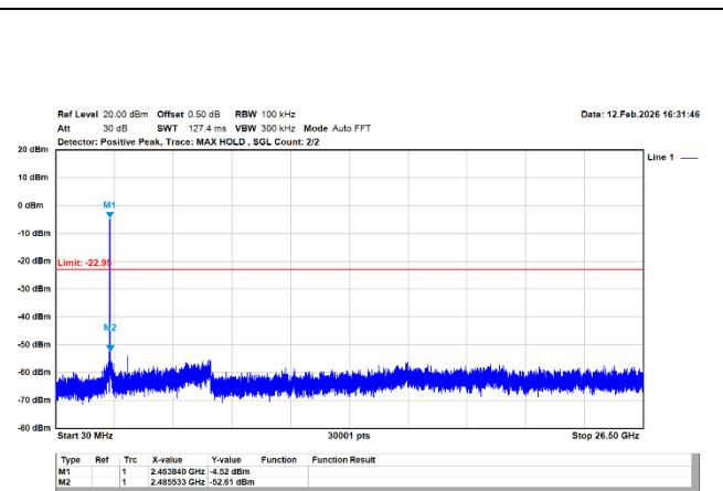
802.11g/20MHz/6M/2462MHz/Ch11/Ant.1
