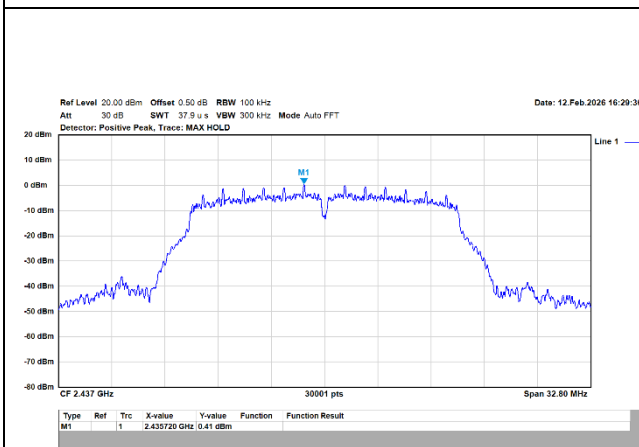
802.11g/20MHz/6M/2437MHz/Ch6/Ant.1 (Ref.)
