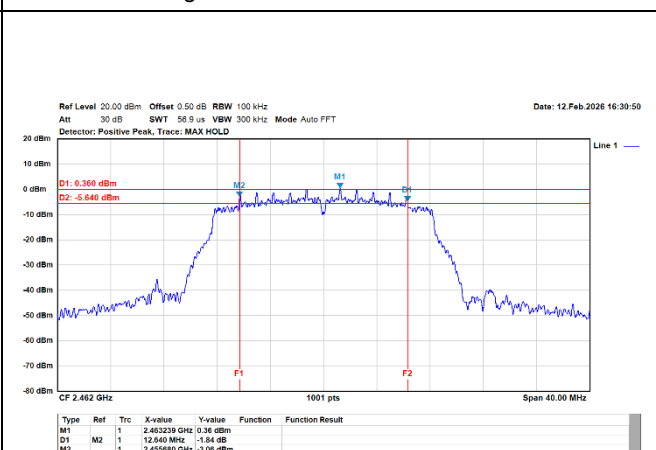
802.11g/20MHz/6M/2462MHz/Ch11/Ant.1
