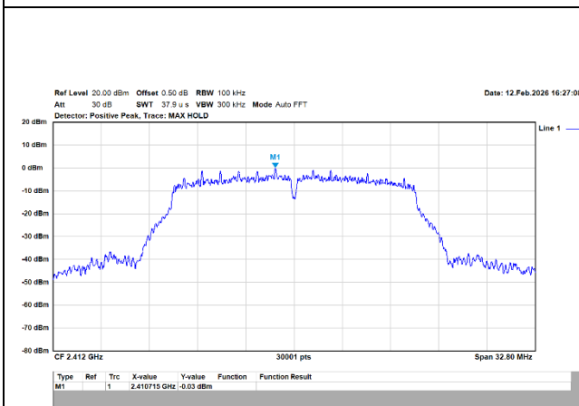
802.11g/20MHz/6M/2412MHz/Ch1/Ant.1 (Ref.)
